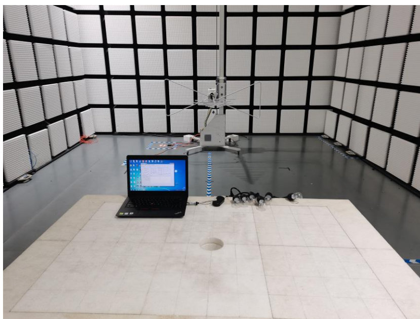
Fig. 2 Radiated emission setup photo(30MHz-1GHz)
