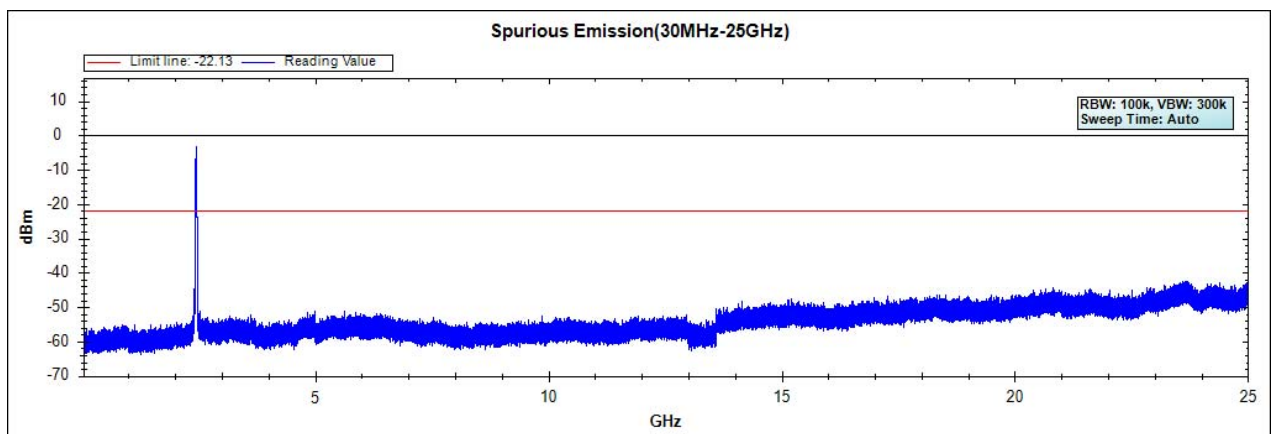
Channel 07 (2452MHz) 30MHz -25GHz-Chain B
