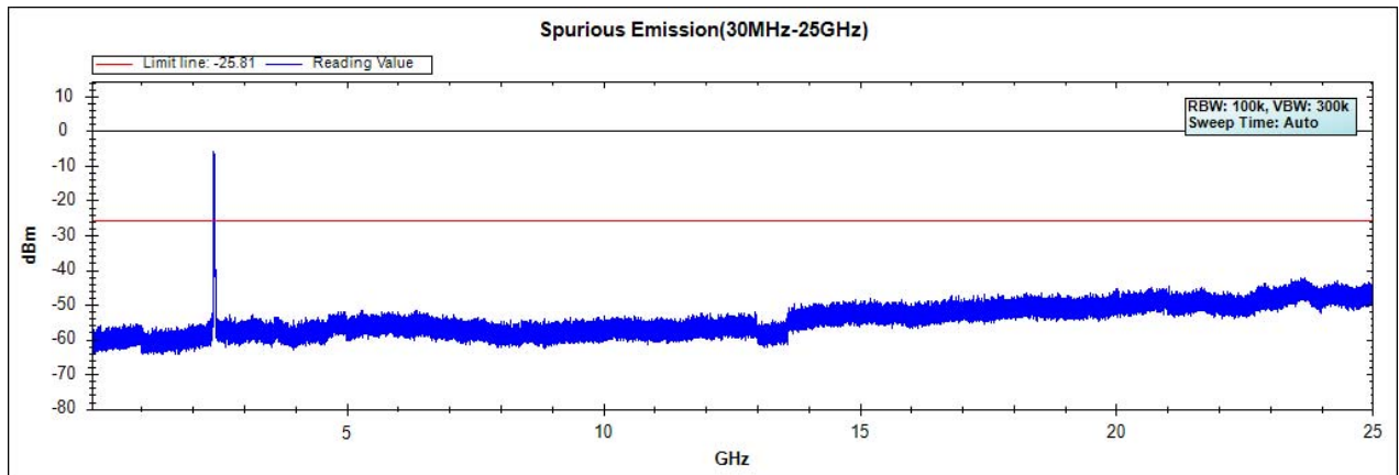
Channel 04 (2437MHz) 30MHz -25GHz-Chain B
