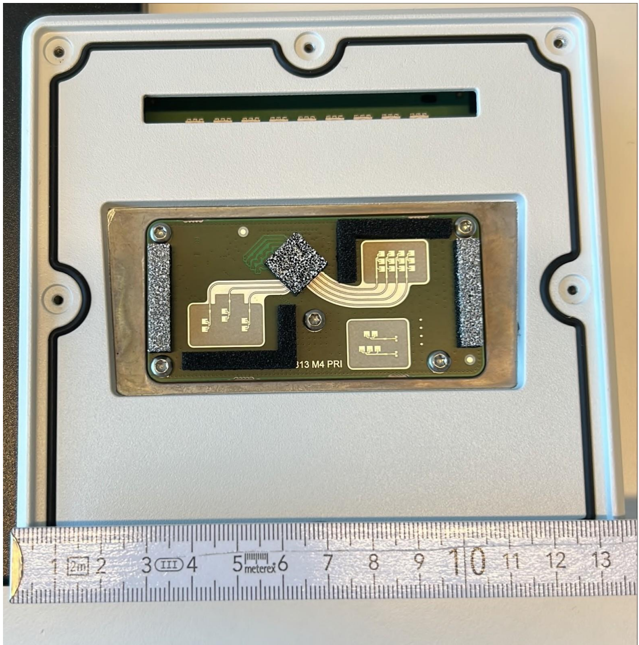
Front view of EUT and RF PCB without radome
