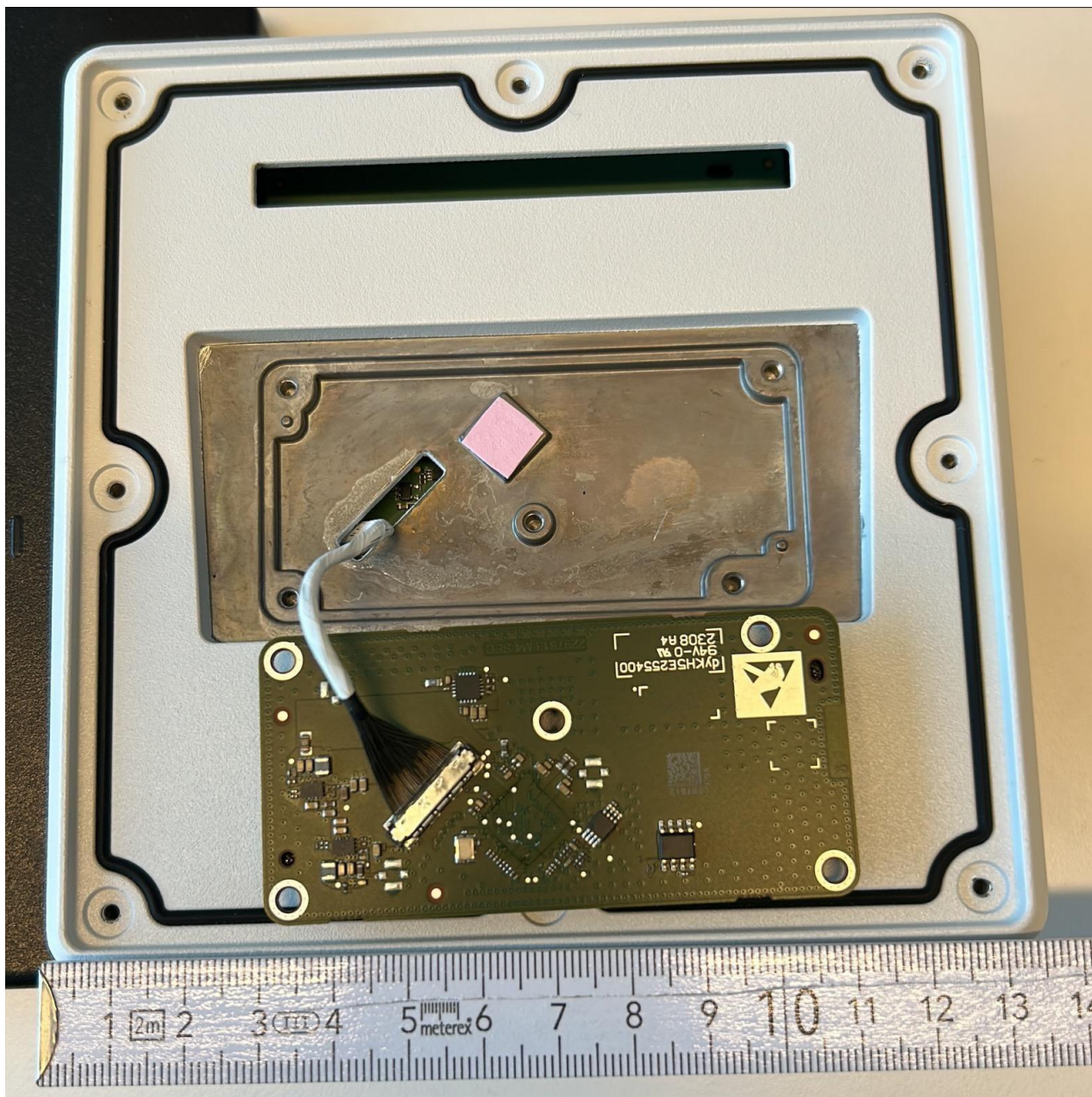
Front view of EUT and back view of RF PCB without radome
