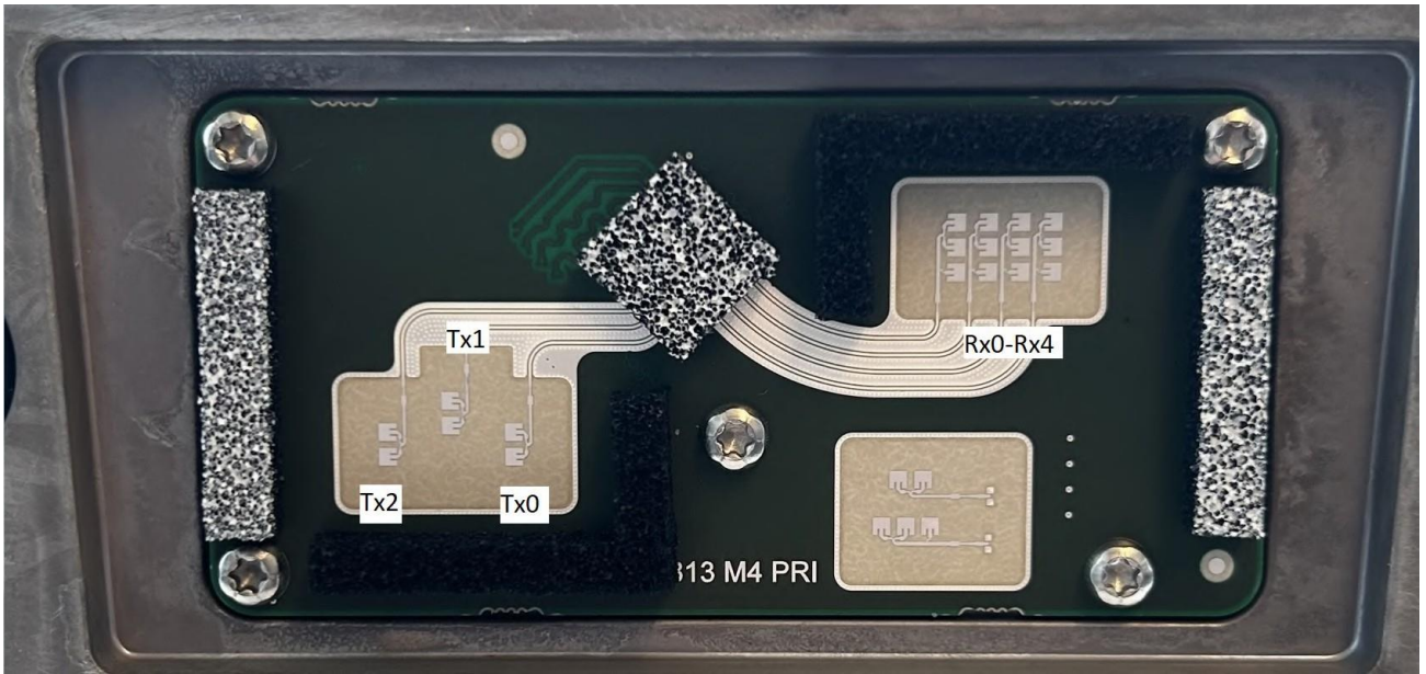
Close-up view of RF PCB with antenna labeling
