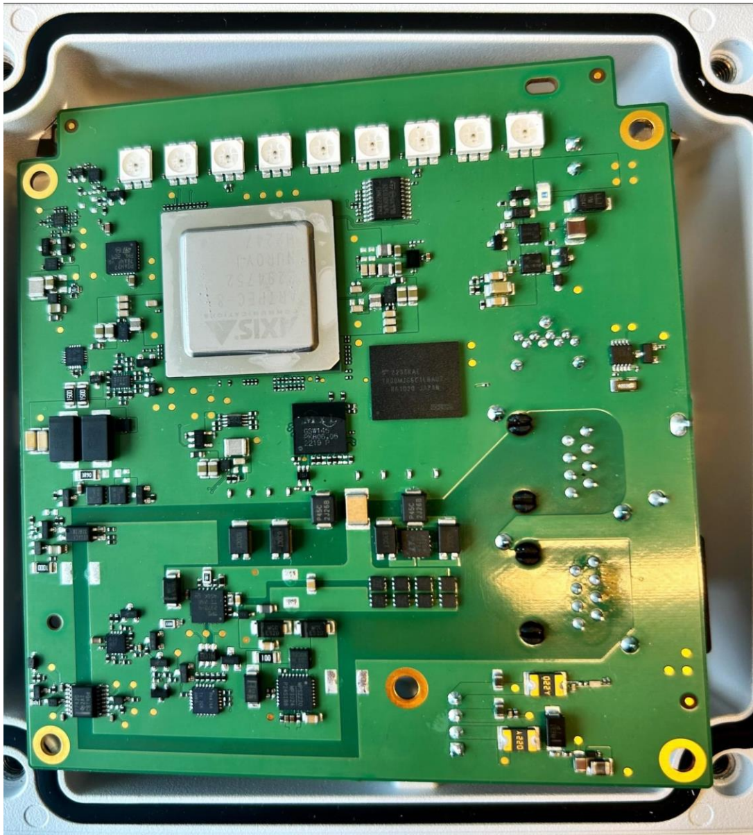
Back view of EUT with gasket and label location
