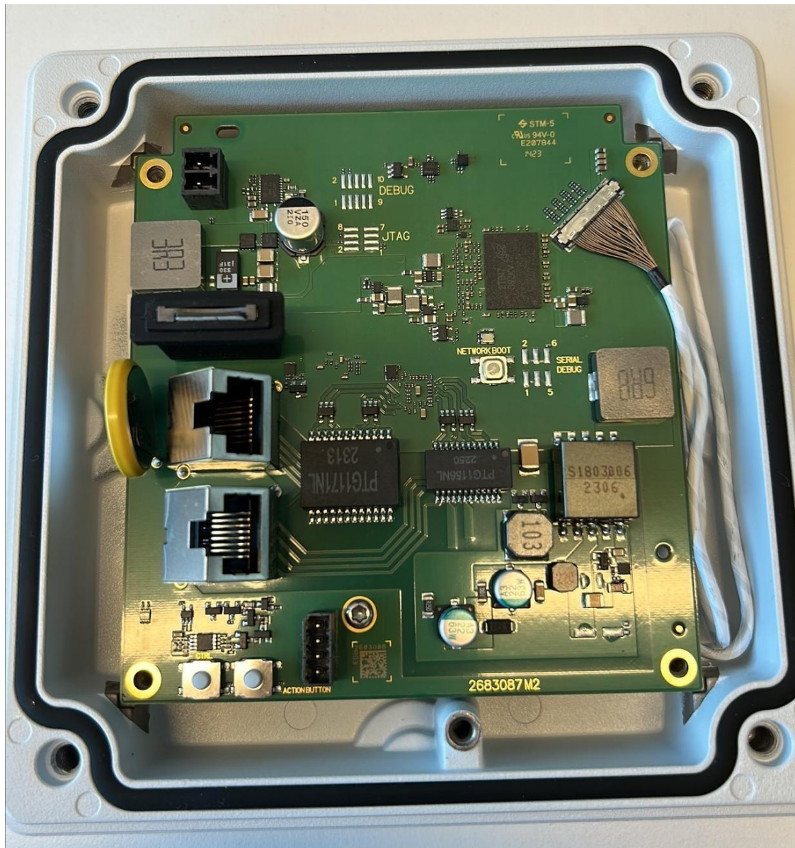
Back view of EUT and main PCB without gasket.
