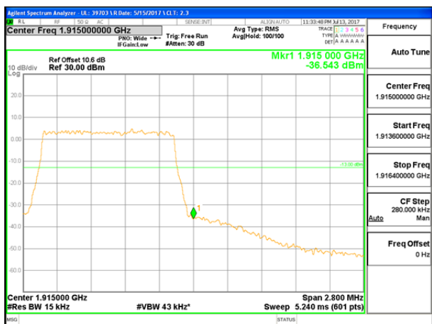
LTE B25 1.4MHz QPSK High Channel FRB
