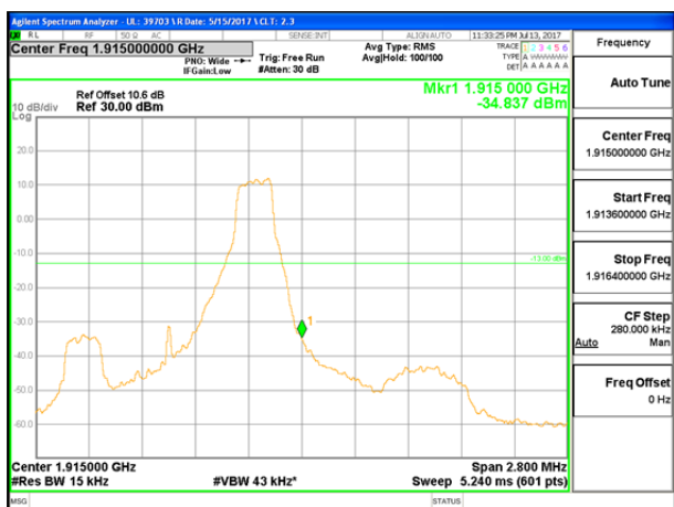
LTE B25 1.4MHz QPSK High Channel 1RB
