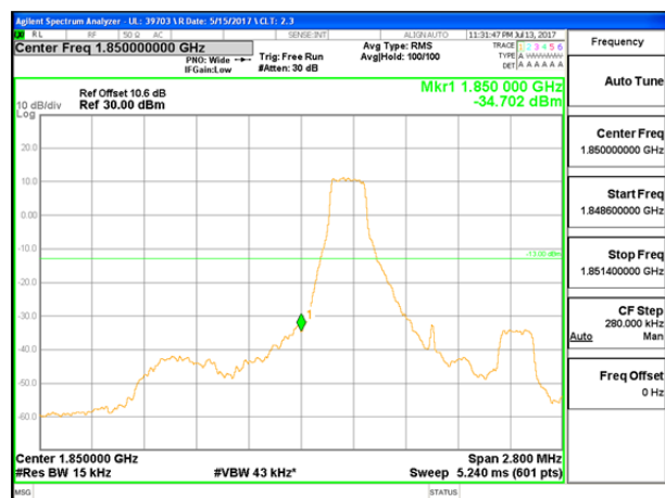
LTE B25 1.4MHz QPSK Low Channel 1RB
