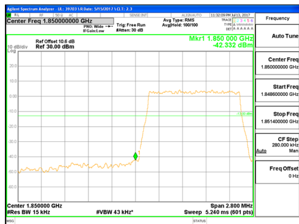
LTE B25 1.4MHz QPSK Low Channel FRB
