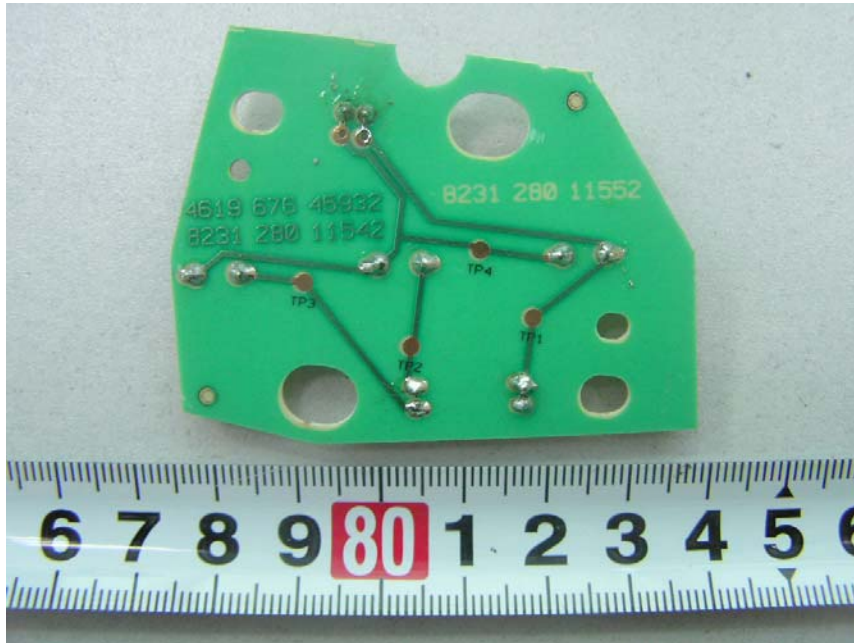
EUT- Fan Control PCB Bottom View
