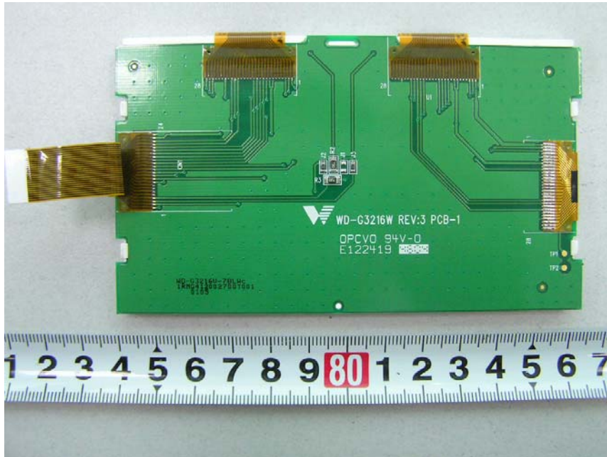
EUT- LCD Bottom View
