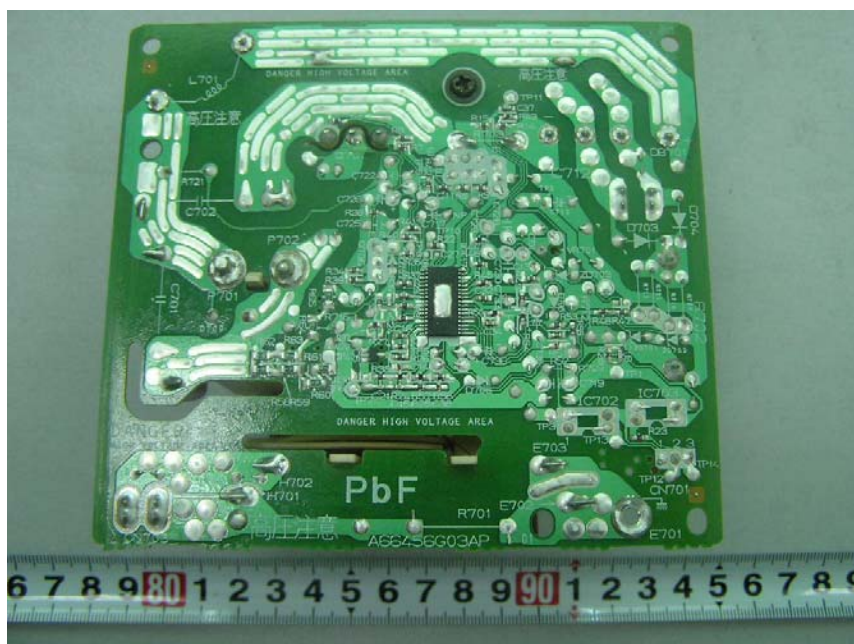
EUT- Transformer PCB Bottom View
