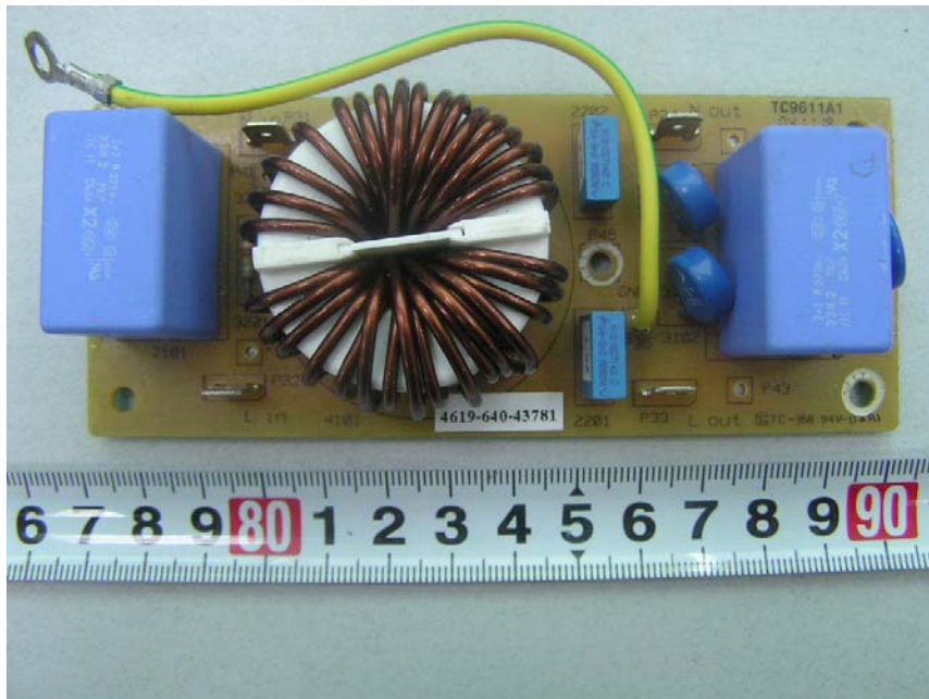
EUT- EMI Filter Top View
