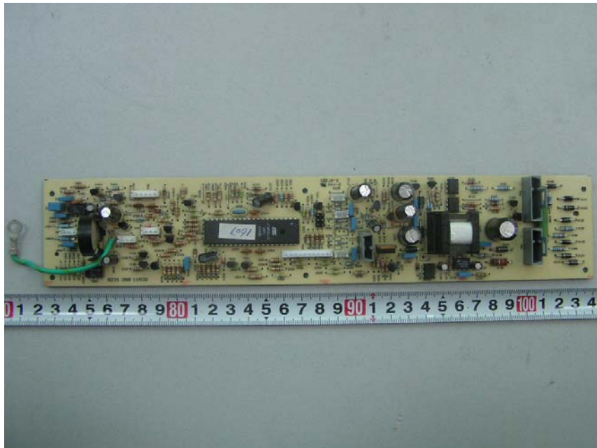
EUT- Power PCB Top View
