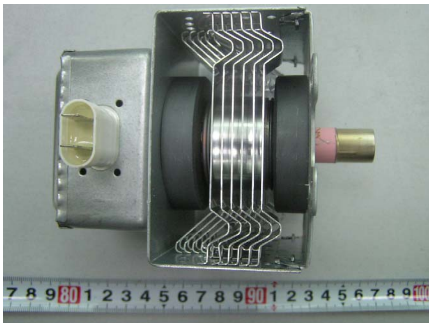
EUT- Magnetron Front View
