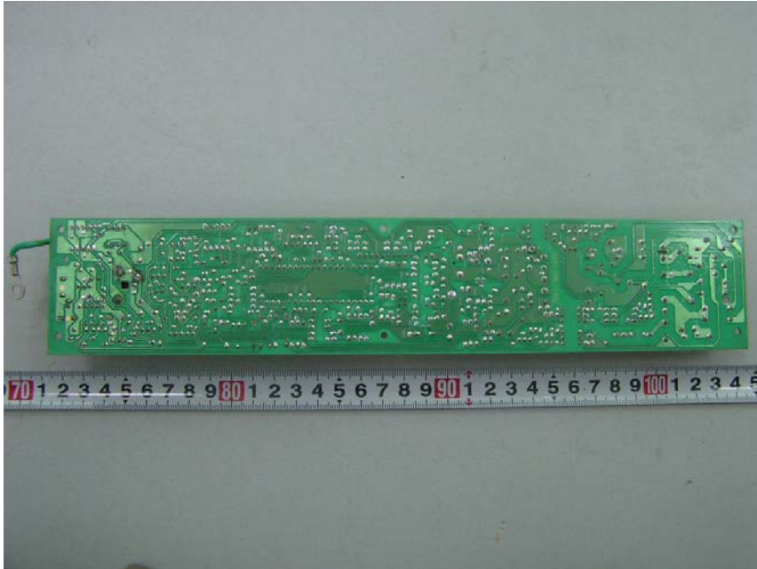
EUT- Power PCB Bottom View
