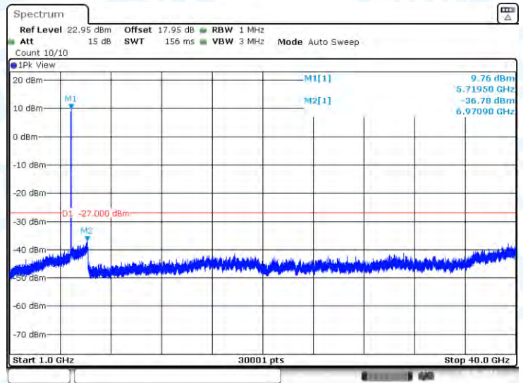
11AC20-CDD-Ant2-5720-1000~40000-PASS
