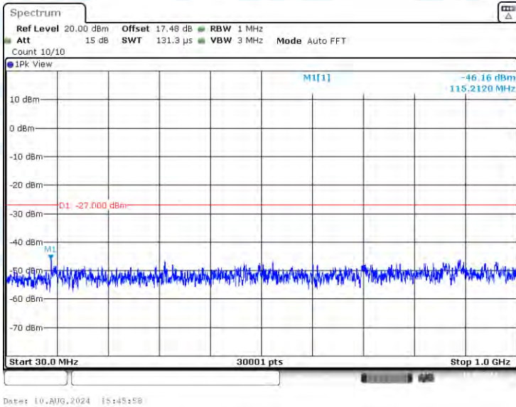
11AC20-CDD-Ant1-5240-30~1000-PASS
