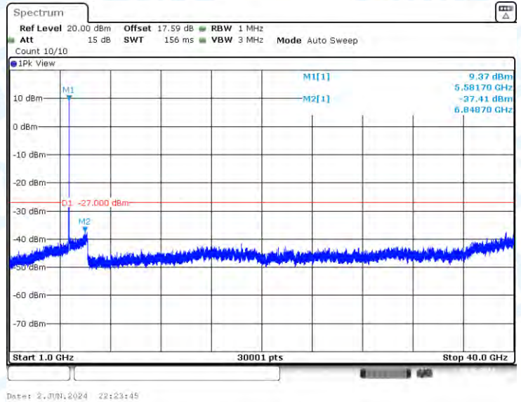
11AC20-CDD-Ant1-5580-1000~40000-PASS
