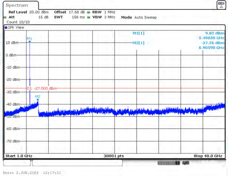
11AC20-CDD-Ant3-5500-1000~40000-PASS
