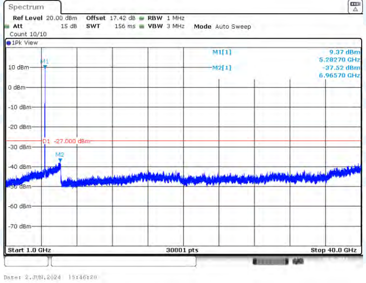
11AC20-CDD-Ant1-5280-1000~40000-PASS
