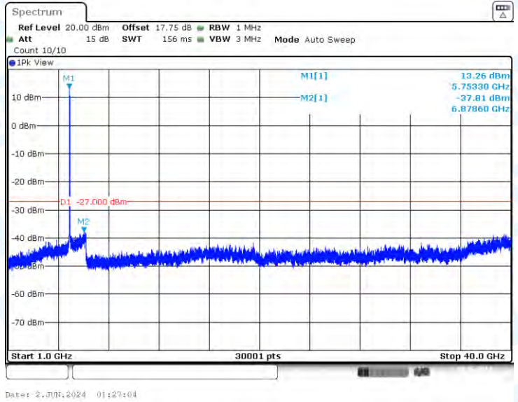
11N40-CDD-Ant2-5755-1000~40000-PASS
