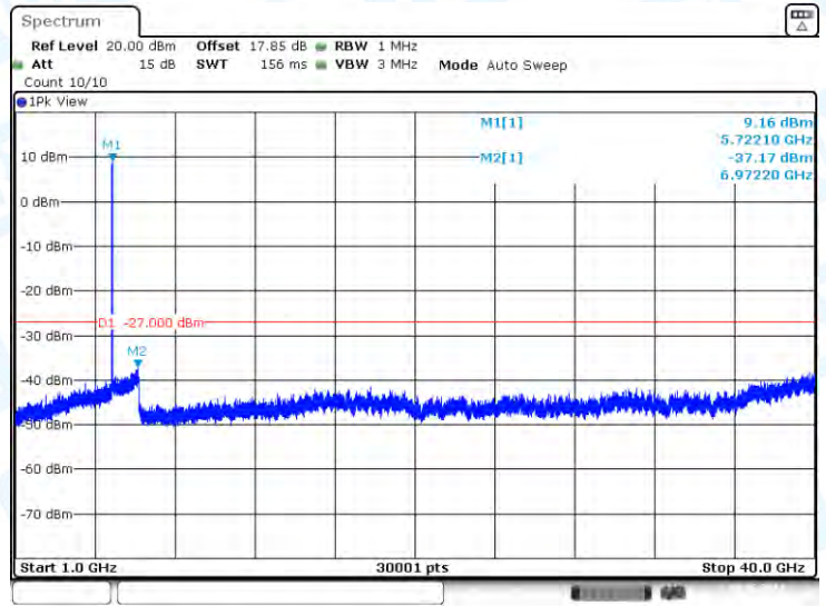
11AC20-CDD-Ant1-5720-1000~40000-PASS
