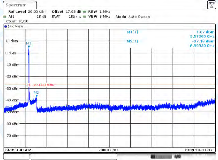
11AC160-CDD-Ant1-5570-1000~40000-PASS
