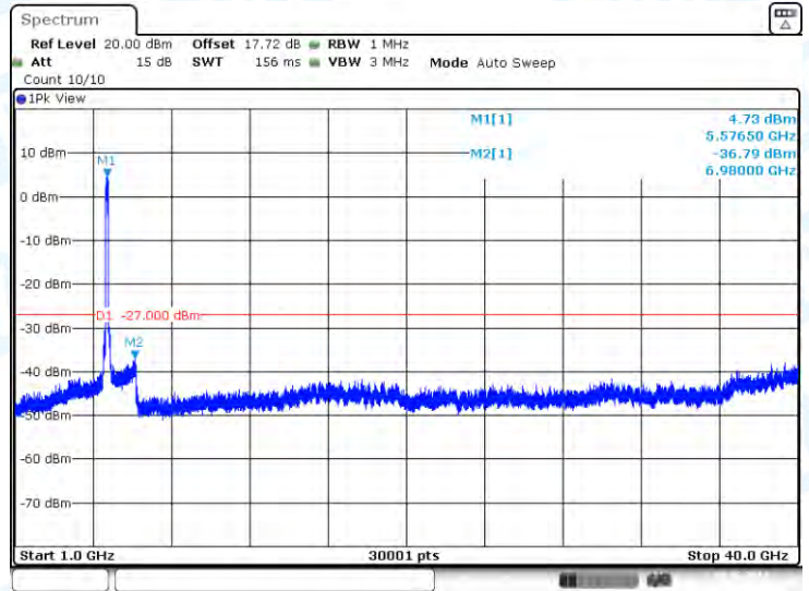
11AC160-CDD-Ant2-5570-1000~40000-PASS
