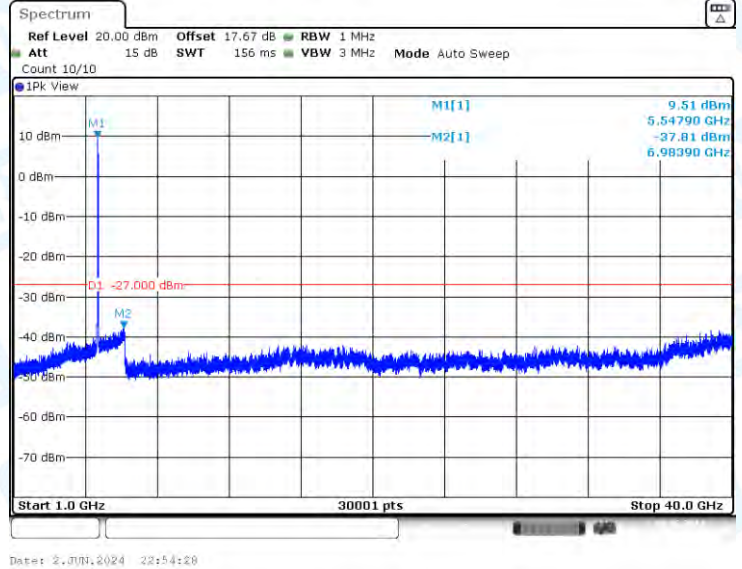
11AC40-CDD-Ant2-5550-1000~40000-PASS
