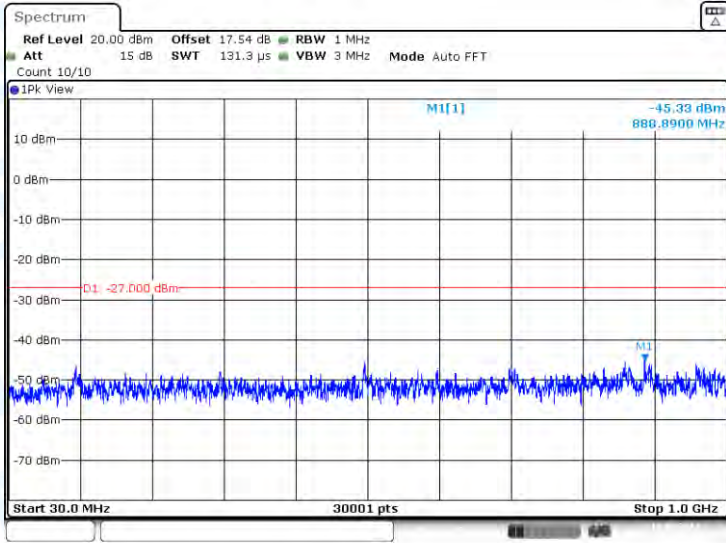
11AC20-CDD-Ant2-5200-30~1000-PASS
