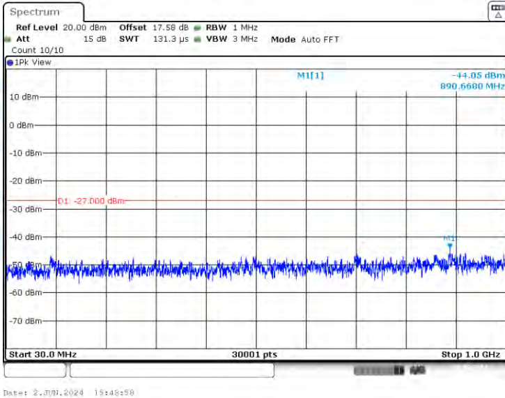
11AC20-CDD-Ant2-5280-30~1000-PASS
