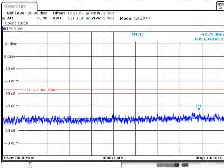
11AC80-CDD-Ant1-5690-30~1000-PASS
