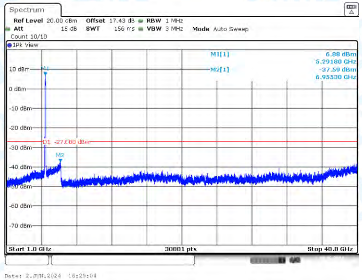
11AC80-CDD-Ant1-5290-1000~40000-PASS
