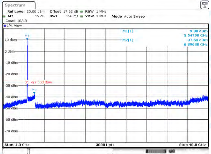
11AC40-CDD-Ant3-5510-1000~40000-PASS
