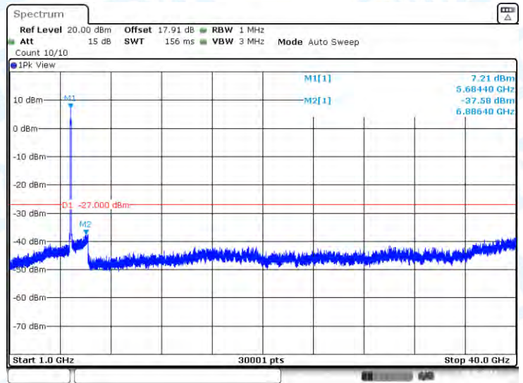
11AC80-CDD-Ant1-5690-1000~40000-PASS
