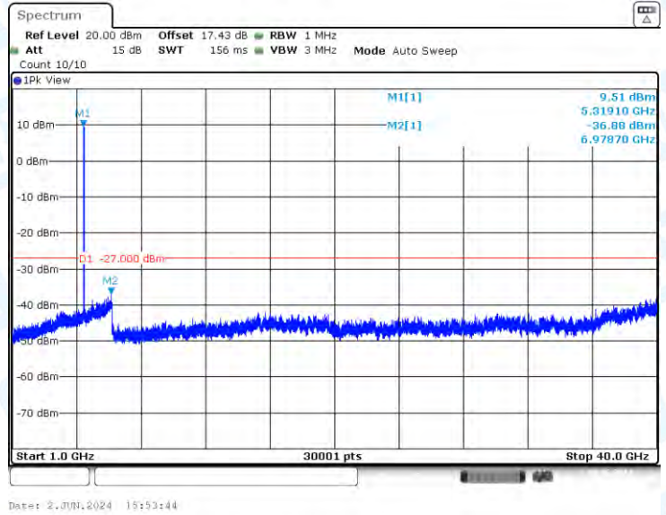
11AC20-CDD-Ant1-5320-1000~40000-PASS
