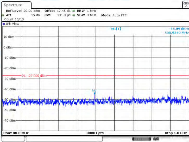
11N40-CDD-Ant3-5795-30~1000-PASS
