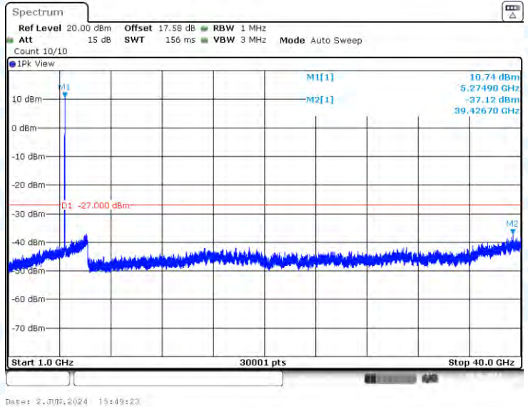
11AC20-CDD-Ant2-5280-1000~40000-PASS
