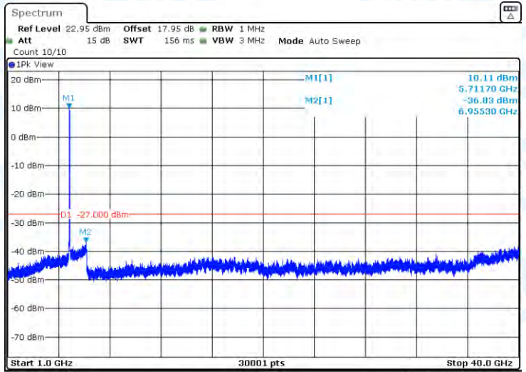
11AC40-CDD-Ant2-5710-1000~40000-PASS
