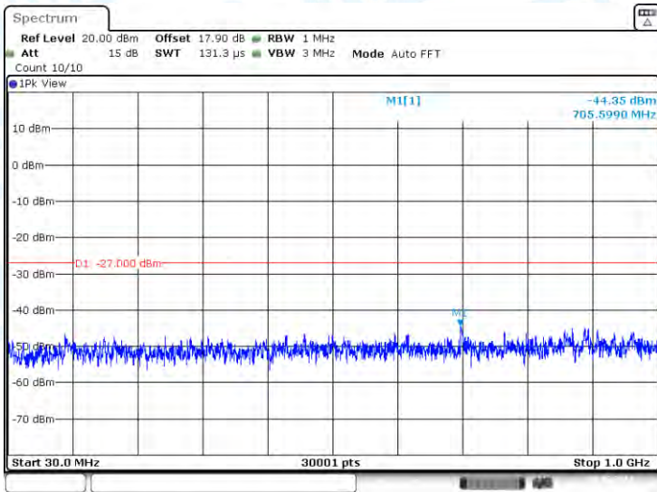
11N40-CDD-Ant3-5550-30~1000-PASS
