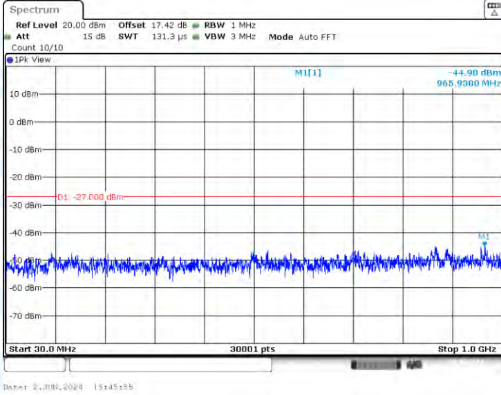
11AC20-CDD-Ant1-5280-30~1000-PASS
