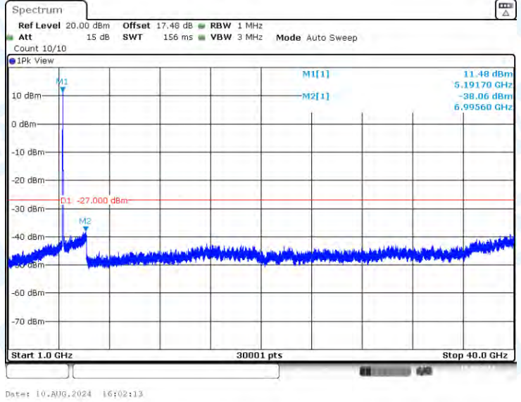
11AC40-CDD-Ant2-5190-1000~40000-PASS
