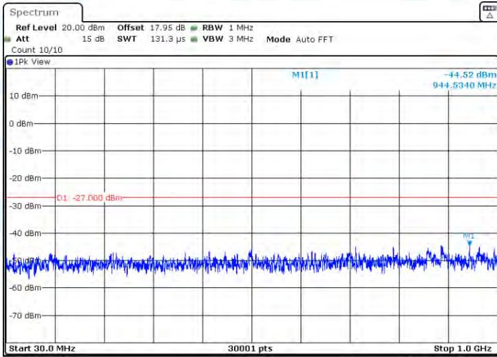
11AC40-CDD-Ant2-5710-30~1000-PASS
