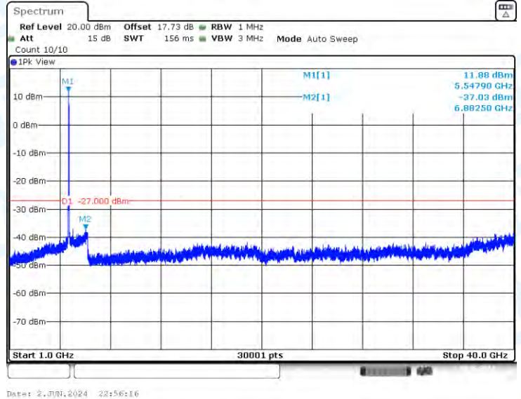
11AC40-CDD-Ant3-5550-1000~40000-PASS
