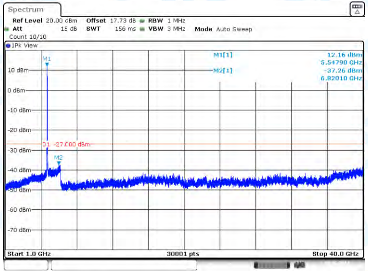
11N40-CDD-Ant2-5550-1000~40000-PASS
