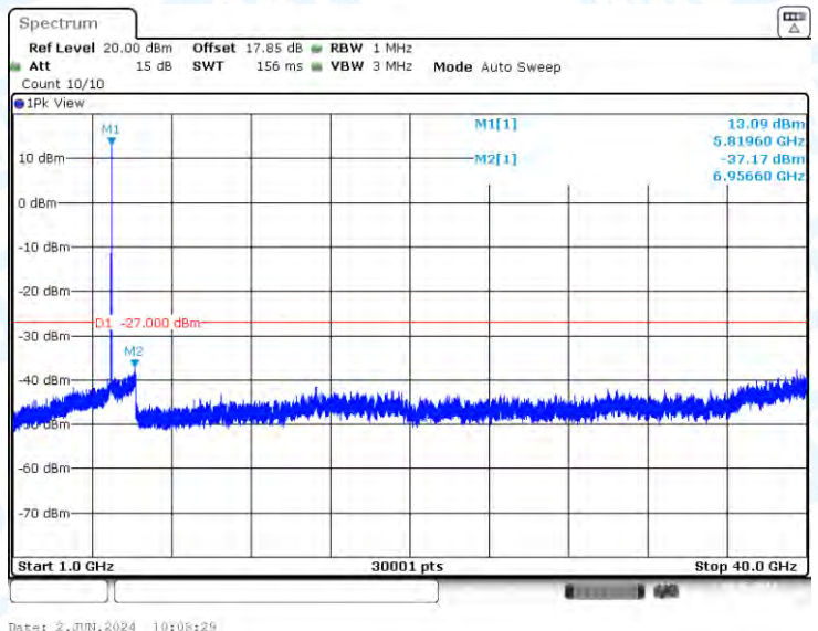
11AC20-CDD-Ant1-5825-1000~40000-PASS
