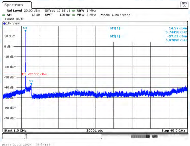
11AC20-CDD-Ant2-5745-1000~40000-PASS
