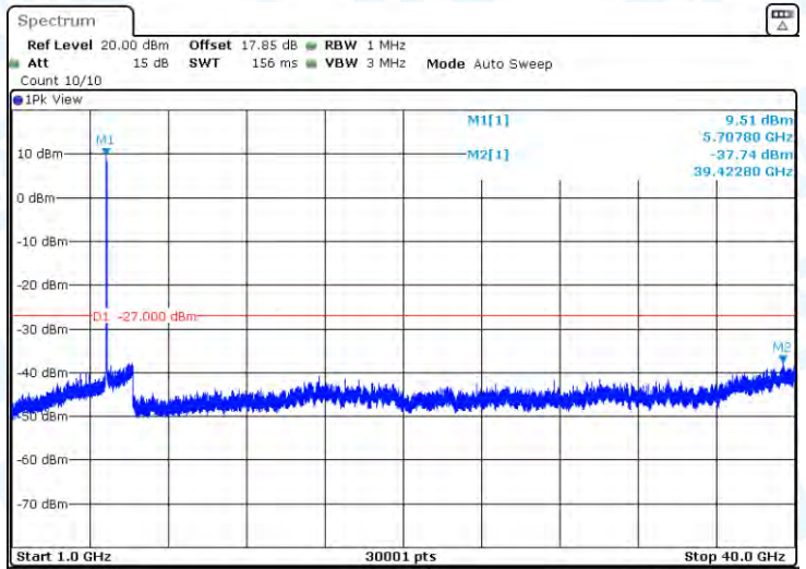
11AC40-CDD-Ant1-5710-1000~40000-PASS
