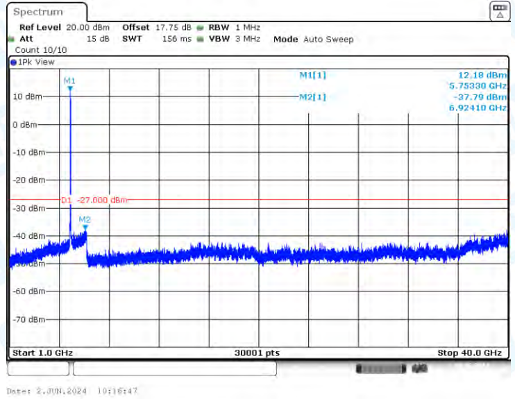
11AC40-CDD-Ant1-5755-1000~40000-PASS
