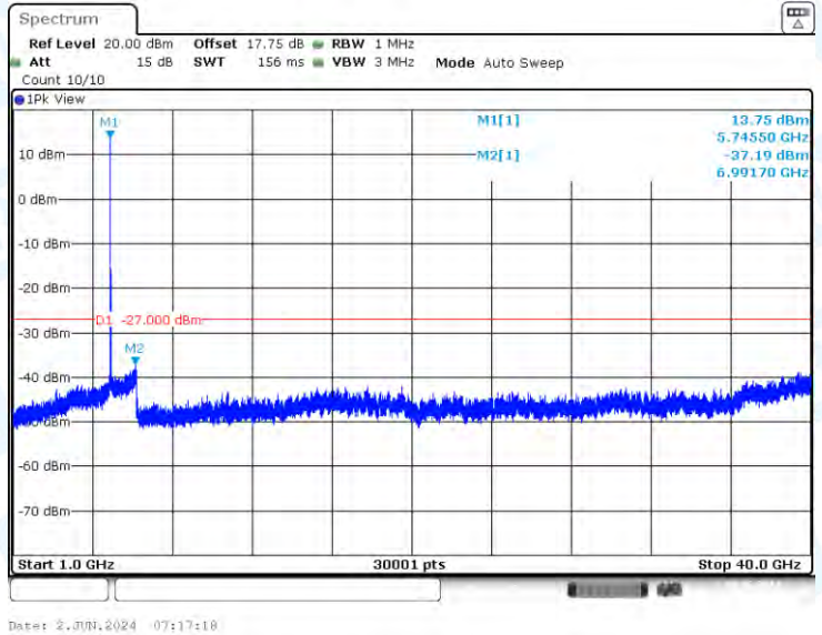
11AC20-CDD-Ant1-5745-1000~40000-PASS
