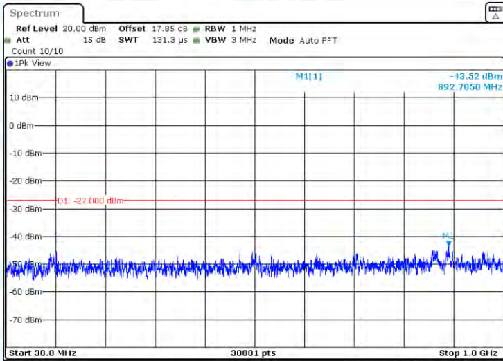
11AC40-CDD-Ant1-5710-30~1000-PASS
