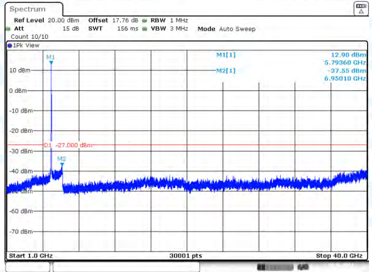
11AC40-CDD-Ant1-5795-1000~40000-PASS
