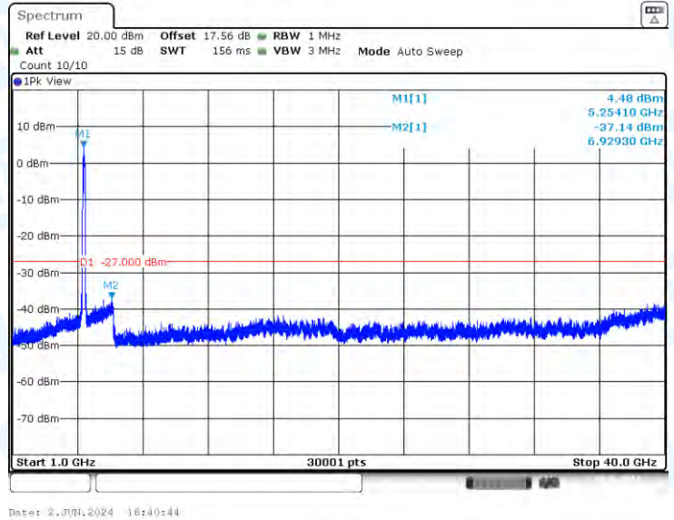
11AC160-CDD-Ant2-5250-1000~40000-PASS
