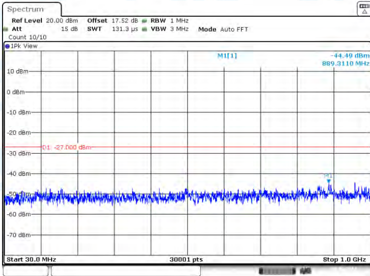
11AC20-CDD-Ant1-5320-30~1000-PASS
