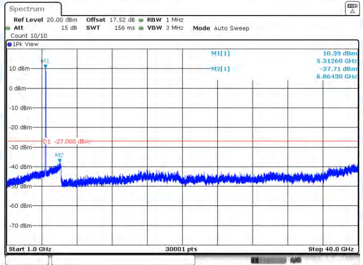
11AC40-CDD-Ant1-5310-1000~40000-PASS
