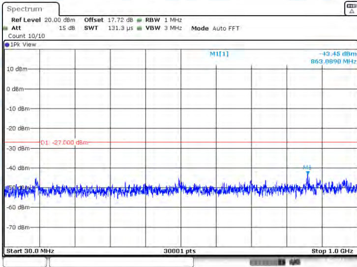
11AC160-CDD-Ant2-5570-30~1000-PASS
