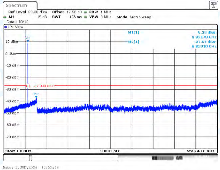
11AC20-CDD-Ant2-5320-1000~40000-PASS
