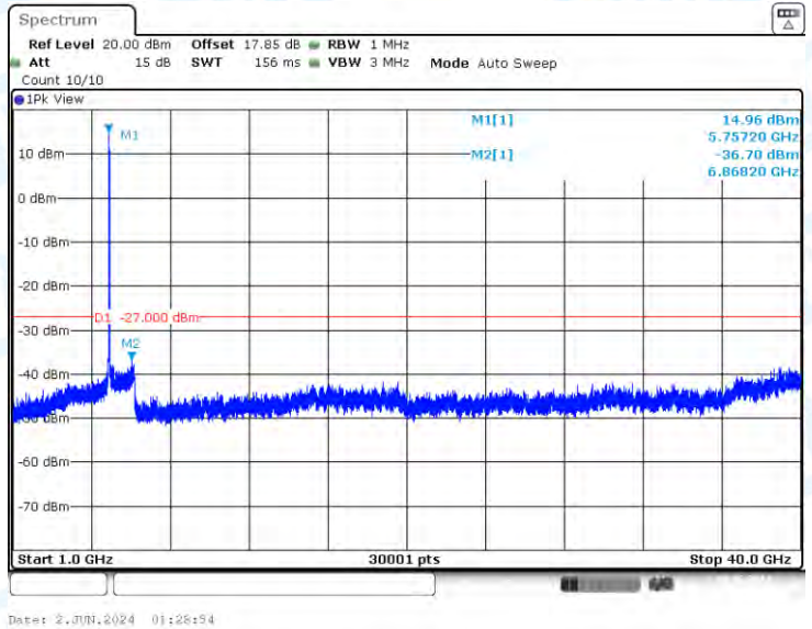
11N40-CDD-Ant3-5755-1000~40000-PASS
