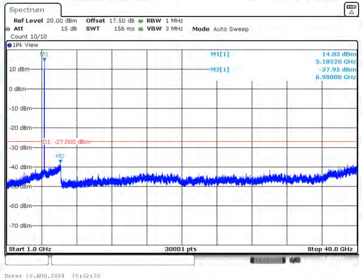
11AC20-CDD-Ant2-5180-1000~40000-PASS
