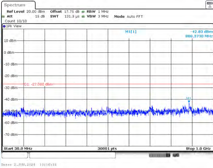
11AC40-CDD-Ant1-5755-30~1000-PASS
