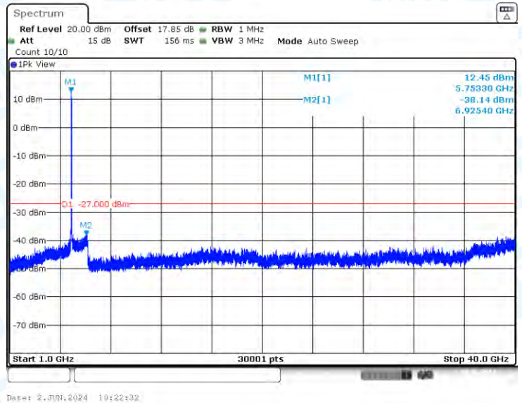
11AC40-CDD-Ant2-5755-1000~40000-PASS
