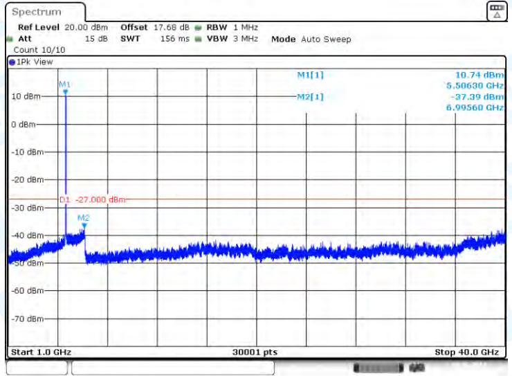
11AC40-CDD-Ant2-5510-1000~40000-PASS
