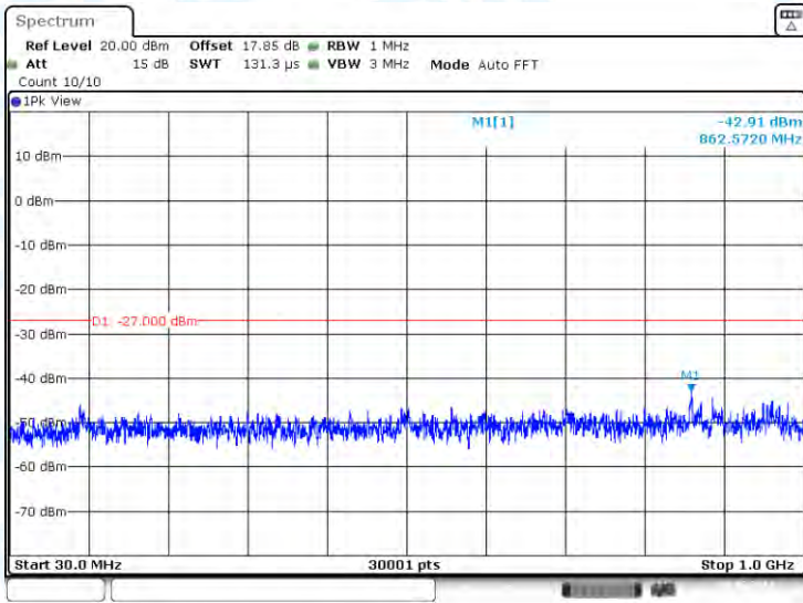
11AC20-CDD-Ant1-5720-30~1000-PASS
