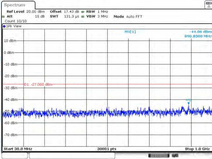
11AC20-CDD-Ant3-5280-30~1000-PASS
