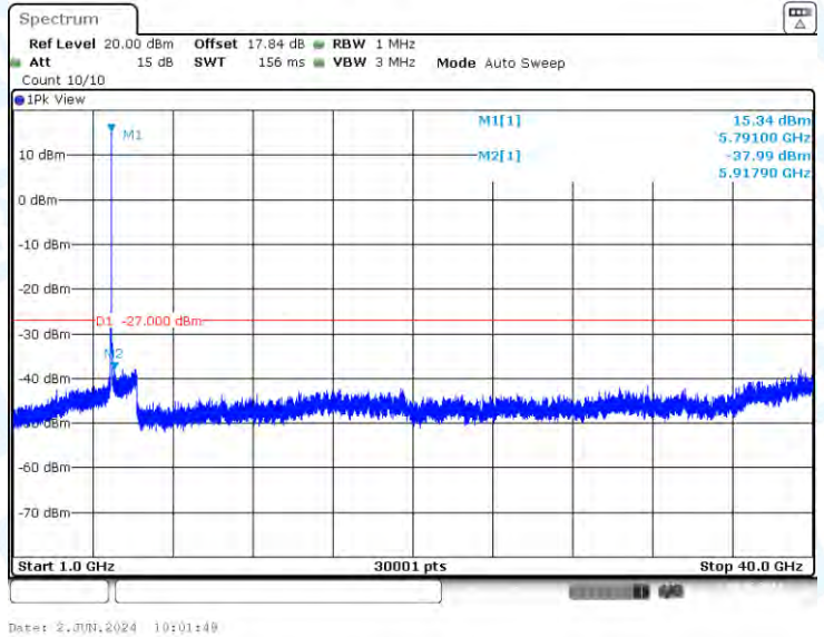
11AC20-CDD-Ant3-5785-1000~40000-PASS
