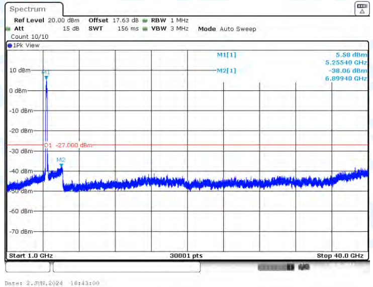
11AC160-CDD-Ant3-5250-1000~40000-PASS
