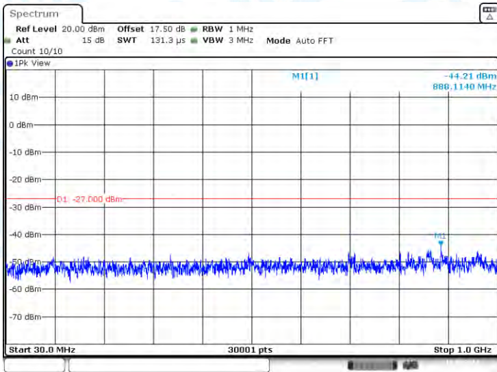
11AC20-CDD-Ant1-5180-30~1000-PASS
