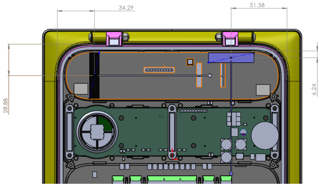
Wi-Fi Antenna Placement
