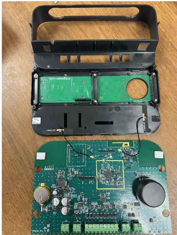
Inside PCB antenna connections
