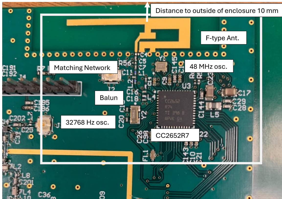
Bluetooth RF section of circuit board
