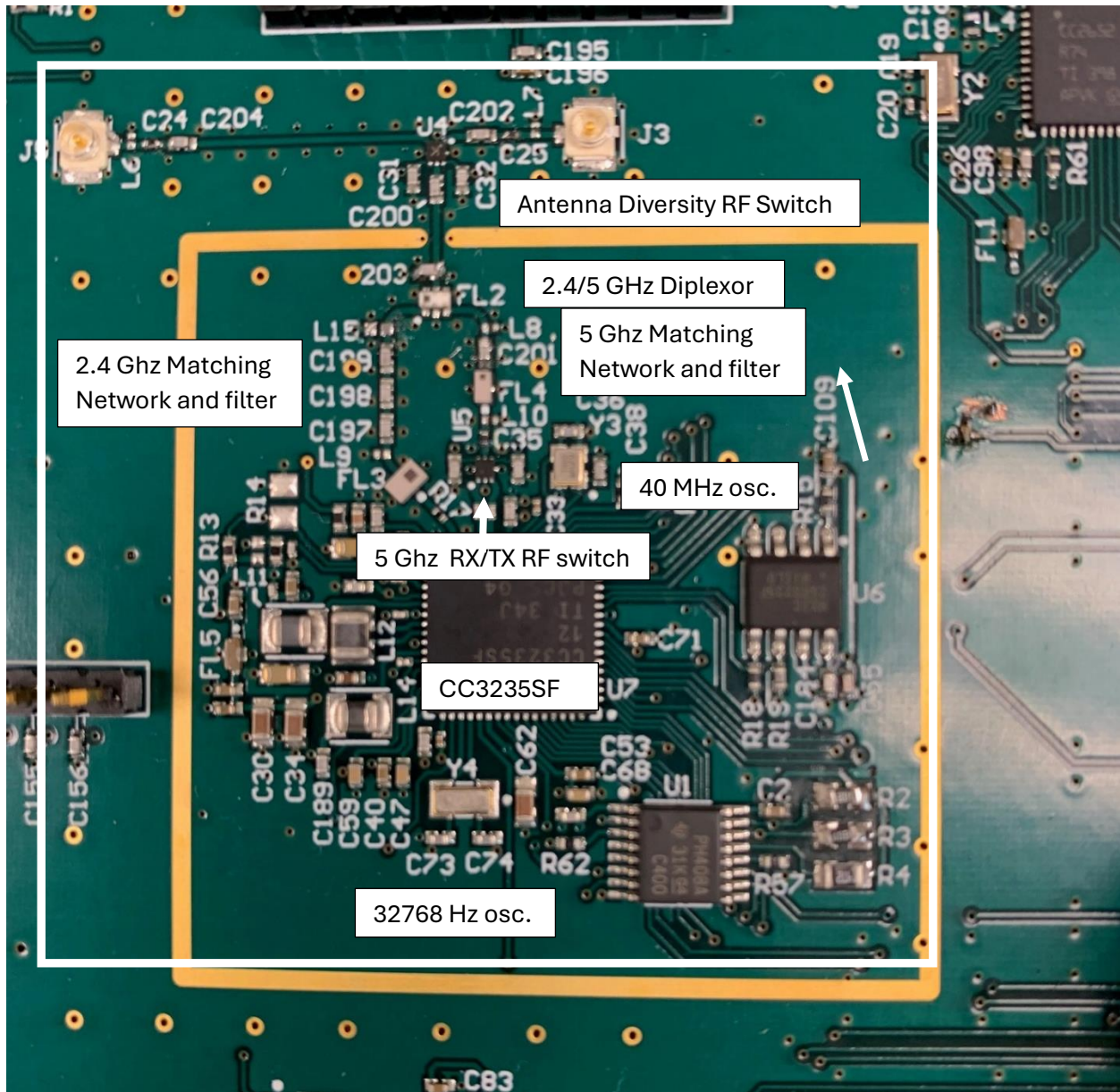
Wi-Fi RF section of circuit board
