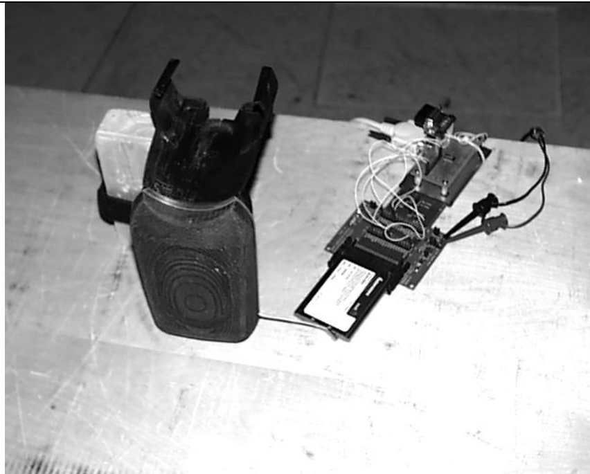
EUT Close Up Shows 915 PC Card-6 operated outside of IP3
