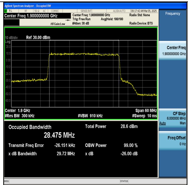
NTNV-n25-PC3-15-30-H-CP-256QAM-Outer_Full-Ant1- PASS
