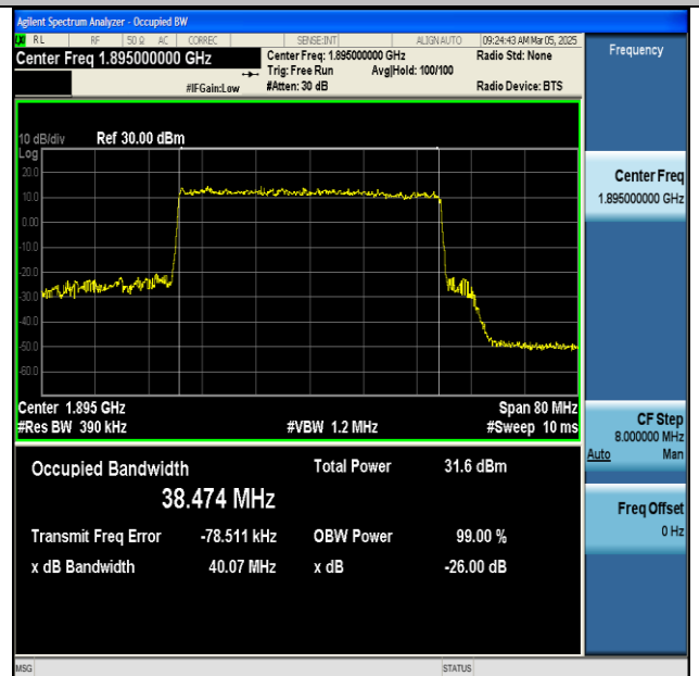
NTNV-n25-PC3-15-40-H-CP-64QAM-Outer_Full-Ant1-PASS
