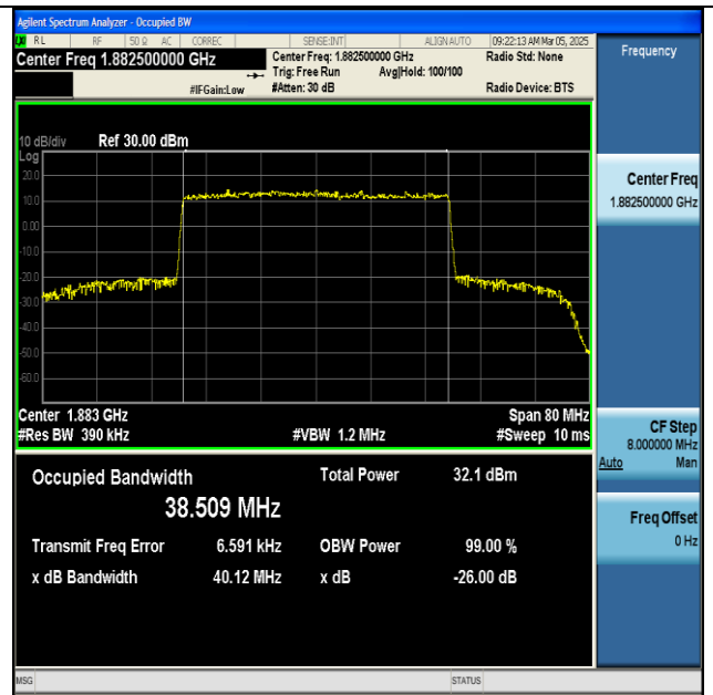
NTNV-n25-PC3-15-40-M-CP-16QAM-Outet_Full-Ant1-PASS
