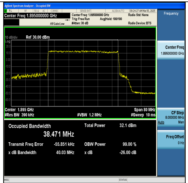
NTNV-n25-PC3-15-40-H-CP-QPSK-Outer_Full-Ant1-PASS
