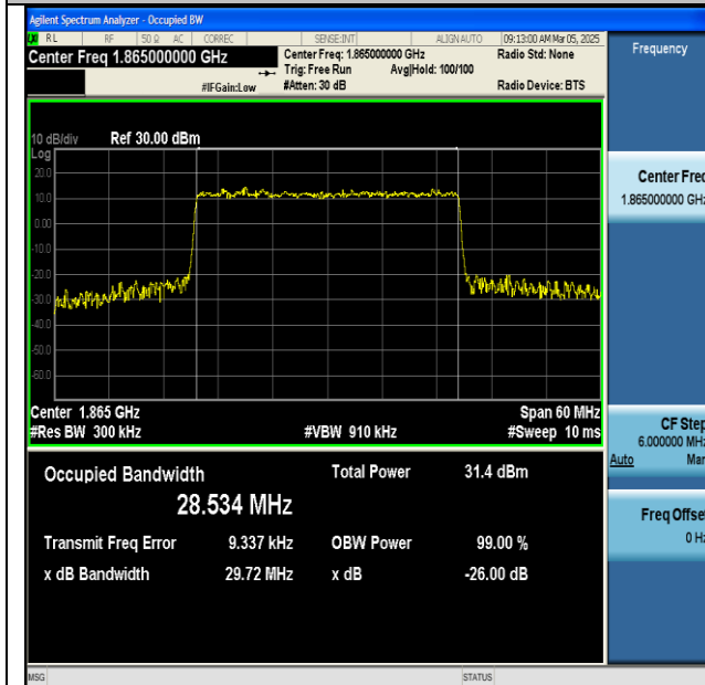
NTNV-n25-PC3-15-30-L-CP-64QAM-Outer_Full-Ant1-PASS
