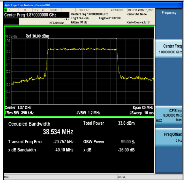
NTNV-n25-PC3-15-40-L-DFT-QPSK-Outer_Full-Ant1- PASS
