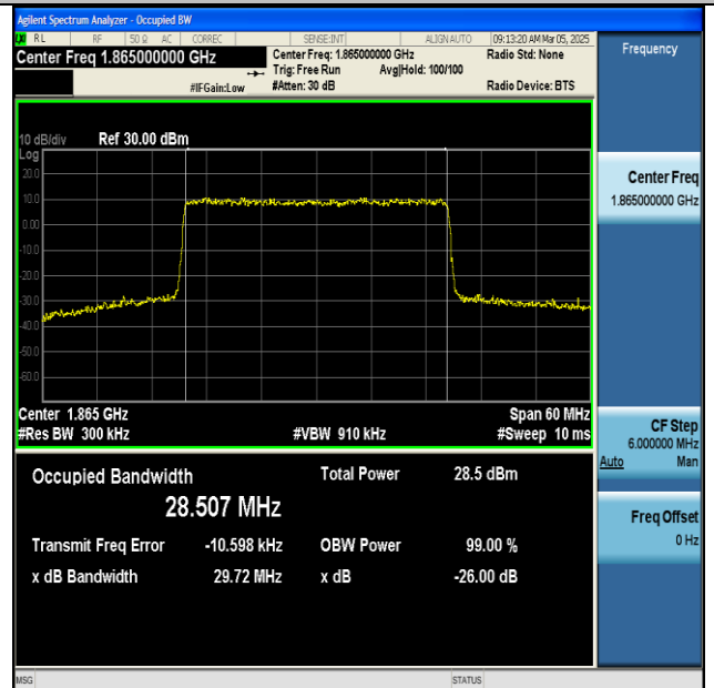
NTNV-n25-PC3-15-30-L-CP-256QAM-Outer_Full-Ant1-PASS
