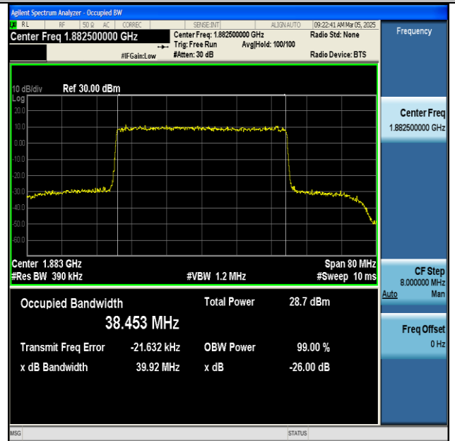
NTNV-n25-PC3-15-40-M-CP-256QAM-Outet_Full-Ant1-PASS
