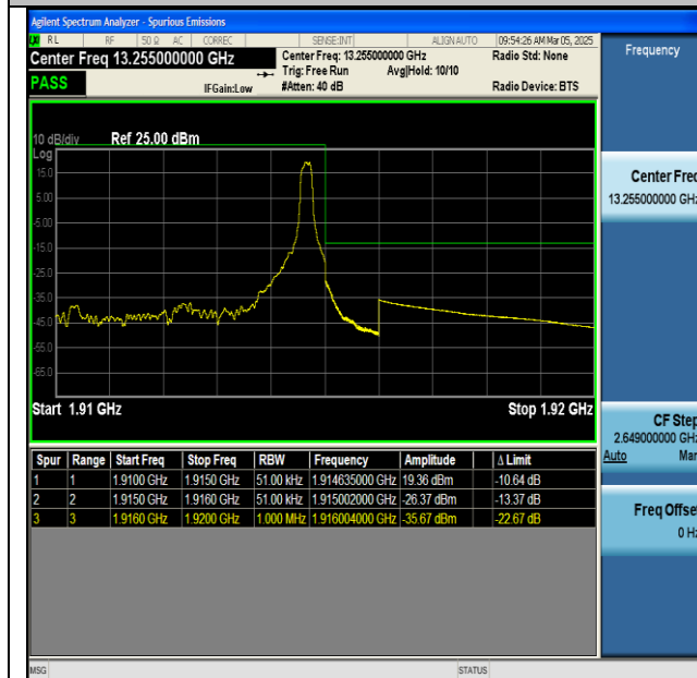
NTNV-n25-PC3-15-5-H-CP-QPSK-Edge_1RB_Right-PASS
