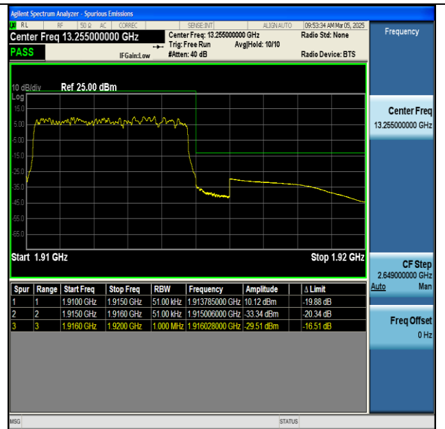
NTNV-n25-PC3-15-5-H-DFT-BPSK-Outer_Full-PASS
