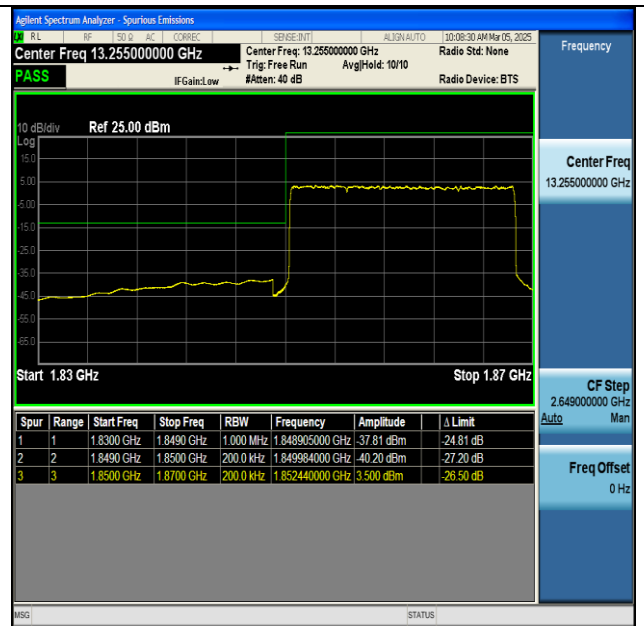
NTNV-n25-PC3-15-20-L-DFT-BPSK-Outer_Full-PASS
