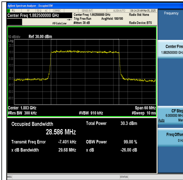
NTNV-n25-PC3-15-30-M-DFT-256QAM-Outer_Full-Ant1-PASS
