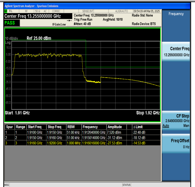
NTNV-n25-PC3-15-5-H-CP-QPSK-Outer_Full-PASS
