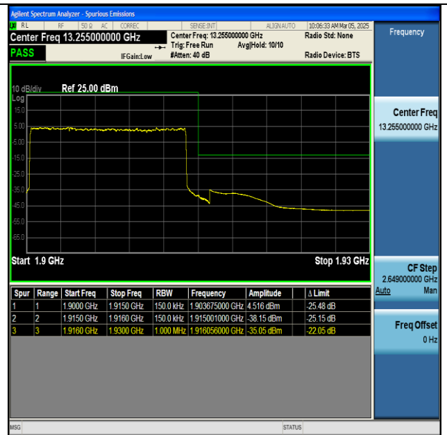
NTNV-n25-PC3-15-15-H-DFT-BPSK-Outer_Full-PASS
