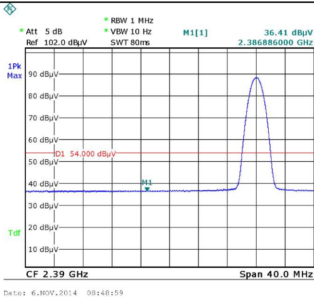
8DPSK-Left Side-Ave
