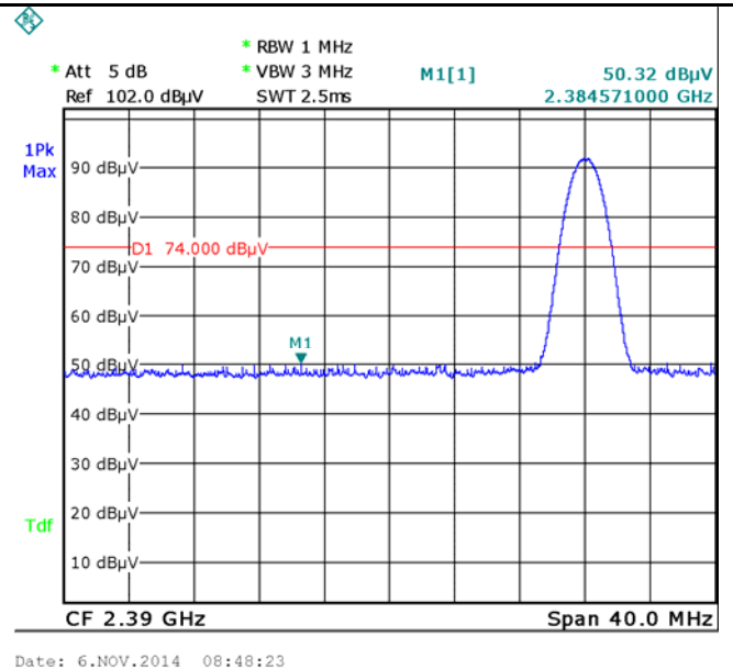
8DPSK-Left Side-PK
