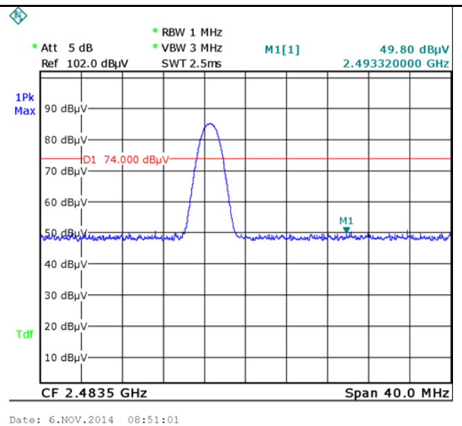
8DPSK-Right Side-PK
