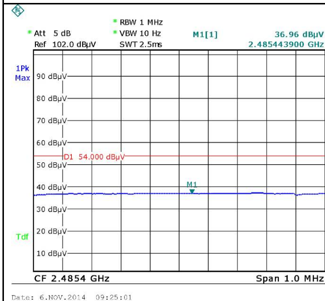
8DPSK-Hopping-PK
