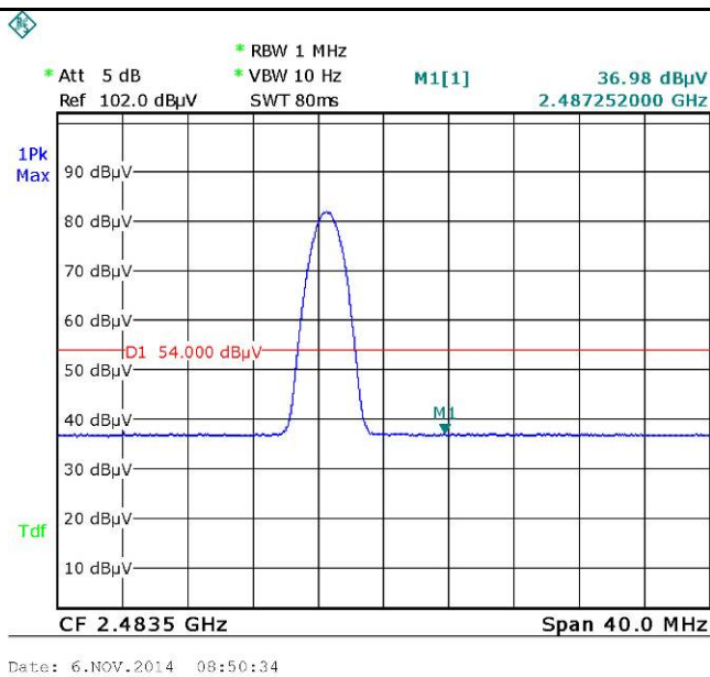
8DPSK-Right Side-Ave
