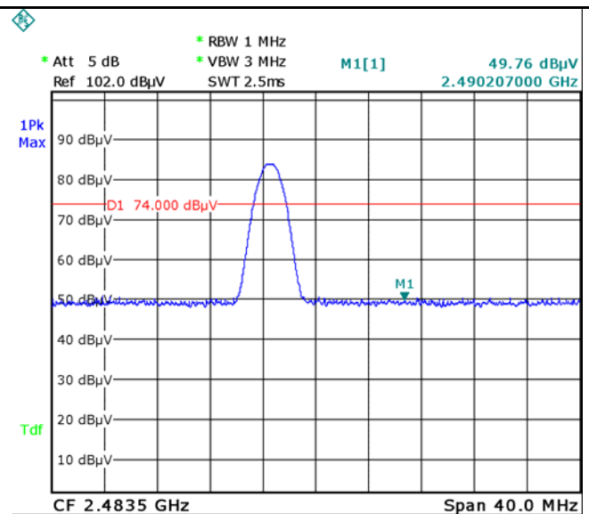
\pi/4 DQPSK-Left Side-PK
