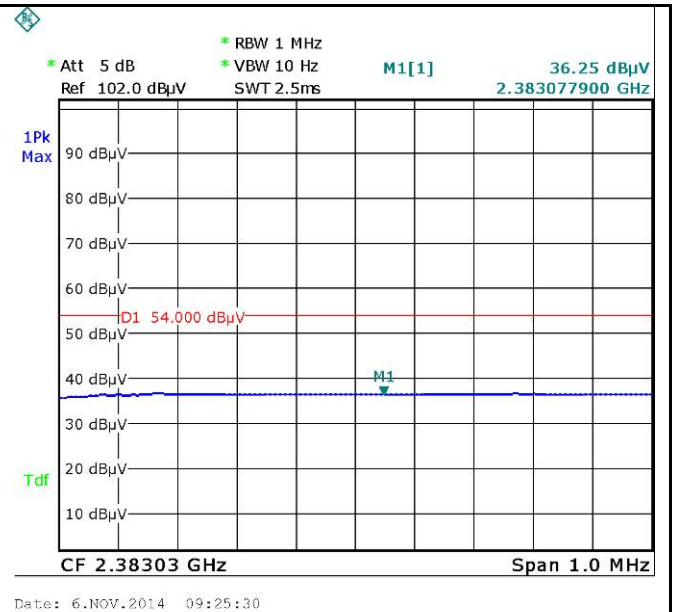
8DPSK-Hopping-Ave-Left Side
