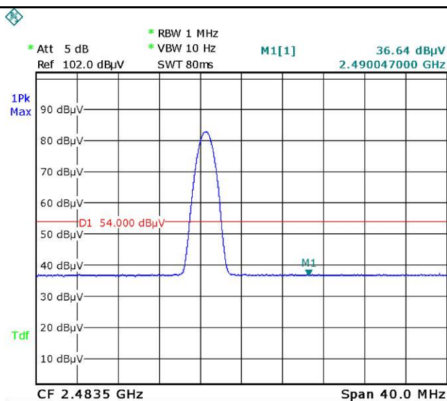
GFSK-Left Side-Ave
