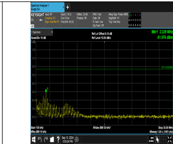
Band17_10MHz_QPSK_23790_1RB#0_0.15~30_0.15~30
