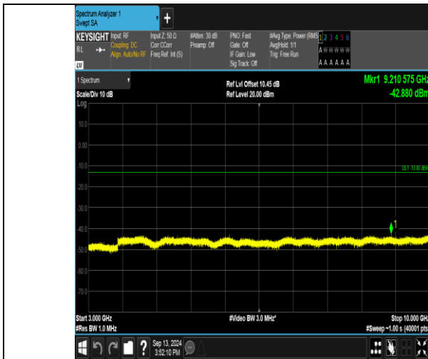
Band17_10MHz_QPSK_23780_50RB#0_3000~10000_3000~10000
