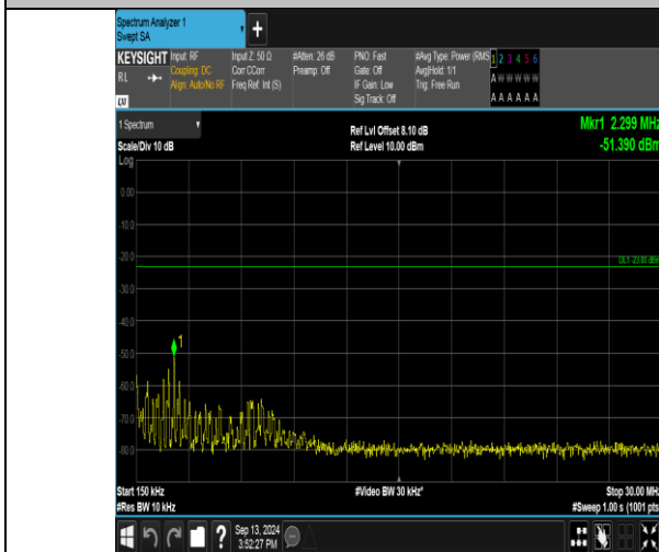
Band17_10MHz_16QAM_23780_50RB#0_0.15~30_0.15~30
