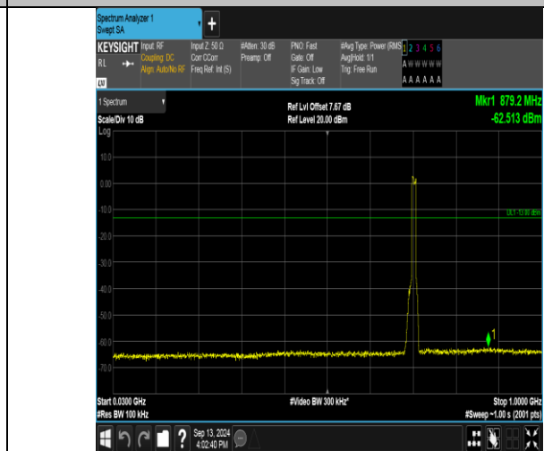
Band17_10MHz_16QAM_23800_50RB#0_30~1000_30~1000
