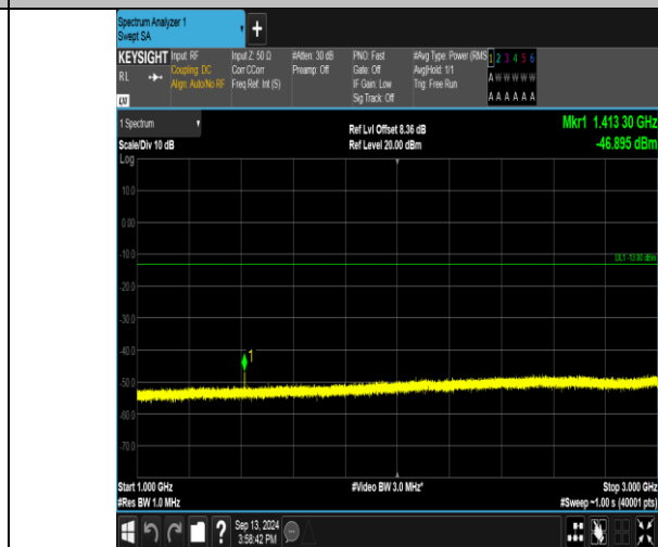
Band17_10MHz_QPSK_23800_1RB#0_1000~3000_1000~3000
