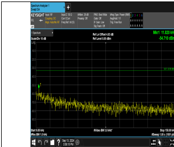
Band17_10MHz_QPSK_23800_1RB#0_0.009~0.15_0.009~0.15
