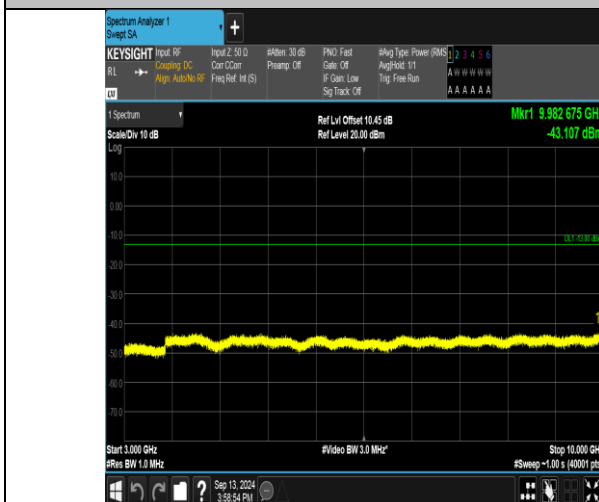
Band17_10MHz_QPSK_23800_1RB#0_3000~10000_3000~10000
