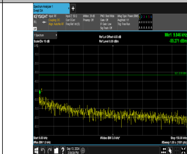
Band17_10MHz_16QAM_23790_1RB#0_0.009~0.15_0.009~0.15
