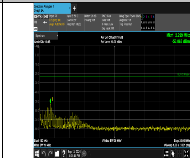
Band17_10MHz_QPSK_23800_50RB#0_0.15~30_0.15~30
