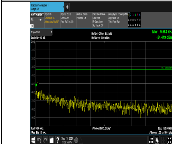
Band17_10MHz_QPSK_23800_1RB#49_0.009~0.15_0.009~0.15
