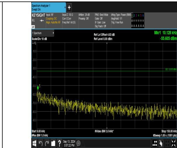
Band17_10MHz_16QAM_23790_50RB#0_0.009~0.15_0.009~0.15
