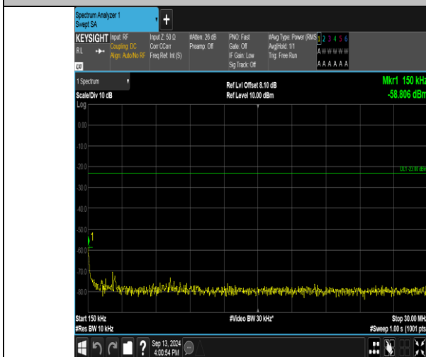
Band17_10MHz_16QAM_23800_1RB#49_0.15~30_0.15~30
