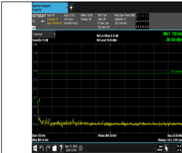
Band17_10MHz_16QAM_23790_1RB#0_0.15~30_0.15~30
