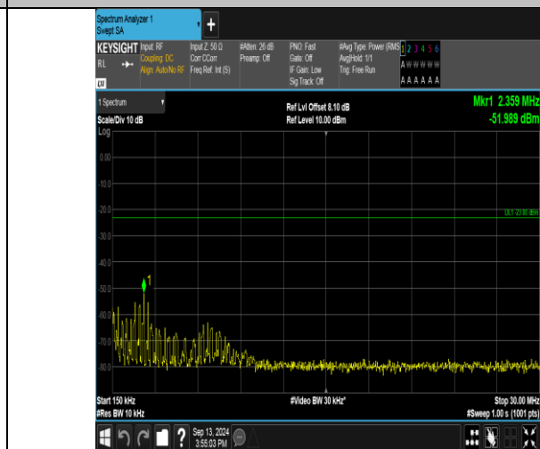
Band17_10MHz_QPSK_23790_1RB#49_0.15~30_0.15~30
