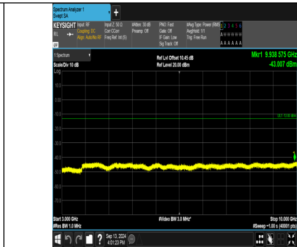
Band17_10MHz_16QAM_23800_1RB#49_3000~10000_3000~10000
