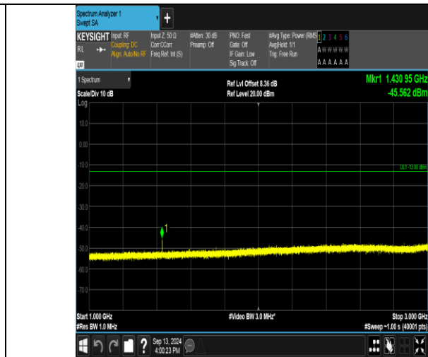
Band17_10MHz_QPSK_23800_1RB#49_1000~3000_1000~3000
