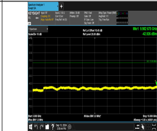
Band17_10MHz_16QAM_23800_1RB#0_3000~10000_3000~10000
