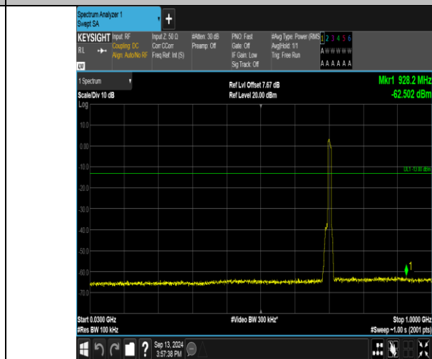
Band17_10MHz_16QAM_23790_50RB#0_30~1000_30~1000
