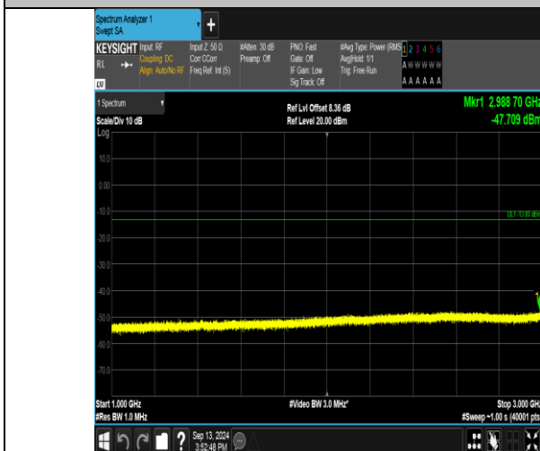
Band17_10MHz_16QAM_23780_50RB#0_1000~3000_1000~3000
