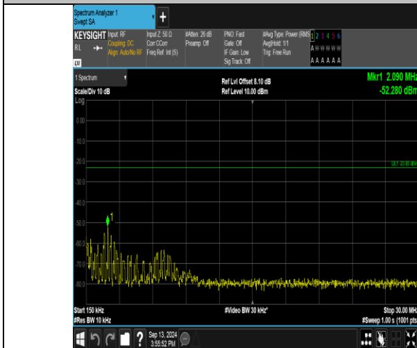
Band17_10MHz_16QAM_23790_1RB#49_0.15~30_0.15~30
