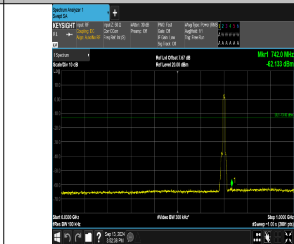
Band17_10MHz_16QAM_23780_50RB#0_30~1000_30~1000
