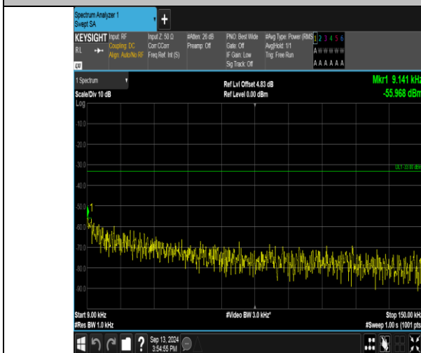
Band17_10MHz_QPSK_23790_1RB#49_0.009~0.15_0.009~0.15
