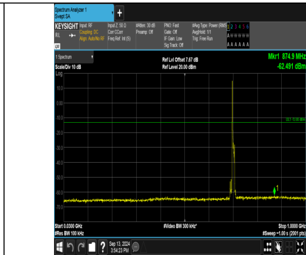
Band17_10MHz_16QAM_23790_1RB#0_30~1000_30~1000
