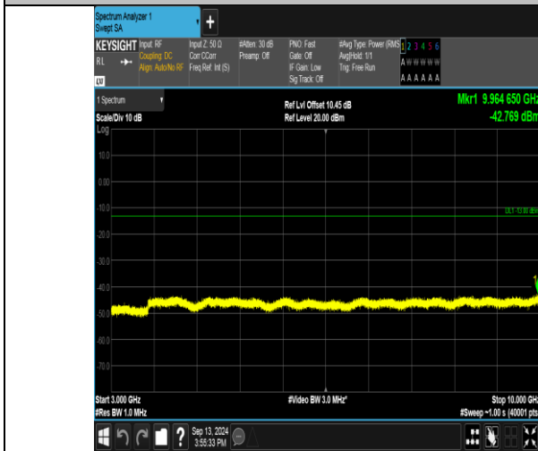
Band17_10MHz_QPSK_23790_1RB#49_3000~10000_3000~10000
