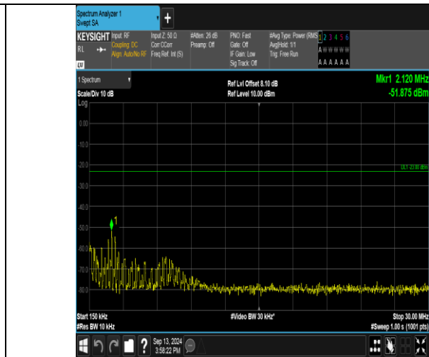
Band17_10MHz_QPSK_23800_1RB#0_0.15~30_0.15~30
