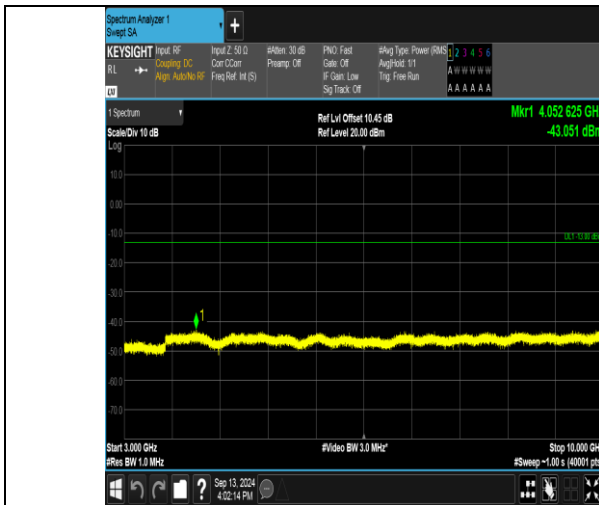
Band17_10MHz_QPSK_23800_50RB#0_3000~10000_3000~10000
