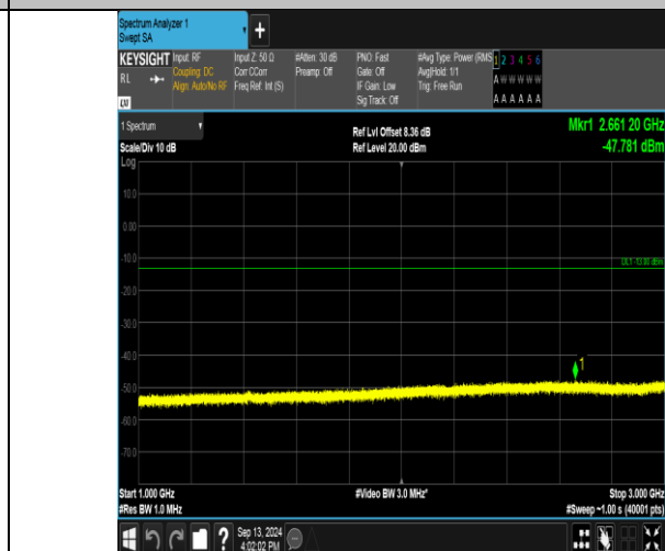
Band17_10MHz_QPSK_23800_50RB#0_1000~3000_1000~3000
