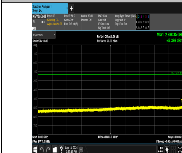
Band17_10MHz_16QAM_23790_50RB#0_1000~3000_1000~3000
