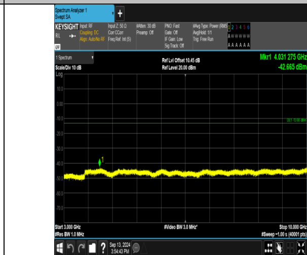
Band17_10MHz_16QAM_23790_1RB#0_3000~10000_3000~10000
