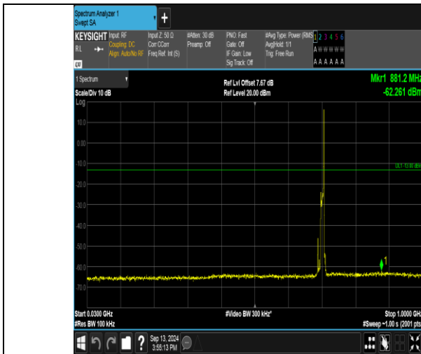
Band17_10MHz_QPSK_23790_1RB#49_30~1000_30~1000
