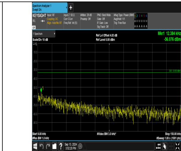
Band17_10MHz_16QAM_23780_50RB#0_0.009~0.15_0.009~0.15
