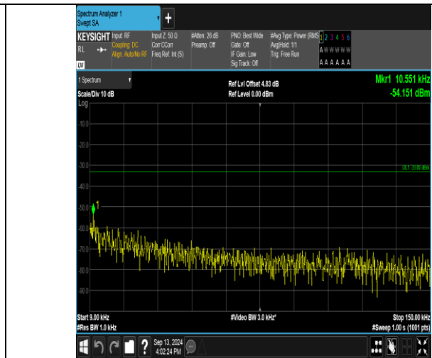
Band17_10MHz_16QAM_23800_50RB#0_0.009~0.15_0.009~0.15
