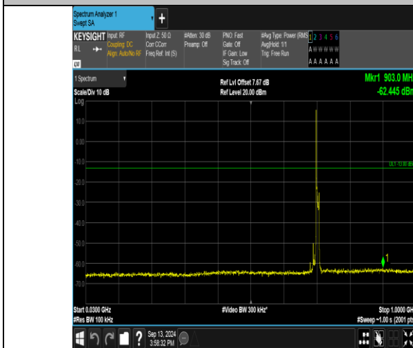
Band17_10MHz_QPSK_23800_1RB#0_30~1000_30~1000
