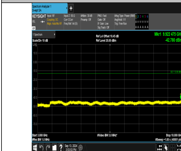
Band17_10MHz_QPSK_23790_1RB#0_3000~10000_3000~10000
