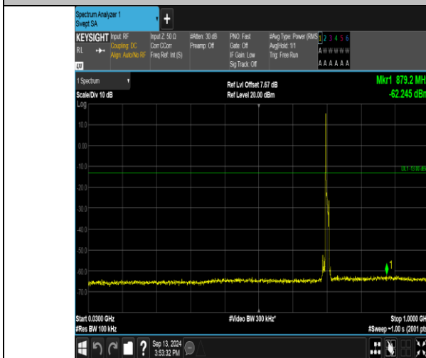
Band17_10MHz_QPSK_23790_1RB#0_30~1000_30~1000
