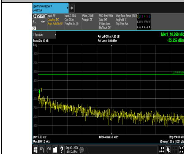
Band17_10MHz_QPSK_23800_50RB#0_0.009~0.15_0.009~0.15
