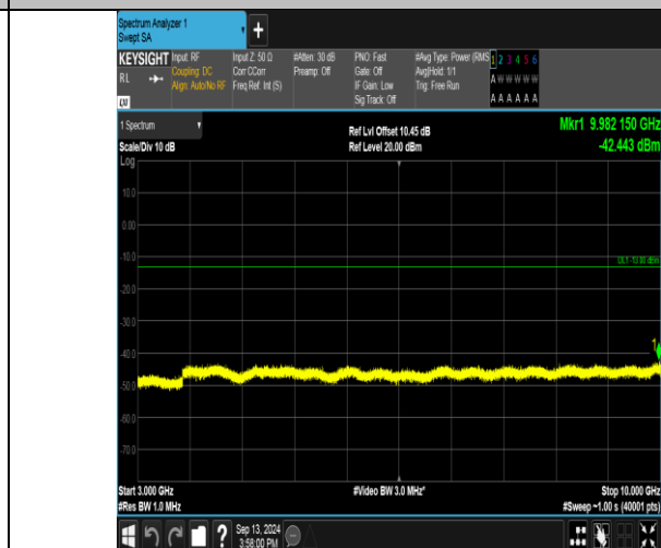
Band17_10MHz_16QAM_23790_50RB#0_3000~10000_3000~10000
