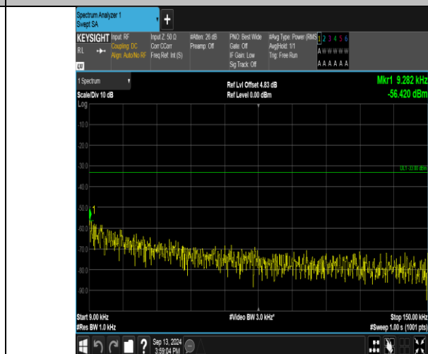
Band17_10MHz_16QAM_23800_1RB#0_0.009~0.15_0.009~0.15
