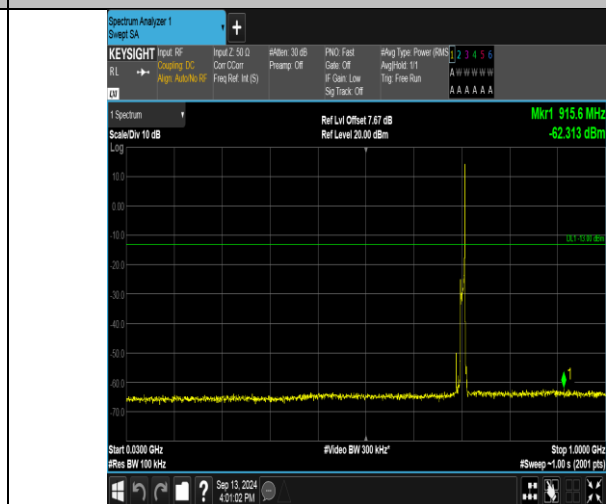
Band17_10MHz_16QAM_23800_1RB#49_30~1000_30~1000
