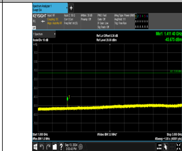
Band17_10MHz_QPSK_23790_1RB#0_1000~3000_1000~3000
