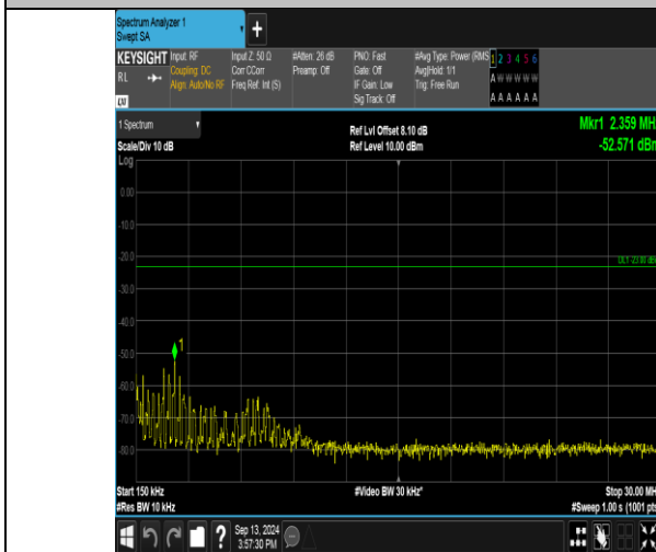
Band17_10MHz_16QAM_23790_50RB#0_0.15~30_0.15~30
