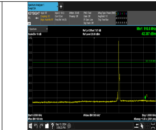
Band17_10MHz_16QAM_23800_1RB#0_30~1000_30~1000
