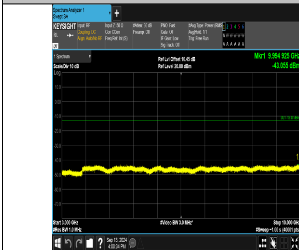
Band17_10MHz_QPSK_23800_1RB#49_3000~10000_3000~10000
