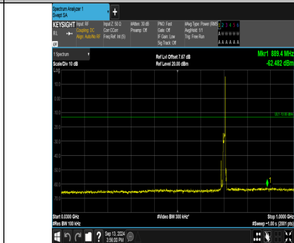
Band17_10MHz_16QAM_23790_1RB#49_30~1000_30~1000
