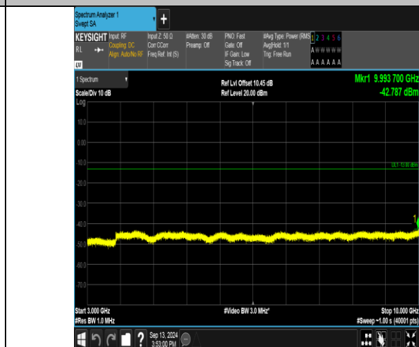
Band17_10MHz_16QAM_23780_50RB#0_3000~10000_3000~10000
