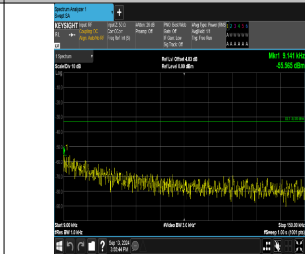
Band17_10MHz_16QAM_23790_1RB#49_0.009~0.15_0.009~0.15
