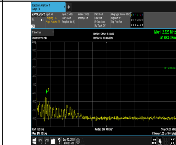
Band17_10MHz_QPSK_23800_1RB#49_0.15~30_0.15~30
