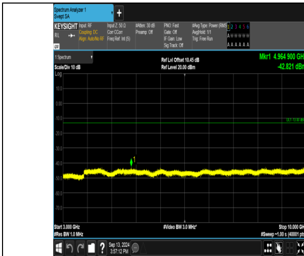
Band17_10MHz_QPSK_23790_50RB#0_3000~10000_3000~10000
