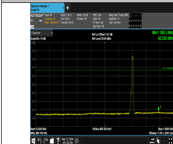
Band17_10MHz_QPSK_23800_50RB#0_30~1000_30~1000
