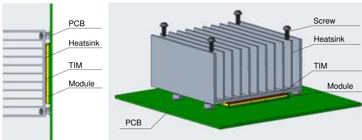
Figure 18: Placement and Fixing of the Heatsink
