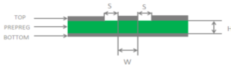
Figure 12: Coplanar Waveguide Design on a 2-layer PCB
