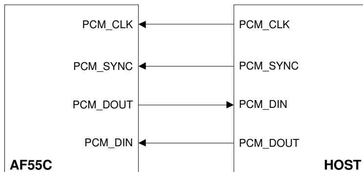
Figure 7: PCM Interface Connection
