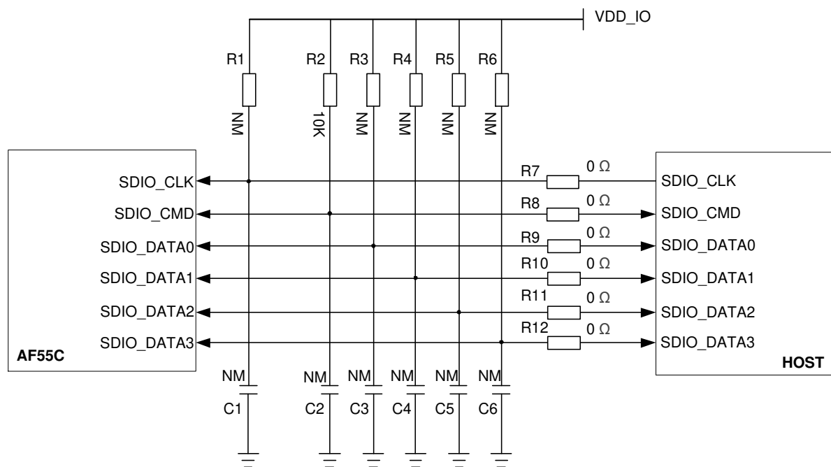
Figure 5: SDIO Interface Connection
