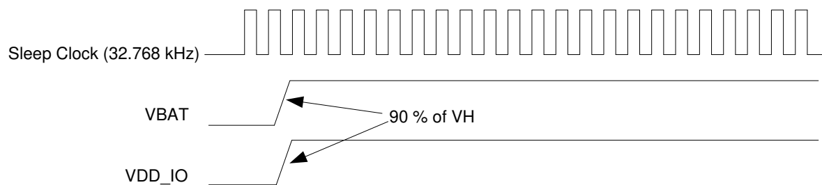
Figure 3: Power-up Timing
