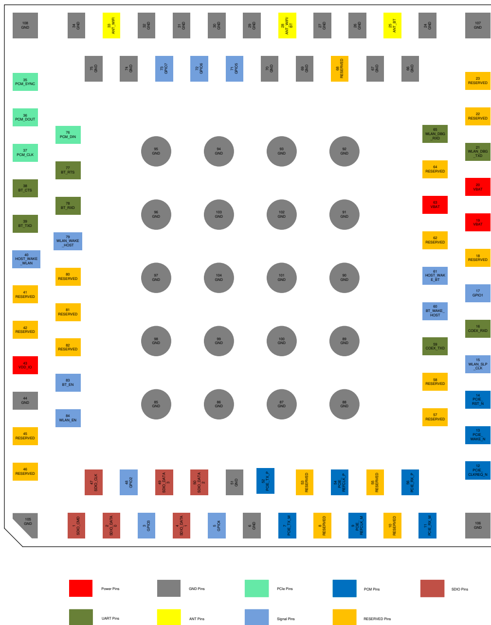
Figure 2: Pin Assignment (Top View)
