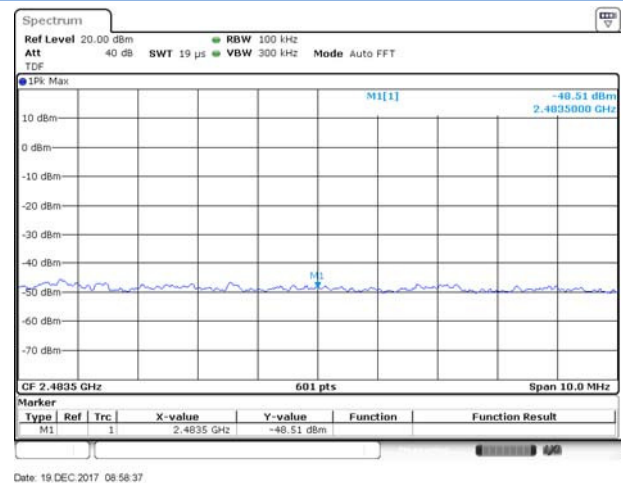
802.11g HIGH CHANNEL, Band Edge
