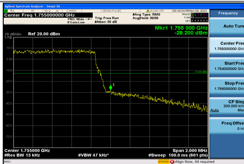
Band4-1.4MHz-16QAM-20393-6RB#0
