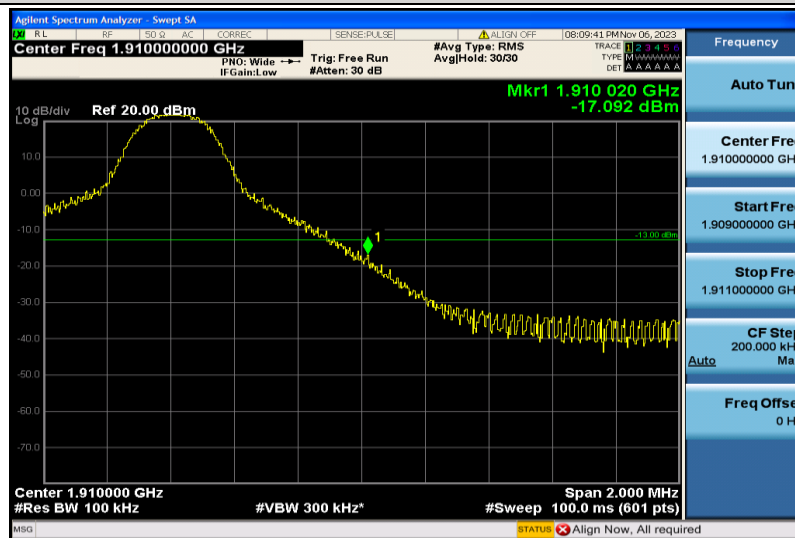
Band2-10MHz-16QAM-19150-1RB#49
