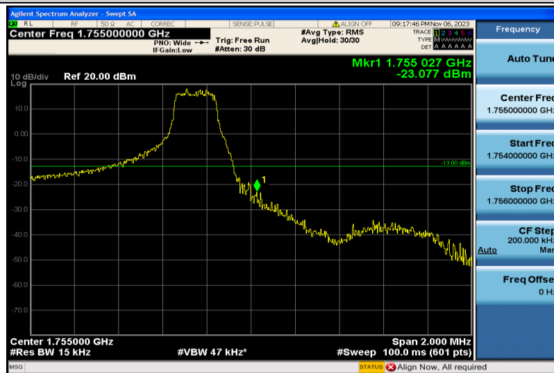
Band4-1.4MHz-16QAM-20393-1RB#5
