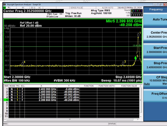
BLE_1M-Ant1-2402-PASS
