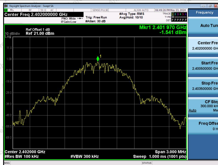
BLE_1M-Ant1-2402-0~Reference-PASS
