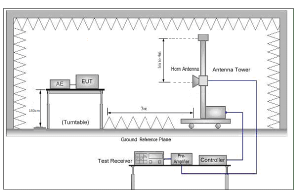
Figure 2. Above 1 GHz
