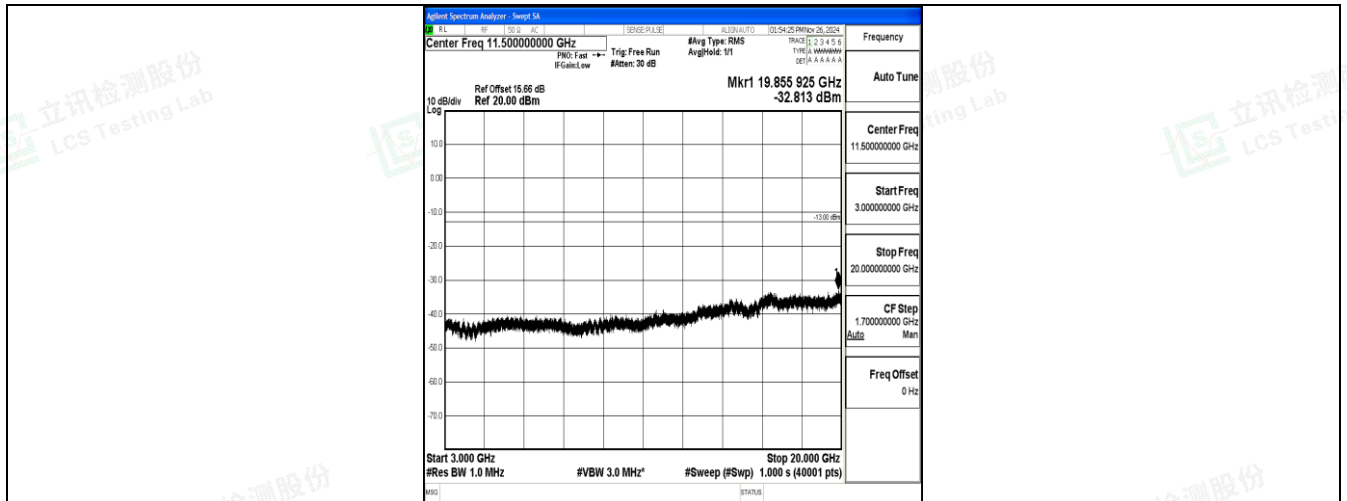
Band2_15MHz_16QAM_18900_1RB#0_3000~20000_3000~20000
