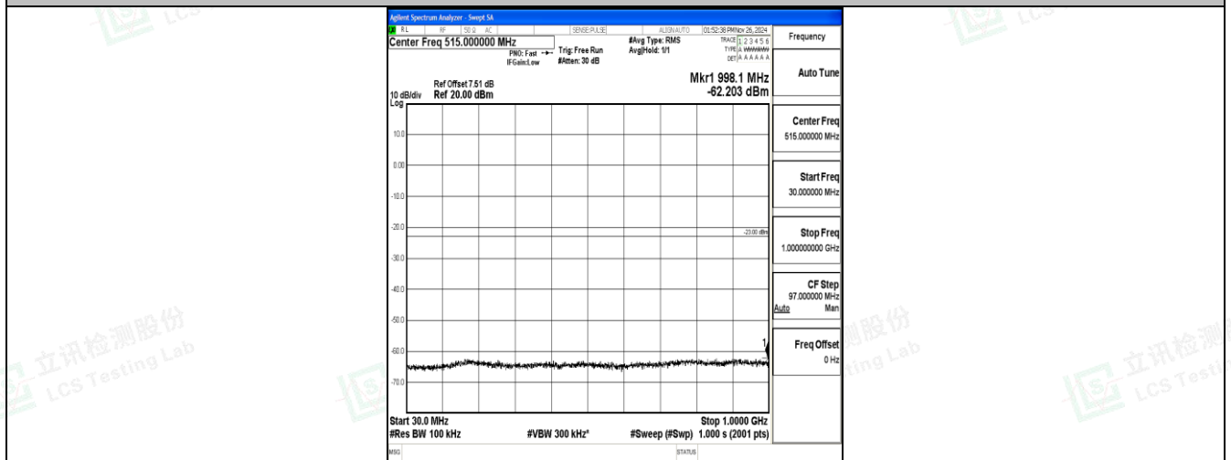
Band2_15MHz_QPSK_18675_1RB#0_30~1000_30~1000
