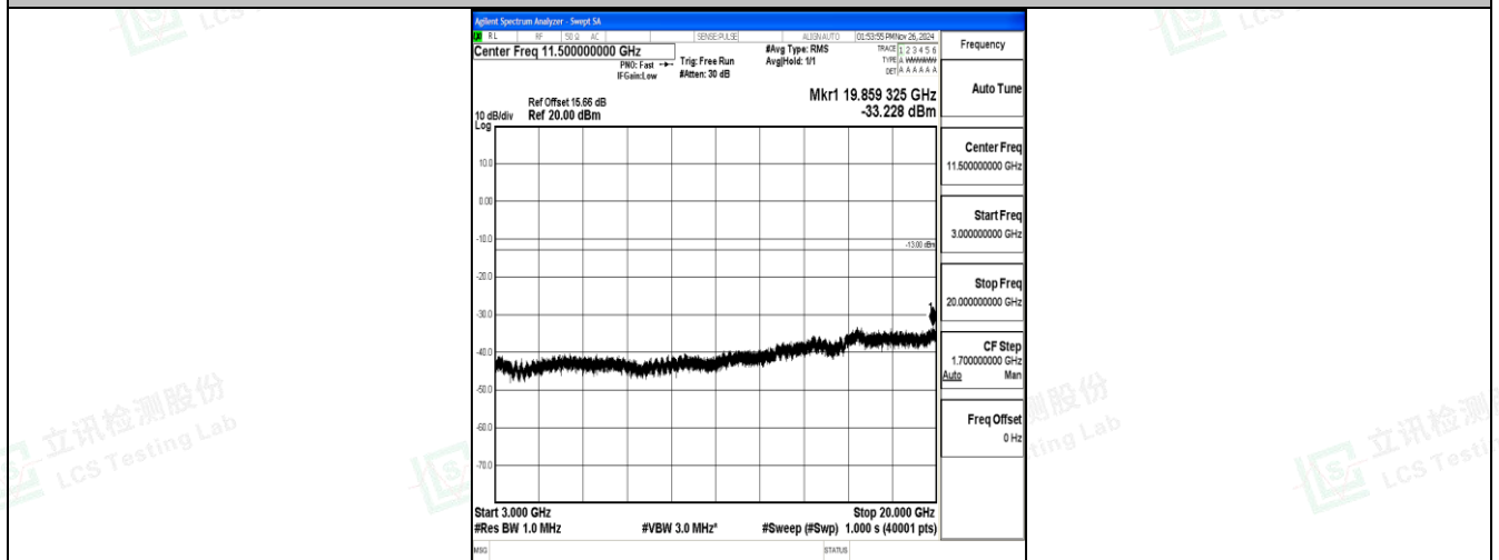
Band2_15MHz_QPSK_18900_1RB#0_3000~20000_3000~20000
