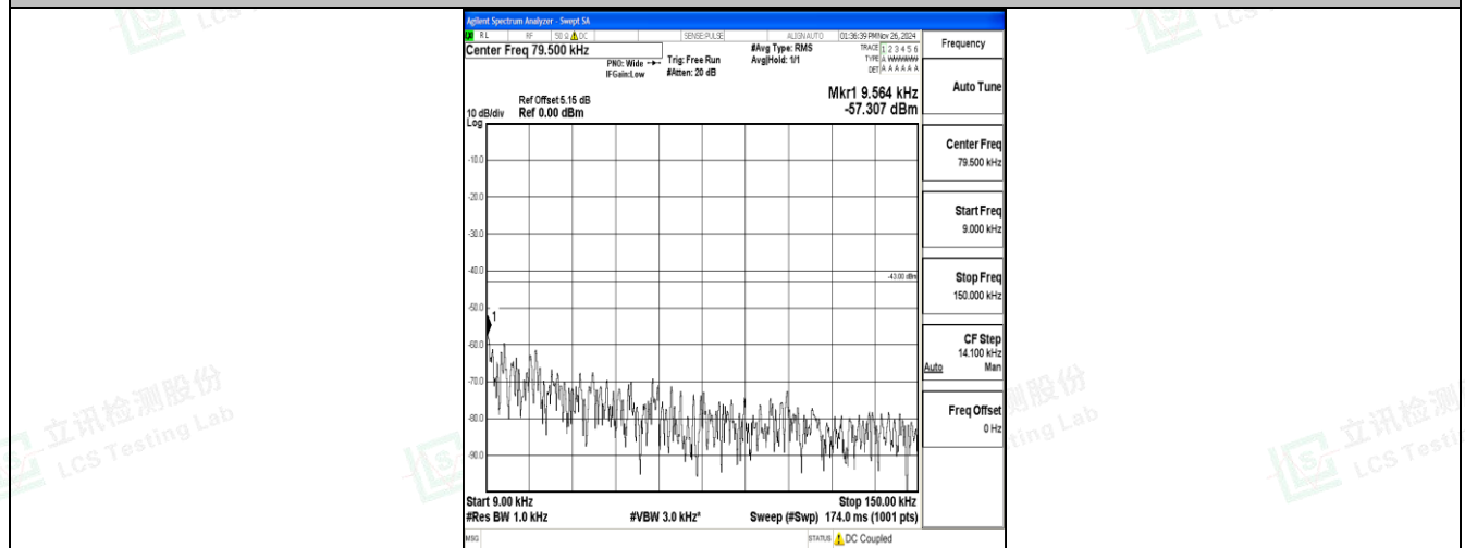
Band2_10MHz_16QAM_18650_1RB#0_0.009~0.15_0.009~0.15
