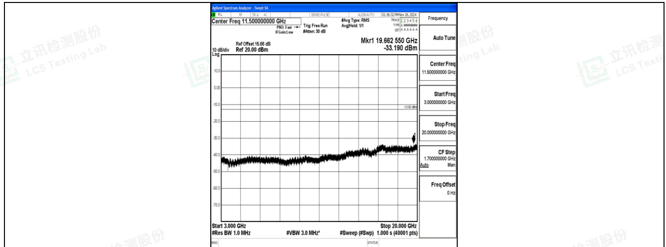
Band2_10MHz_QPSK_18650_1RB#0_3000~20000_3000~20000
