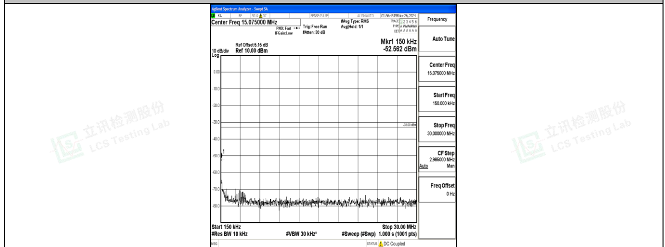
Band2_10MHz_16QAM_18650_1RB#0_0.15~30_0.15~30
