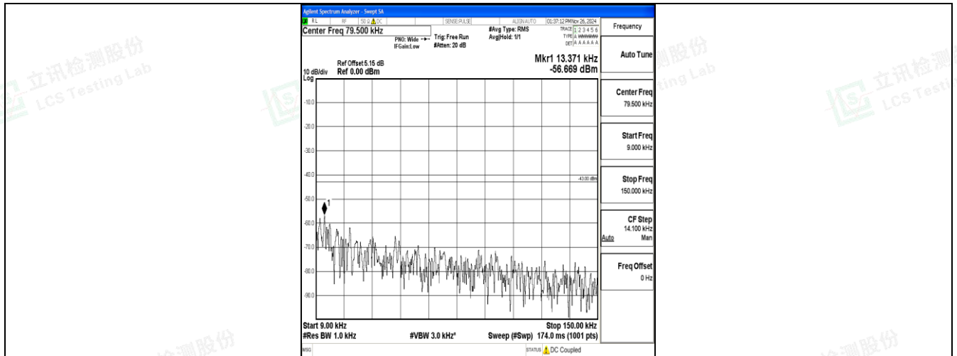
Band2_10MHz_QPSK_18900_1RB#0_0.009~0.15_0.009~0.15
