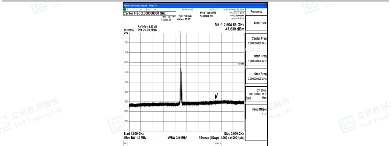
Band2_15MHz_QPSK_19125_1RB#0_1000~3000_1000~3000
