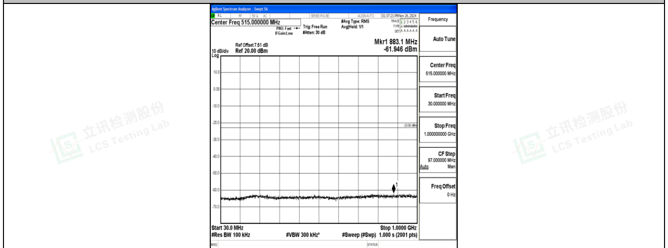
Band2_10MHz_QPSK_18900_1RB#0_30~1000_30~1000
