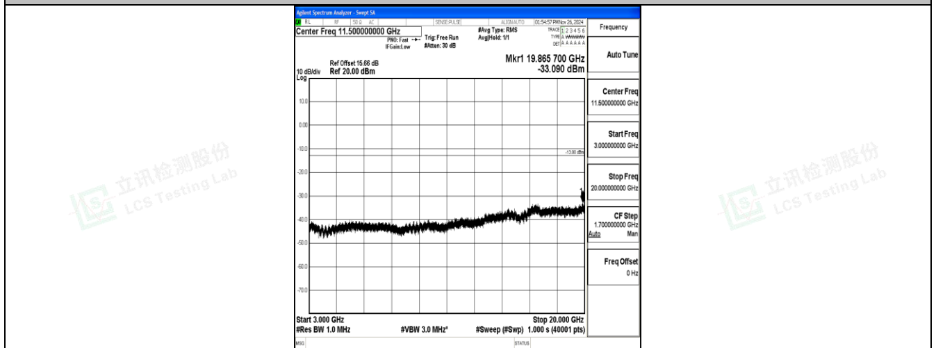
Band2_15MHz_QPSK_19125_1RB#0_3000~20000_3000~20000
