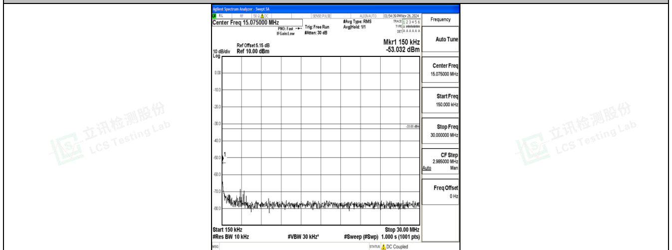
Band2_15MHz_QPSK_19125_1RB#0_0.15~30_0.15~30
