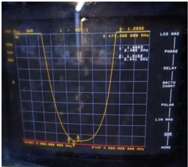
(c) VSWR
