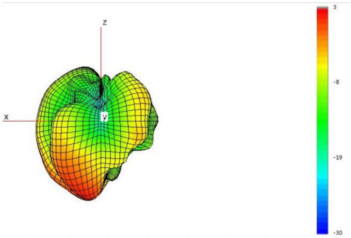
(f) 3D gain pattern, Y+
