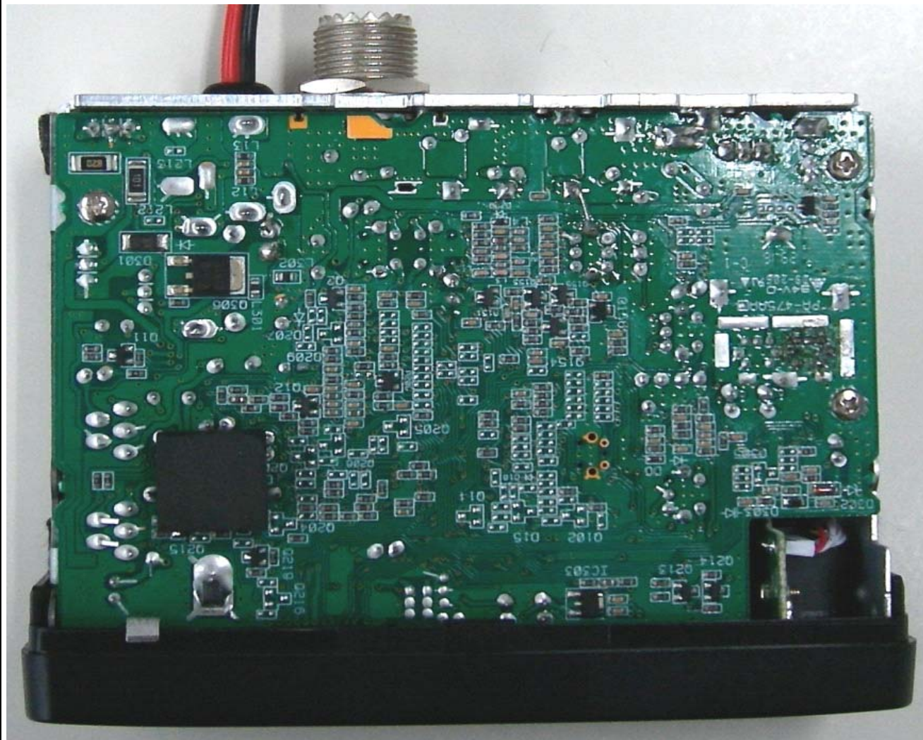
Main PCB Bottom View
