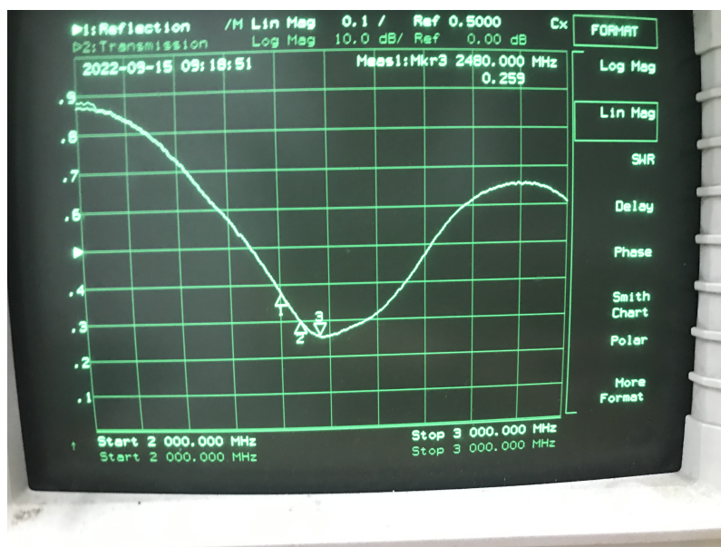
Figure 2 Dongle Antenna S11
