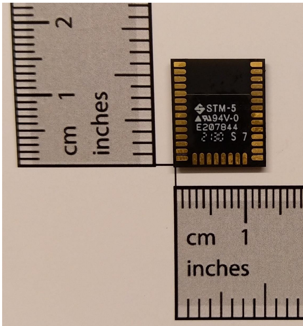
Figure 4: Bottom/Rear External View of the MGM240P32A Modules
