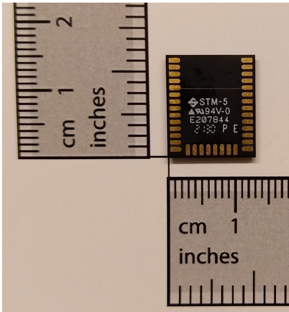
Figure 2: Bottom/Rear External View of the MGM240P22A Modules
