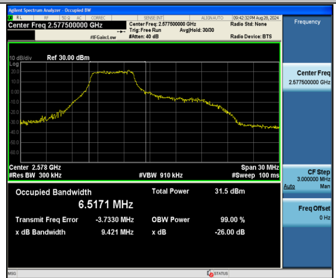
Band38-15MHz-16QAM-37825-27RB#0-PASS
