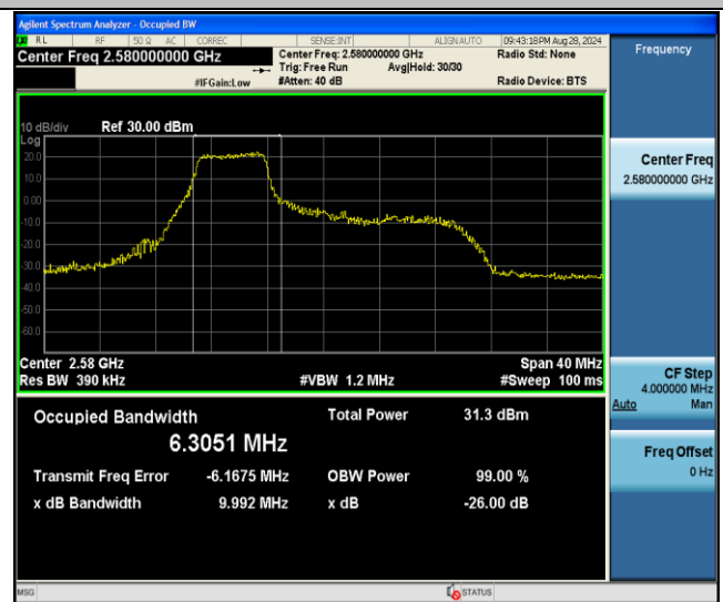
Band38-20MHz-16QAM-37850-27RB#0-PASS
