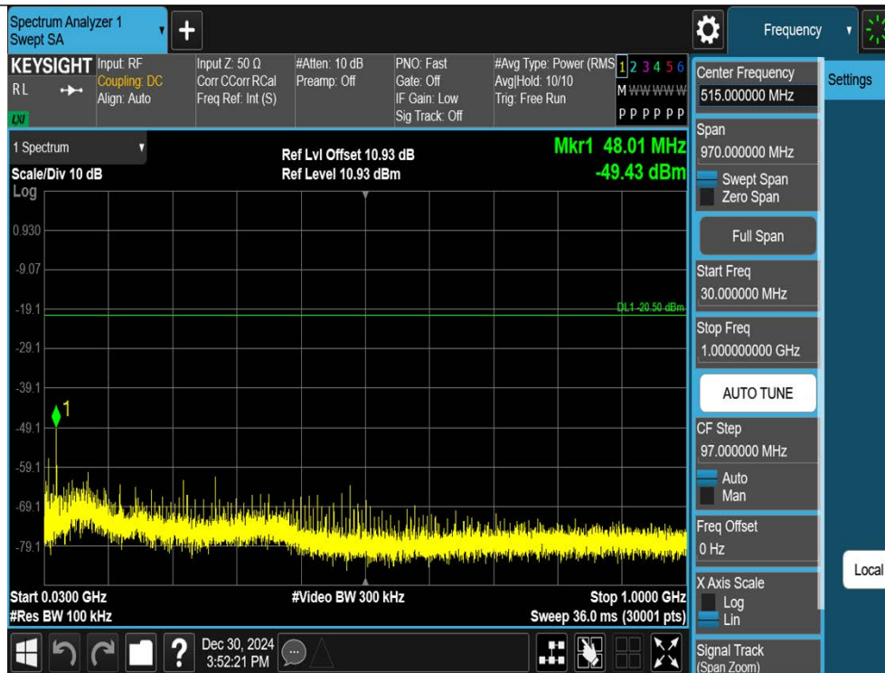
2DH5-Ant1-2480-30~1000-PASS
