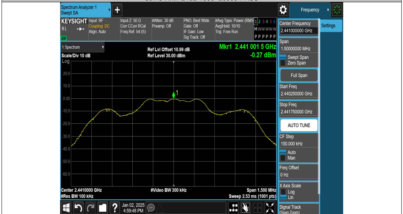
3DH5-Ant1-2441-0~Reference-PASS
