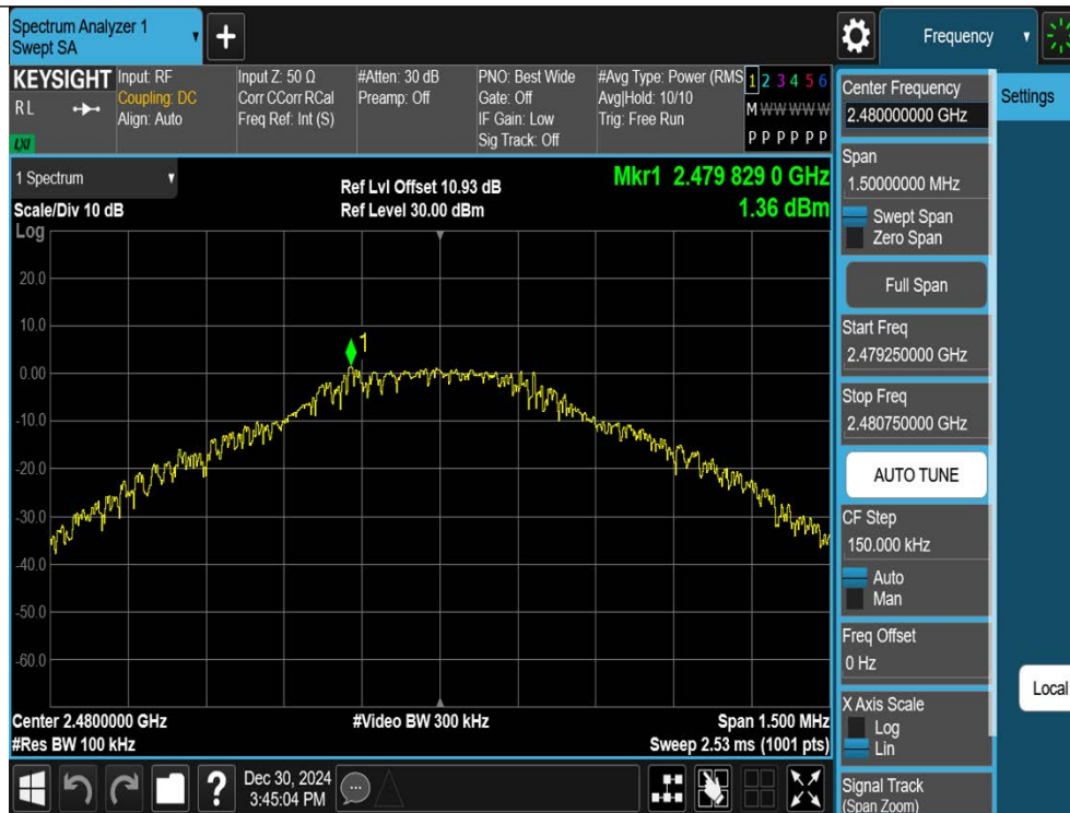
DH5-Ant1-2480-0~Reference-PASS
