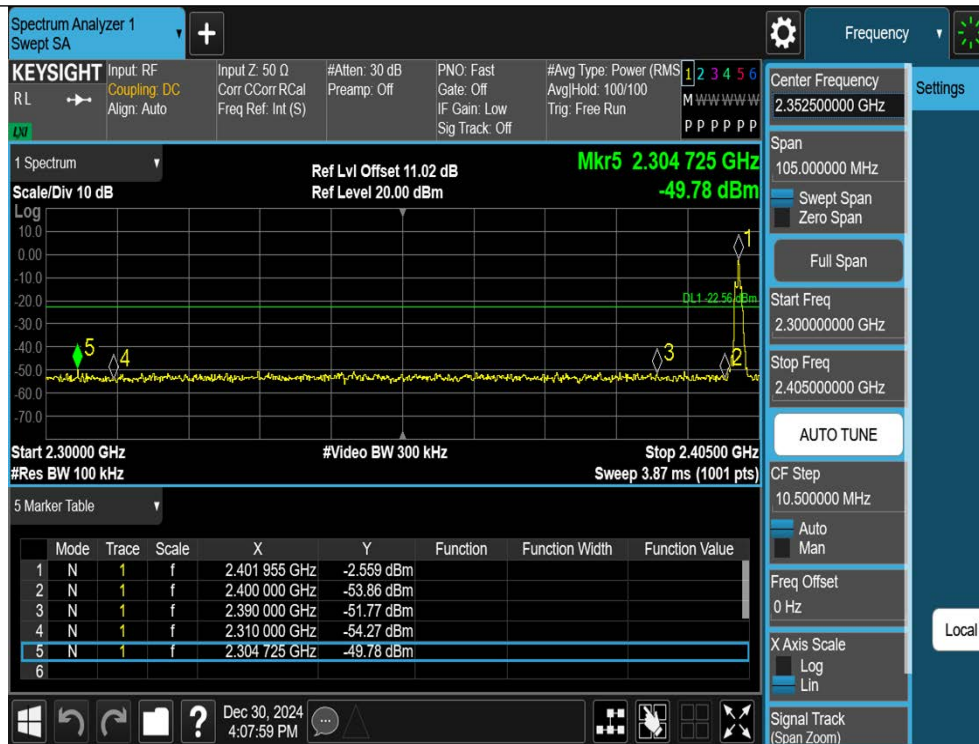
3DH5-Ant1-2402-PASS
