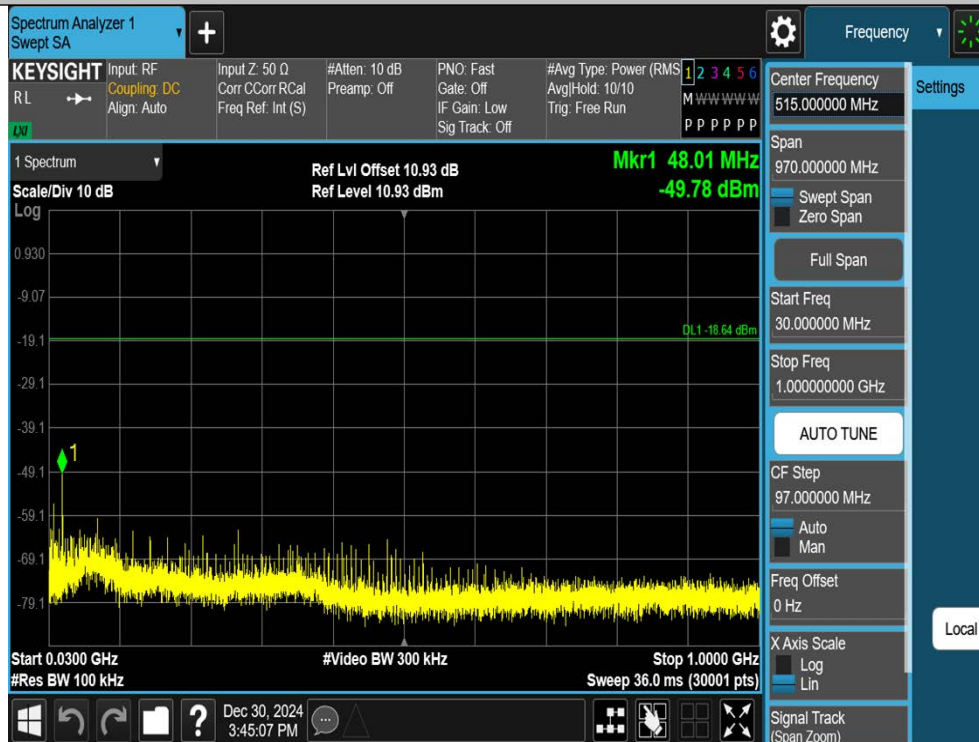
DH5-Ant1-2480-30~1000-PASS
