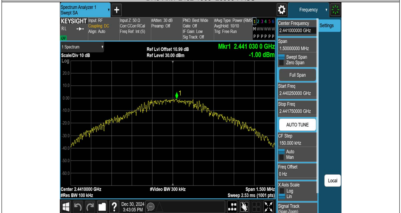
DH5-Ant1-2441-0~Reference-PASS
