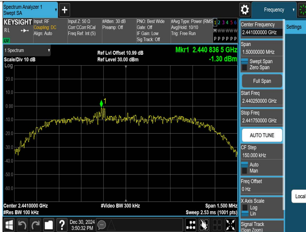
2DH5-Ant1-2441-0~Reference-PASS
