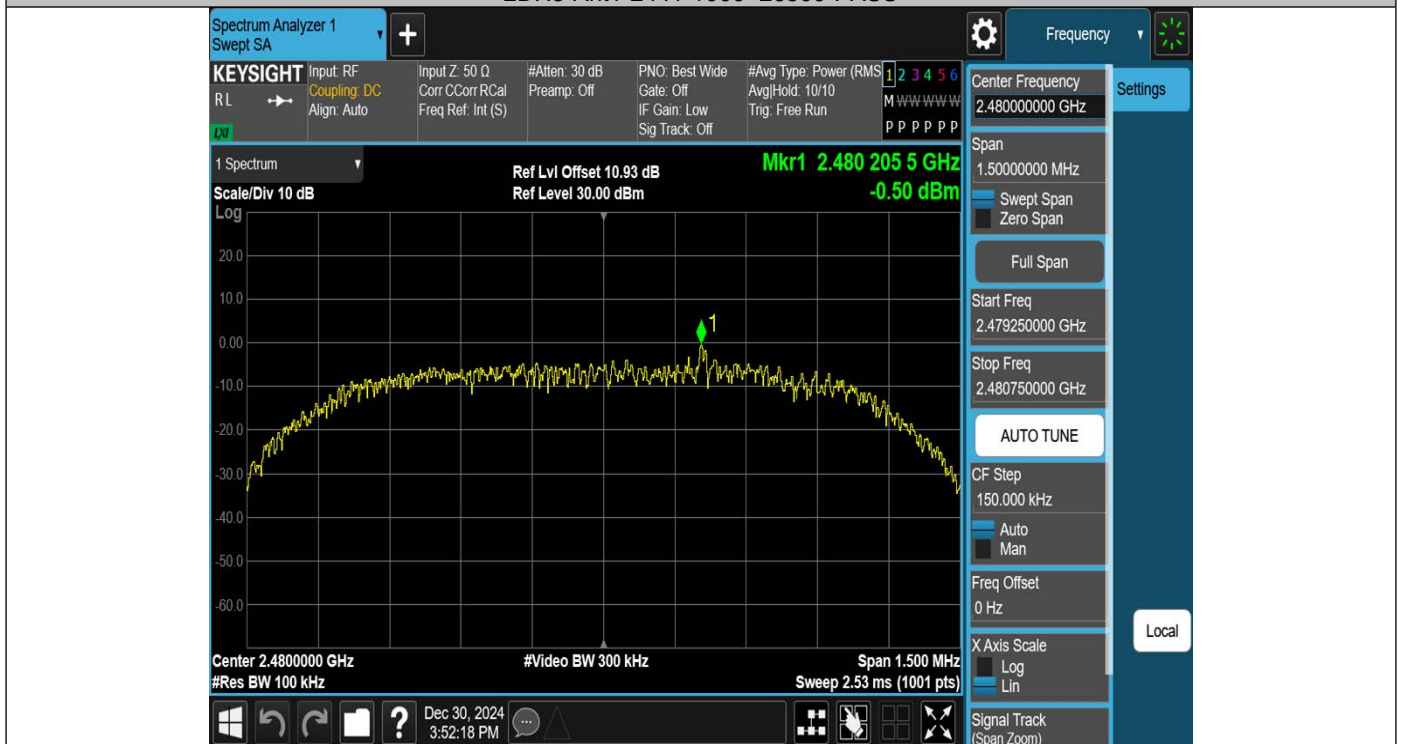
2DH5-Ant1-2480-0~Reference-PASS
