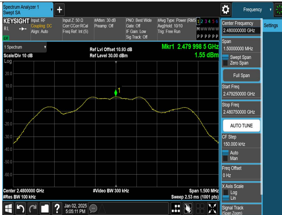
3DH5-Ant1-2480-0~Reference-PASS
