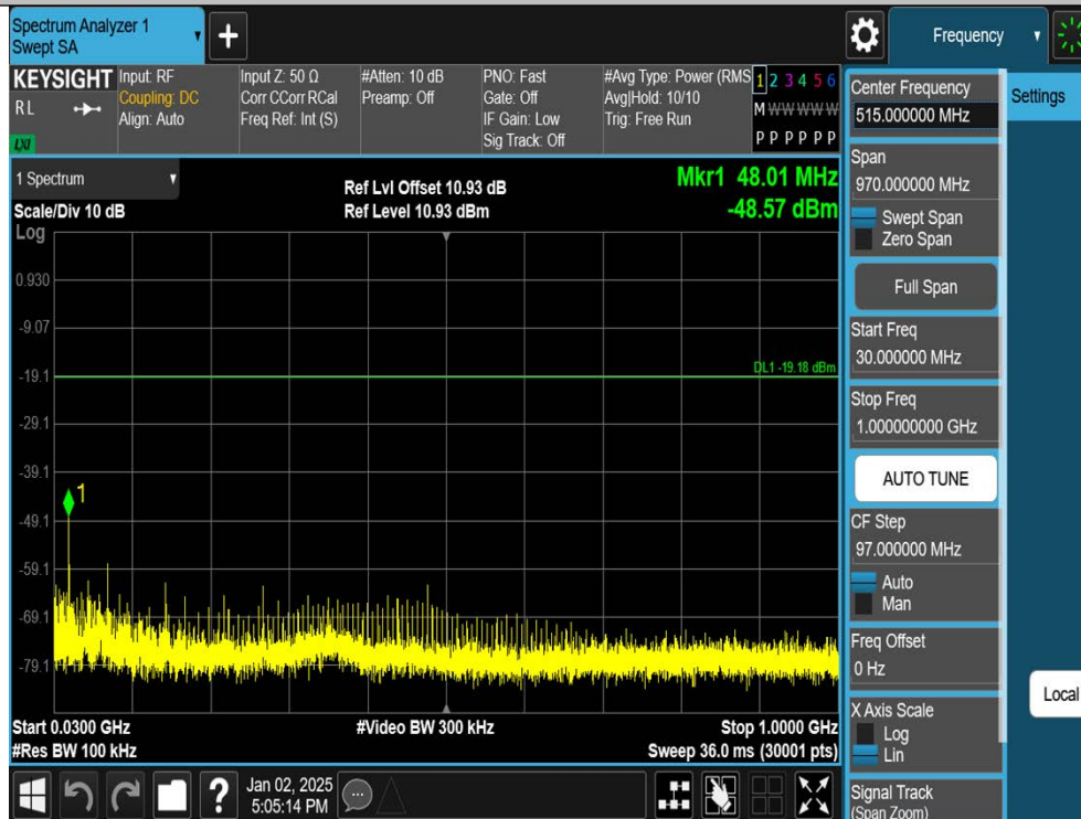
3DH5-Ant1-2480-30~1000-PASS
