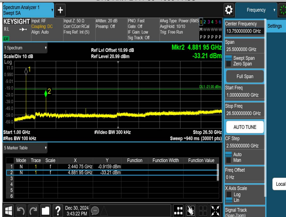
DH5-Ant1-2441-1000~26500-PASS
