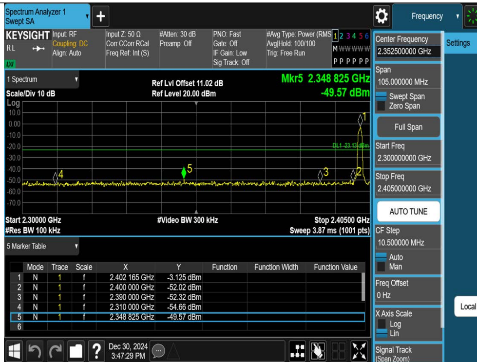
2DH5-Ant1-2402-PASS
