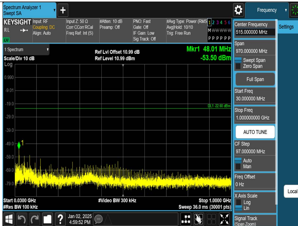
3DH5-Ant1-2441-30~1000-PASS
