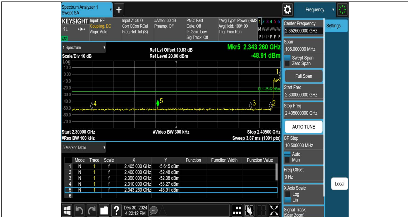
2DH5-Ant1-Hop_2402-PASS
