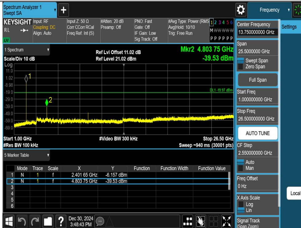
2DH5-Ant1-2402-1000~26500-PASS
