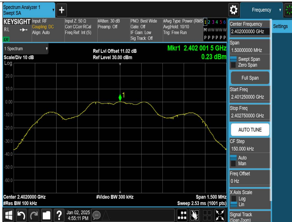
3DH5-Ant1-2402-0~Reference-PASS
