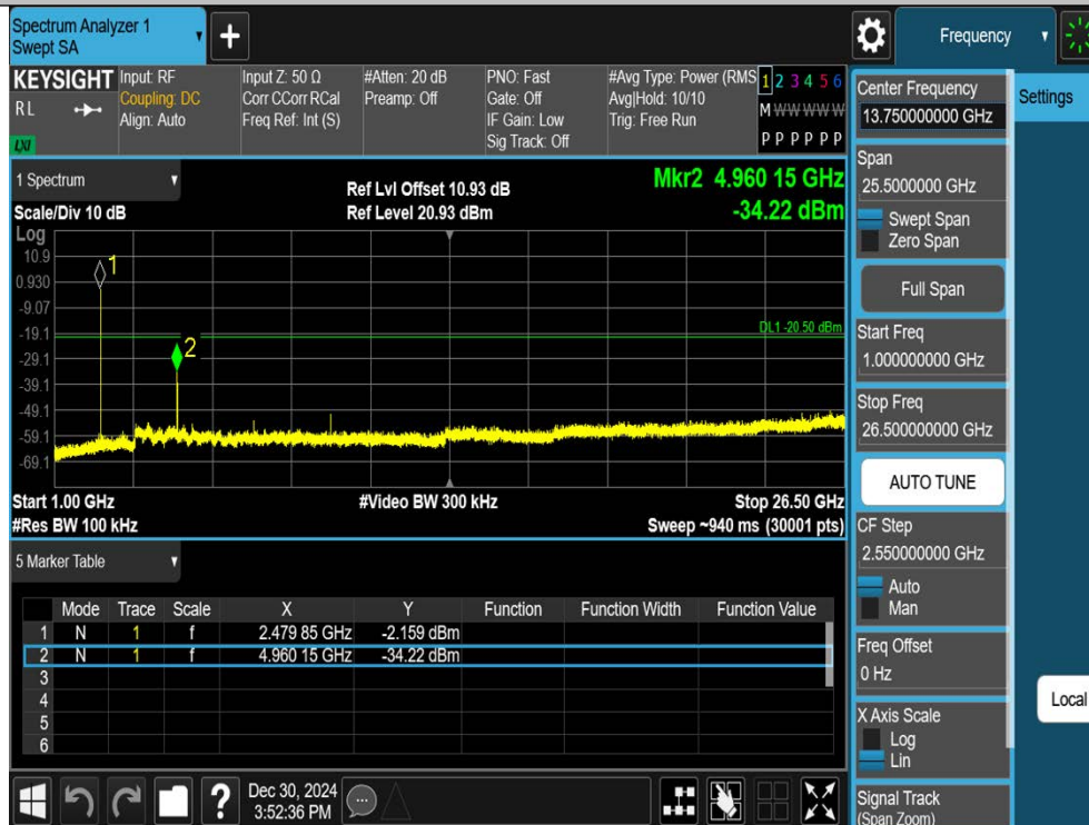
2DH5-Ant1-2480-1000~26500-PASS
