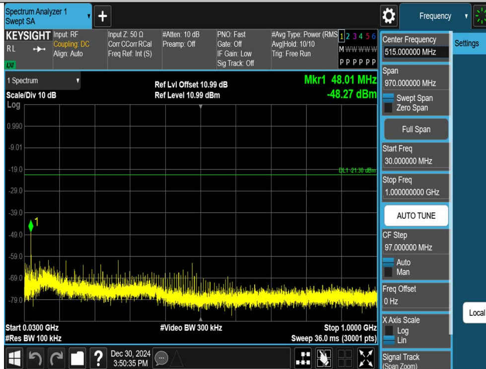
2DH5-Ant1-2441-30~1000-PASS
