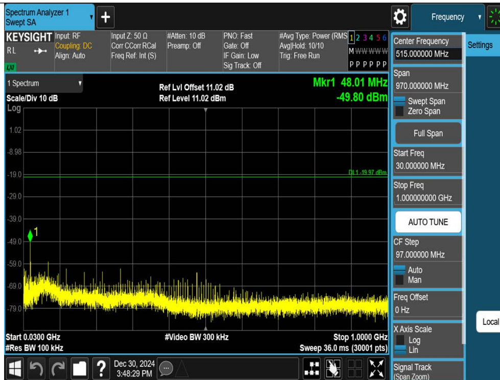
2DH5-Ant1-2402-30~1000-PASS
