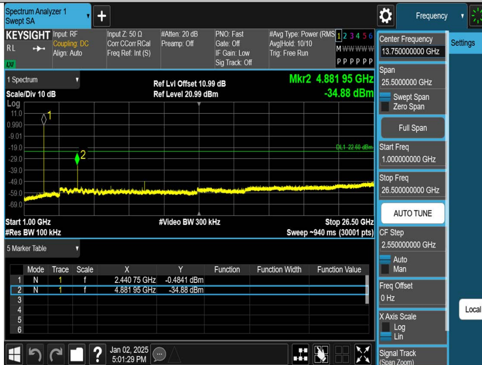
3DH5-Ant1-2441-1000~26500-PASS
