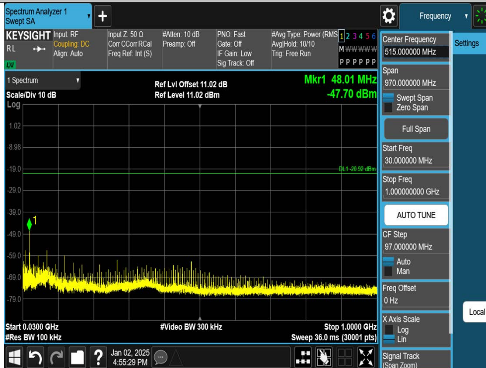
3DH5-Ant1-2402-30~1000-PASS
