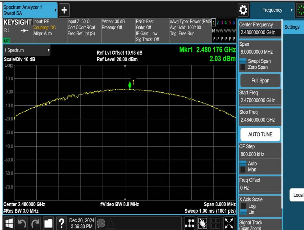
3DH5-Ant1-2480-PASS
