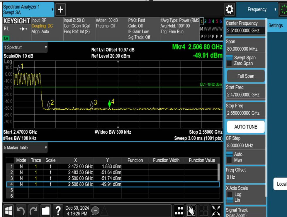
DH5-Ant1-Hop_2480-PASS
