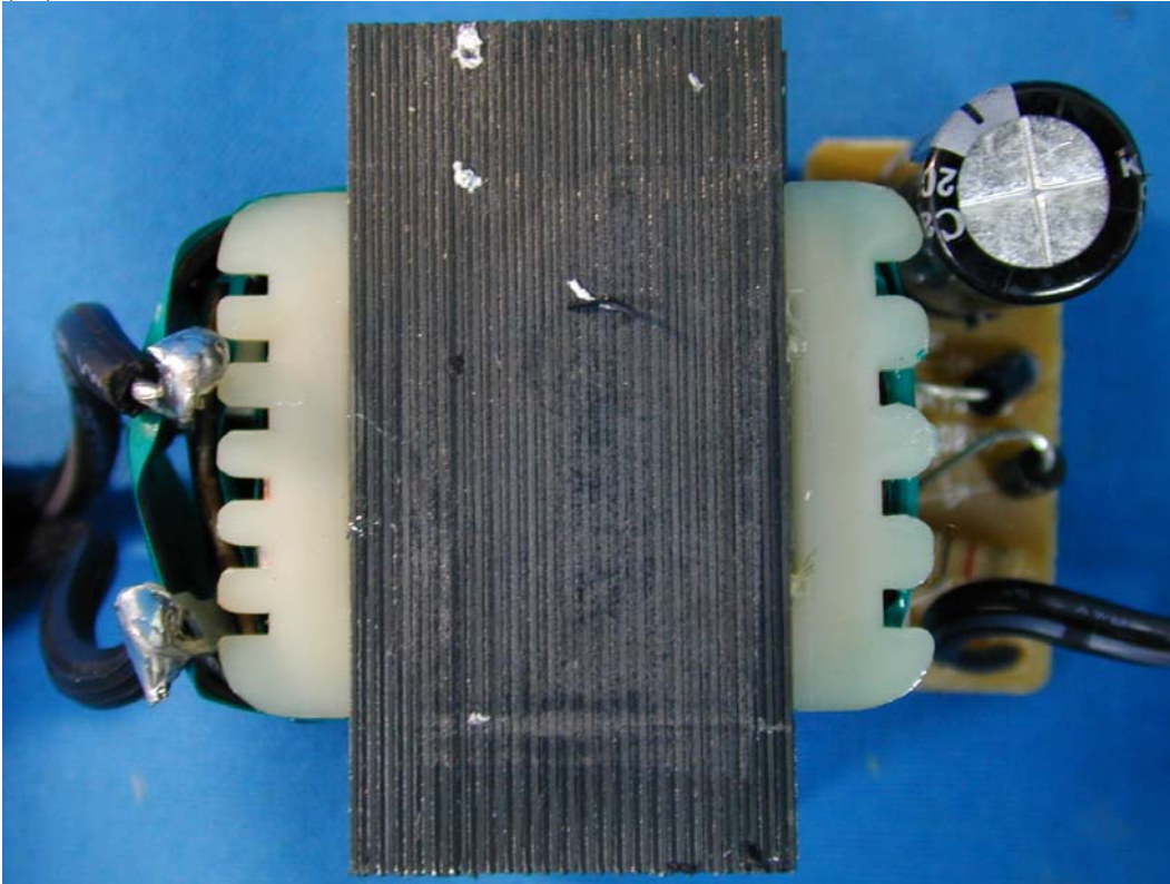
(15) EUT Photo-Mode 1
