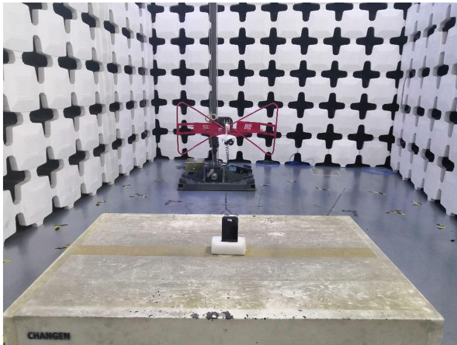
14. Radiated Emissions (Part 22/24/27,,30MHz-1GHz)
