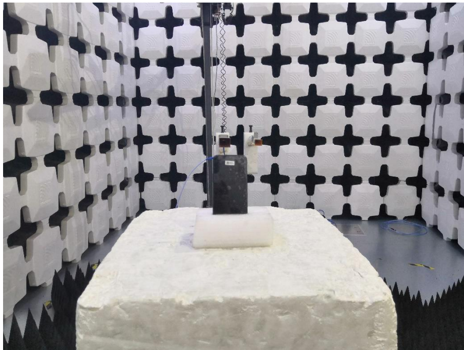
16. Radiated Emissions (Par22/24/27, 18GHz -26.5GHz)
