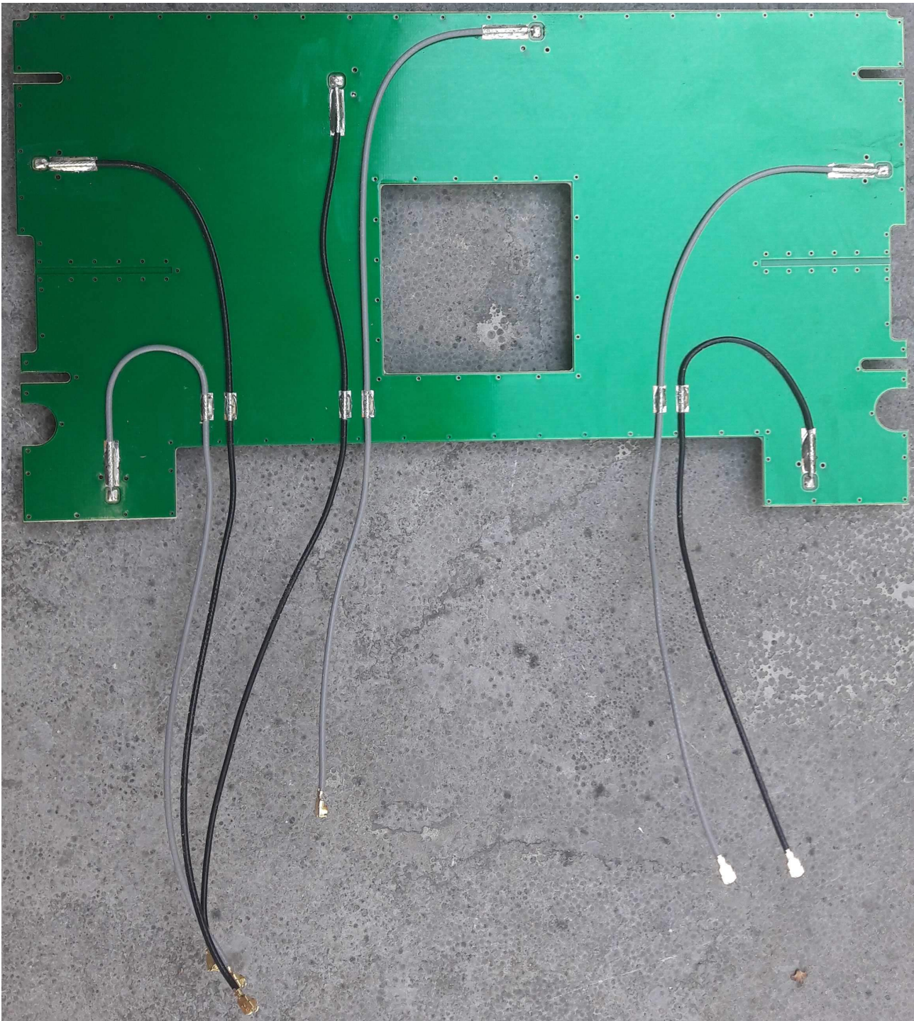
Antenna – backside view
