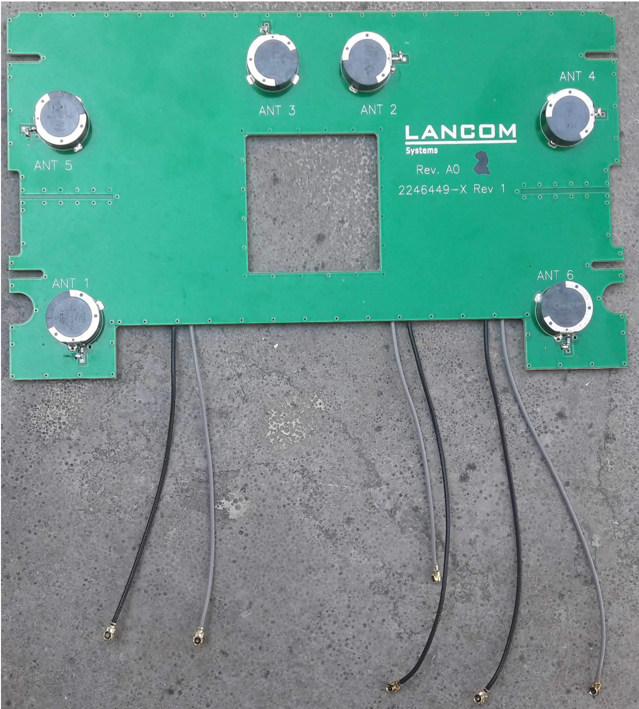
Antenna – front view
