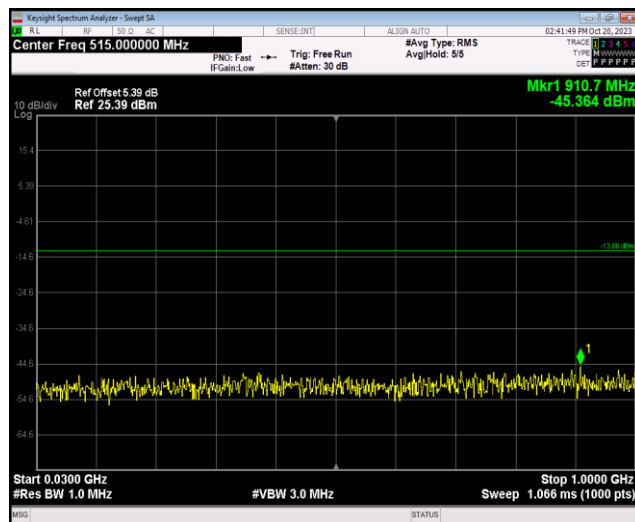
Band2-1.4MHz-QPSK-19193-1RB#0-Range1:30~10 00MHz
