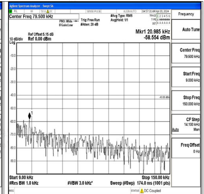
Band4_20MHz_16QAM_20175_1RB#0_0.009~0.15_0.0 09~0.15
