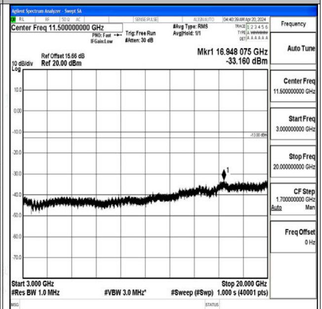
Band4_15MHz_16QAM_20175_1RB#0_3000~20000_3000~20000
