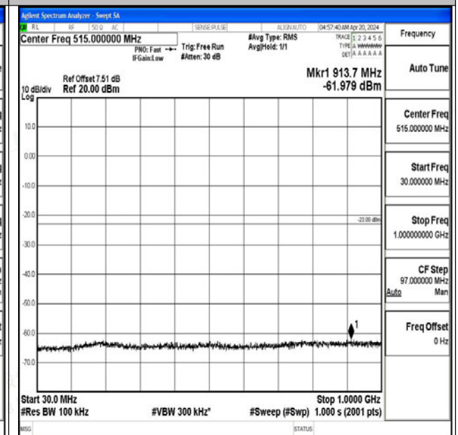
Band4_20MHz_16QAM_20175_1RB#0_30~1000_30~10 00
