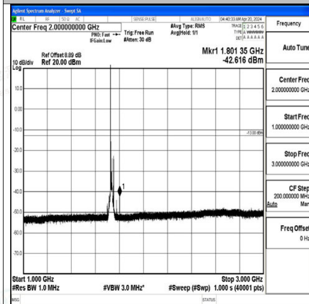
Band4_15MHz_16QAM_20175_1RB#0_1000~3000_1000~3000
