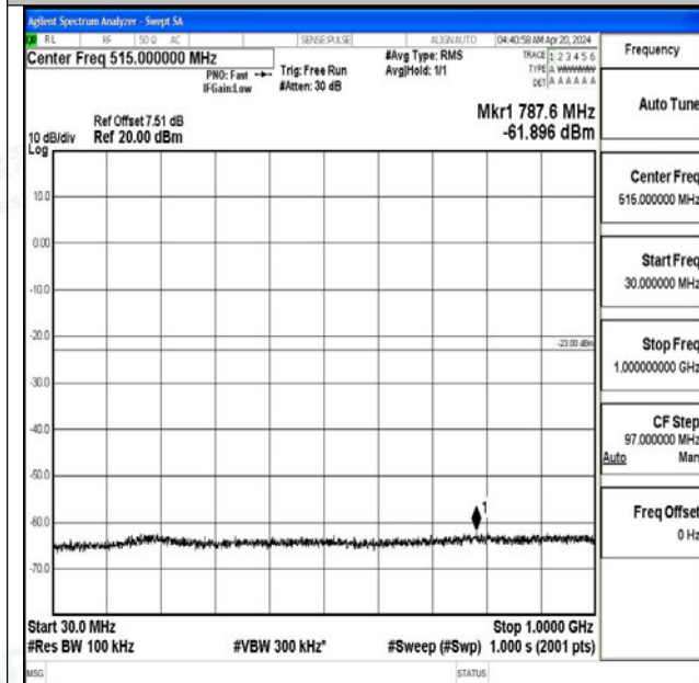
Band4_15MHz_QPSK_20325_1RB#0_30~1000_30~1000
