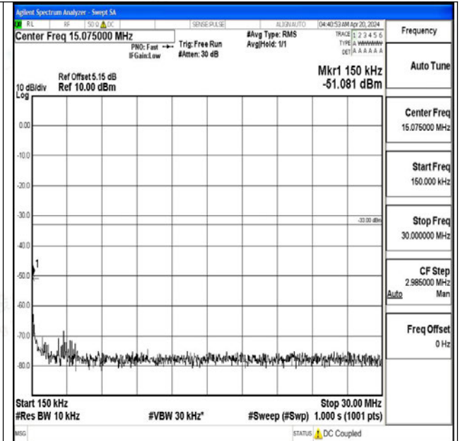
Band4_15MHz_QPSK_20325_1RB#0_0.15~30_0.15~30
