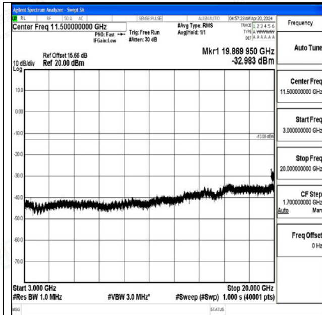
Band4_20MHz_QPSK_20175_1RB#0_3000~20000_300 0~20000
