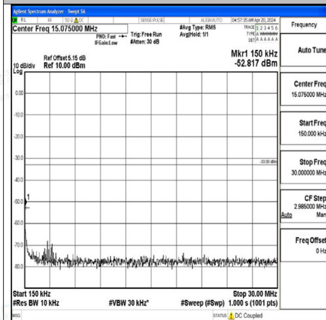
Band4_20MHz_16QAM_20175_1RB#0_0.15~30_0.15~3 0
