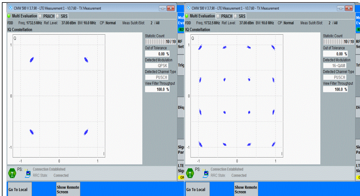
Band4-10MHz-QPSK-20175-50RB#0-PASS
