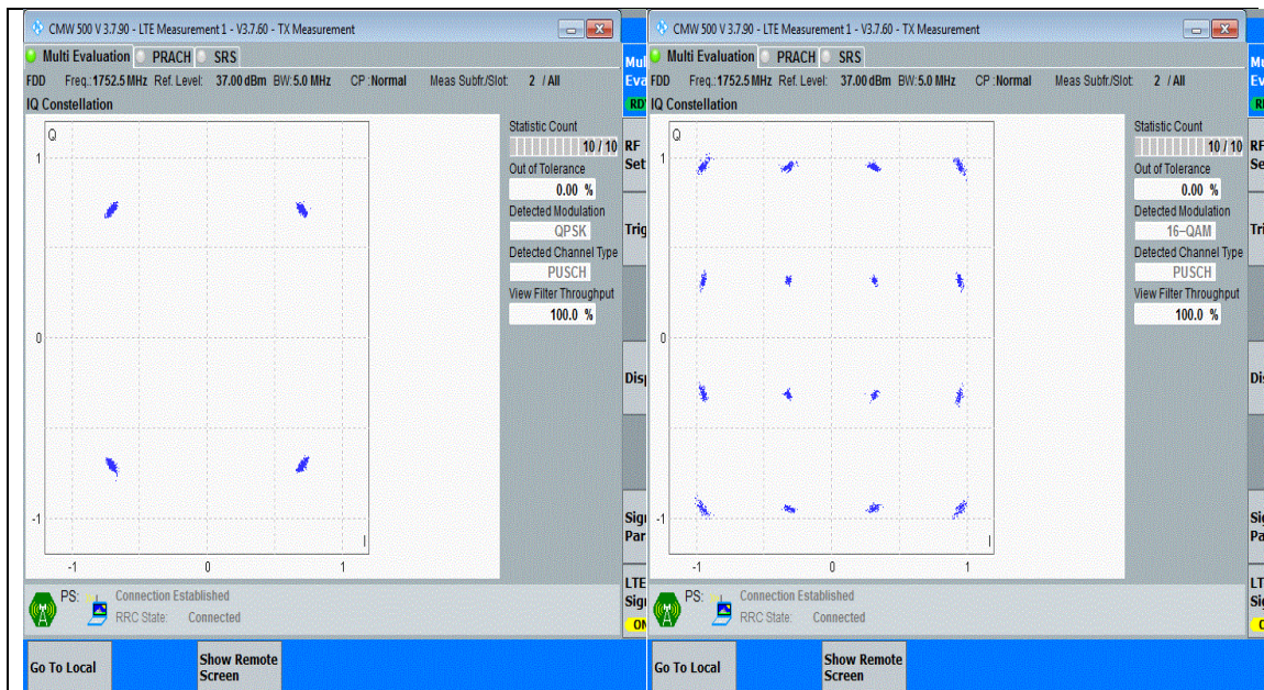
Band4-5MHz-QPSK-20375-25RB#0-PASS
