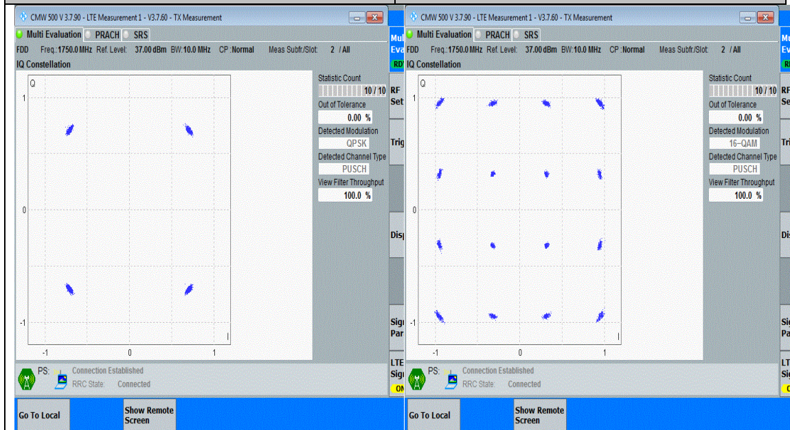
Band4-10MHz-QPSK-20350-50RB#0-PASS
