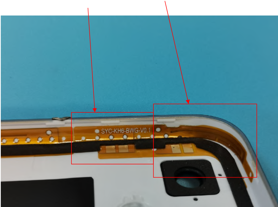
5G WIFI Antenna 2.4G WIFI/BT Antenna
