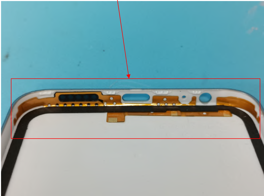
2G/3G/4G DIV Antenna
