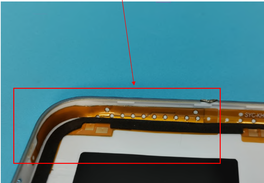
5G WIFI Antenna 2.4G WIFI/BT Antenna
