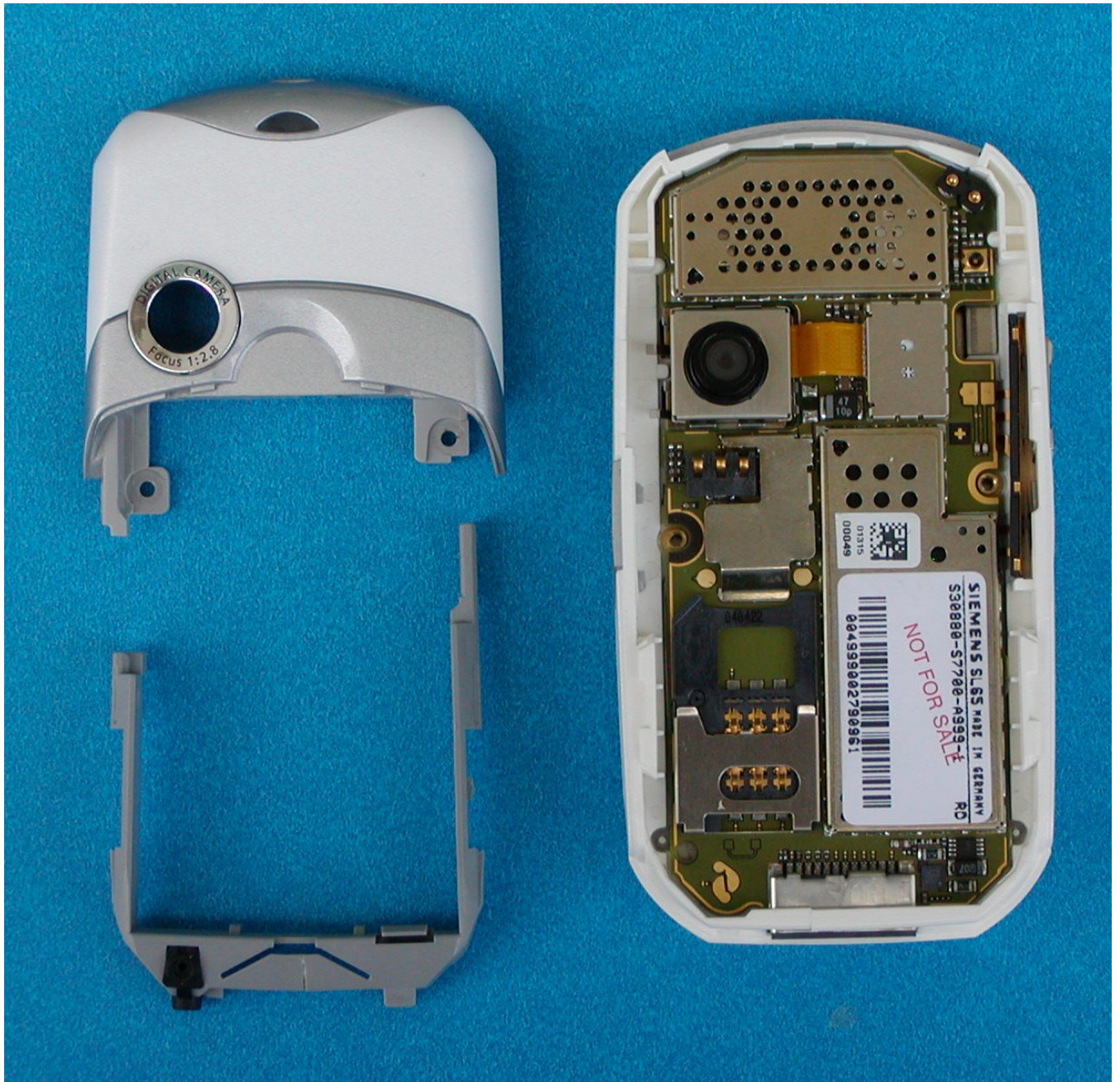
SL65 Disassembly step 1
