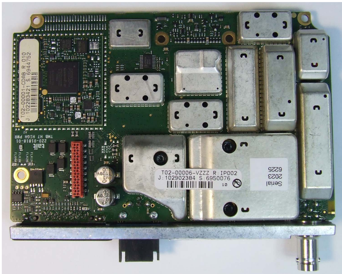
Photograph 01: Radio - Main PCB top with shields
