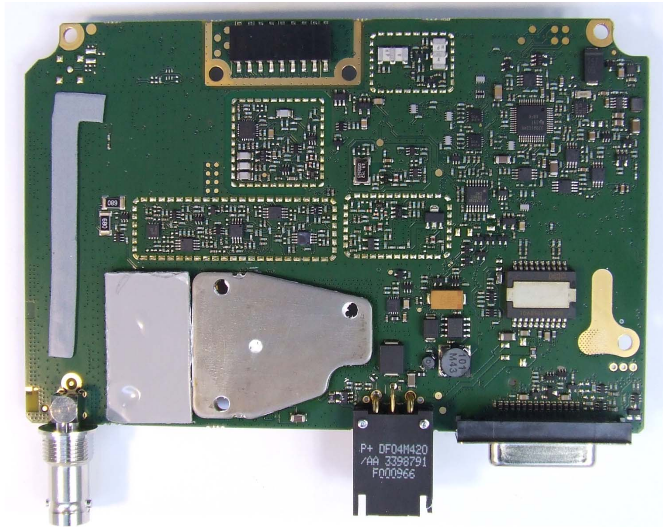
Photograph 04: Radio - Main PCB bottom without shields
