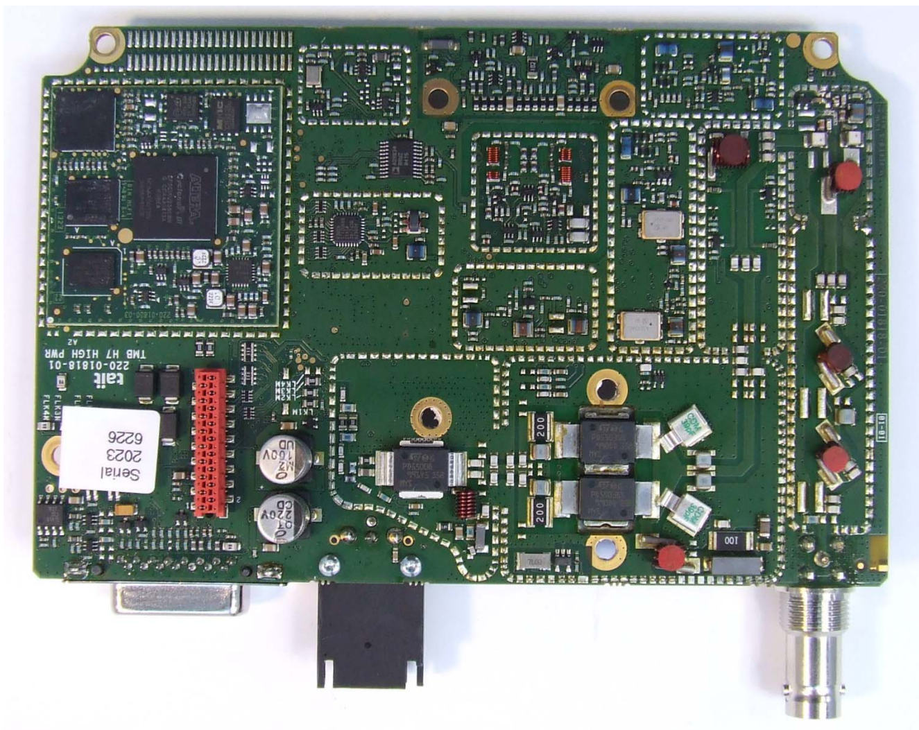
Photograph 02: Radio - Main PCB top without shields
