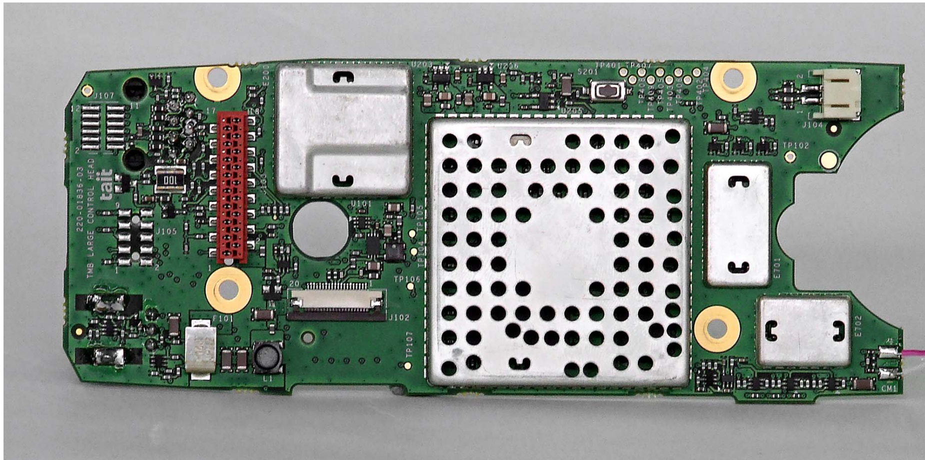
Photograph 07: Control Head - main PCB top with shields
