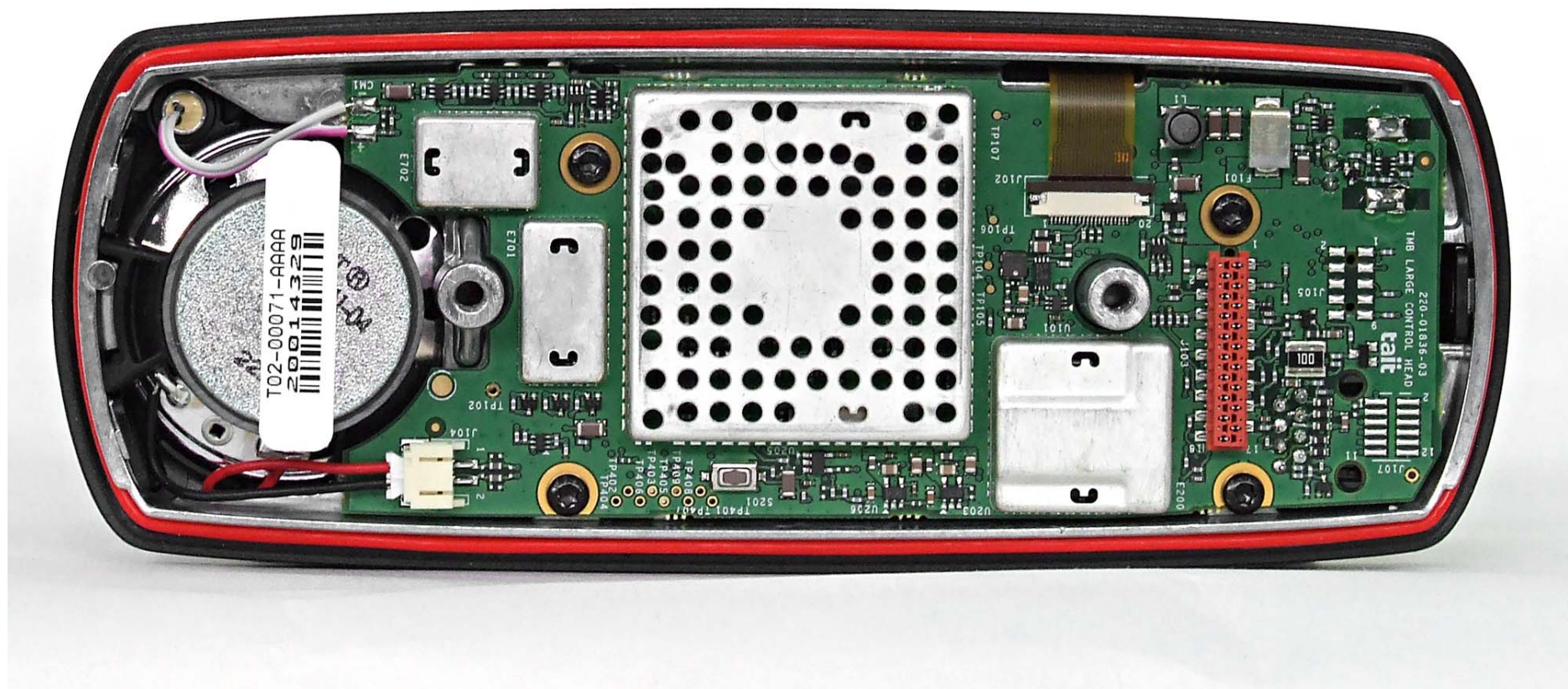
Photograph 05: Control Head - internal
