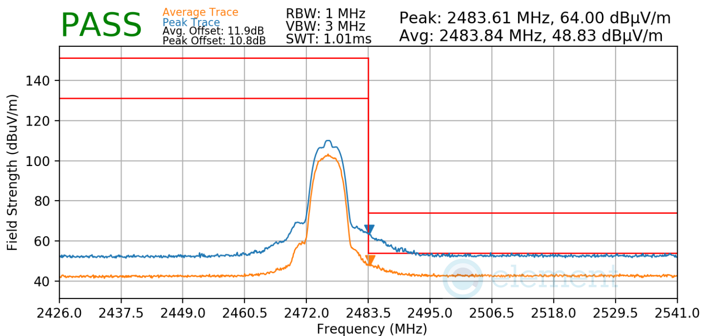
Plot 7-49. Radiated Restricted Upper Band Edge Measurement
