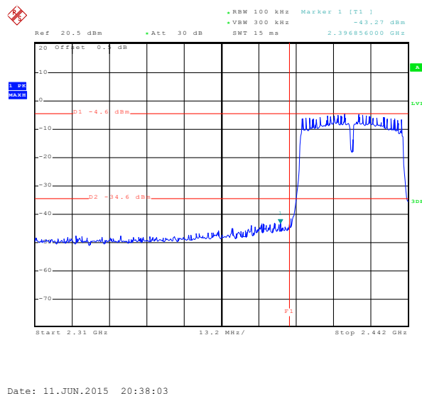
Lowest channel
