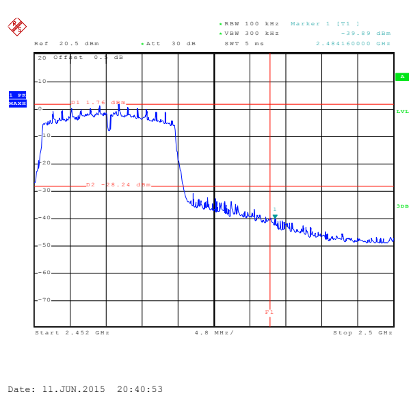
Highest channel
