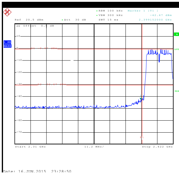
Lowest channel
