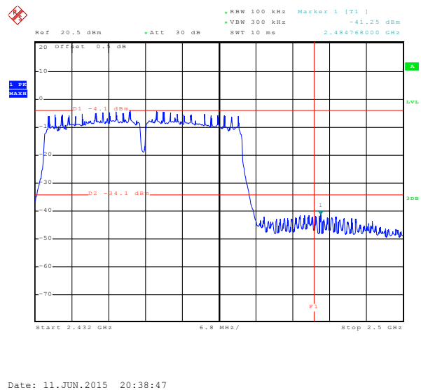
Highest channel
