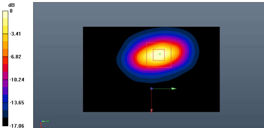
Fig.B.2. Validation 1750MHz 250mW
