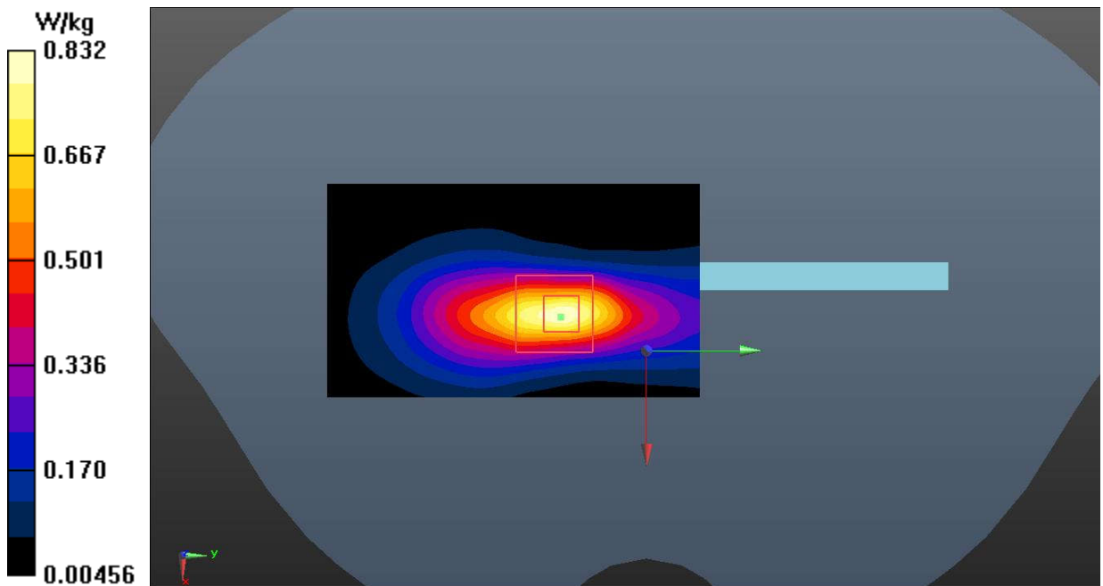
Fig.32 LTE Band 41
