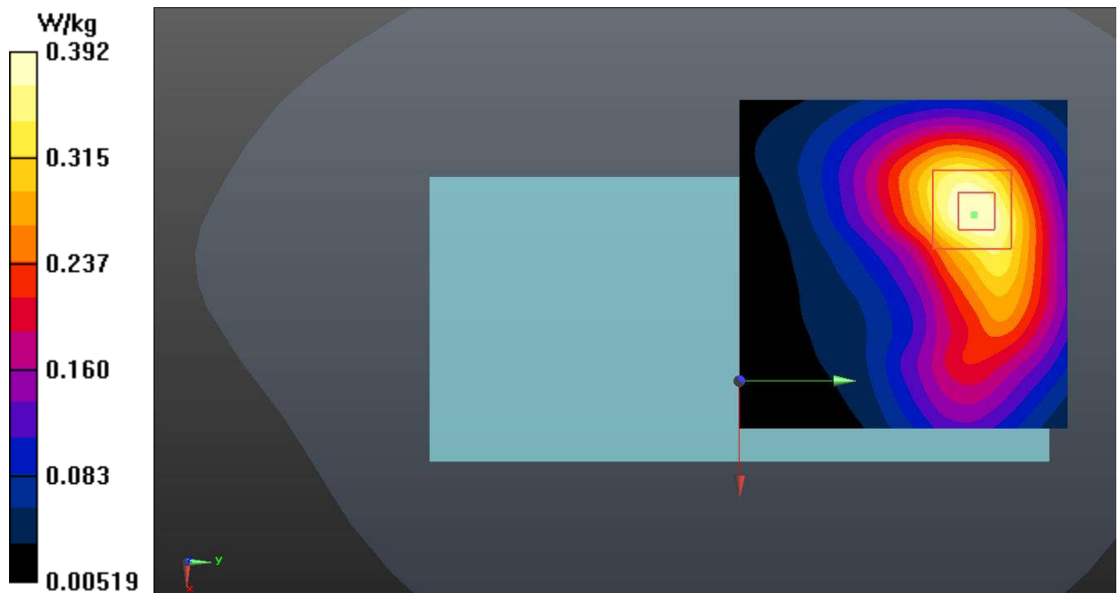
Fig.33 LTE Band 41
