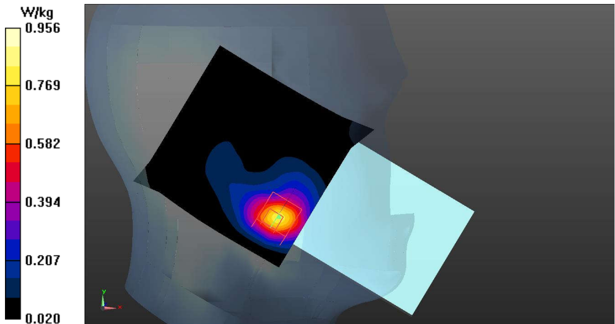
Fig.10 WCDMA Band 4
