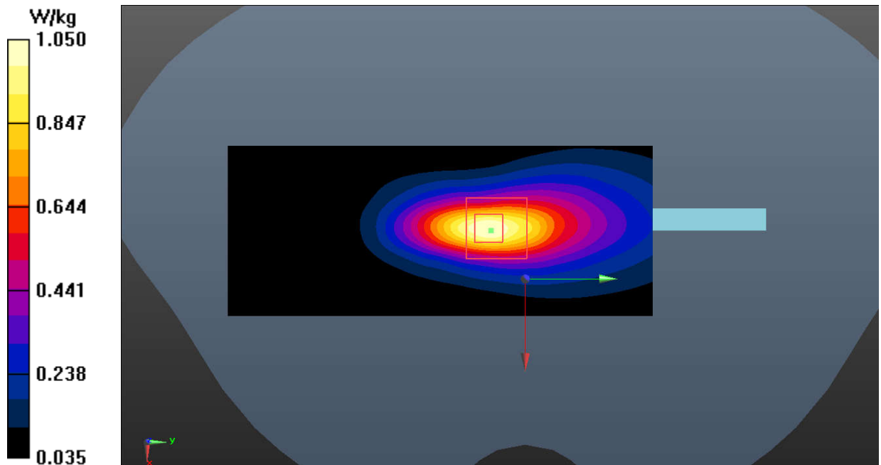
Fig.14 WCDMA Band 5
