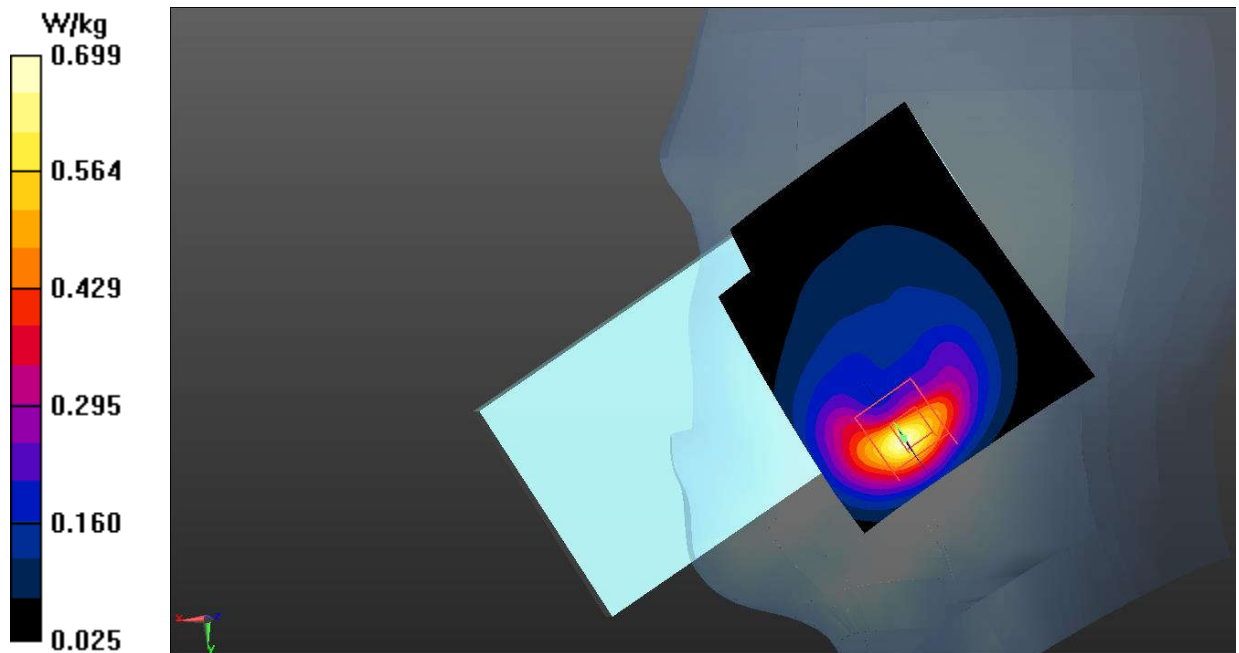
Fig.28 LTE Band 26
