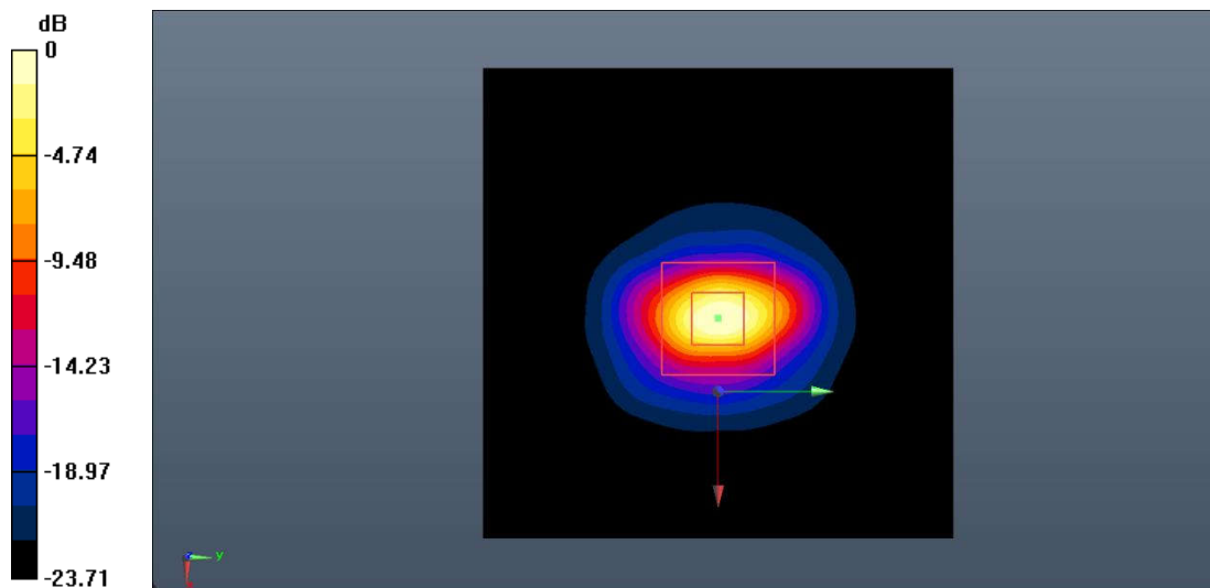
Fig.B.5. Validation 2550MHz 250mW
