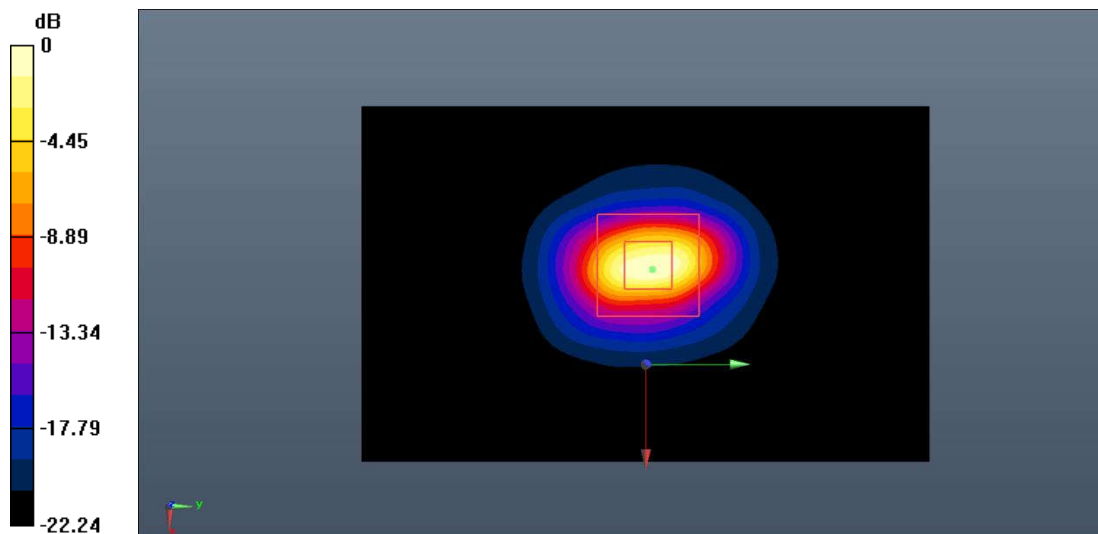
Fig.B.4. Validation 2450MHz 250mW
