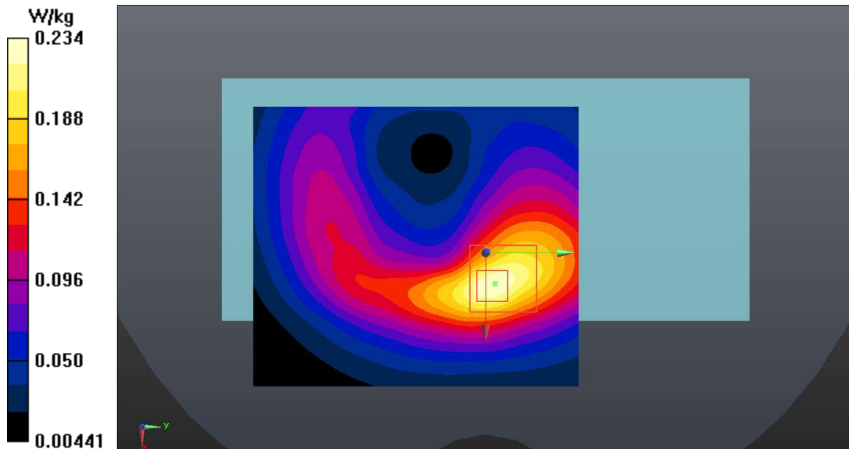
Fig.9 WCDMA Band 2
