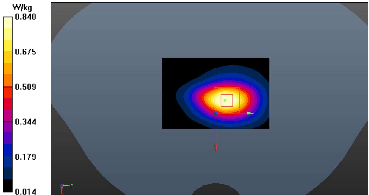
Fig.8 WCDMA Band 2
