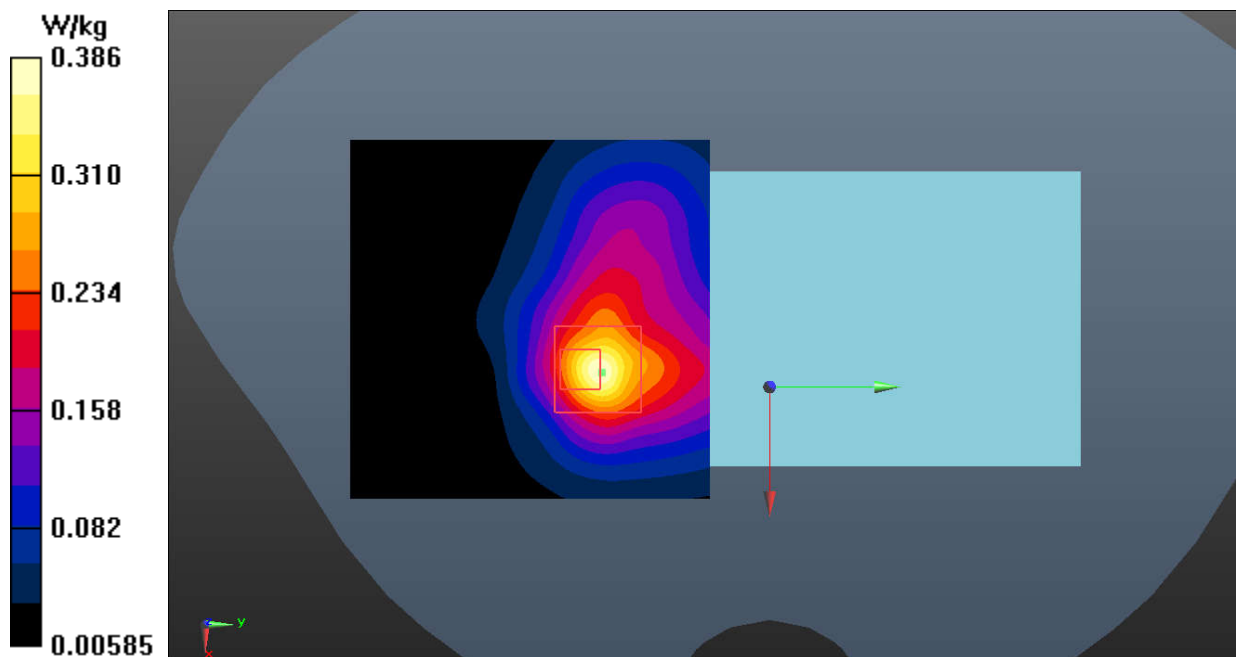
Fig.38 WLAN 2.4G
