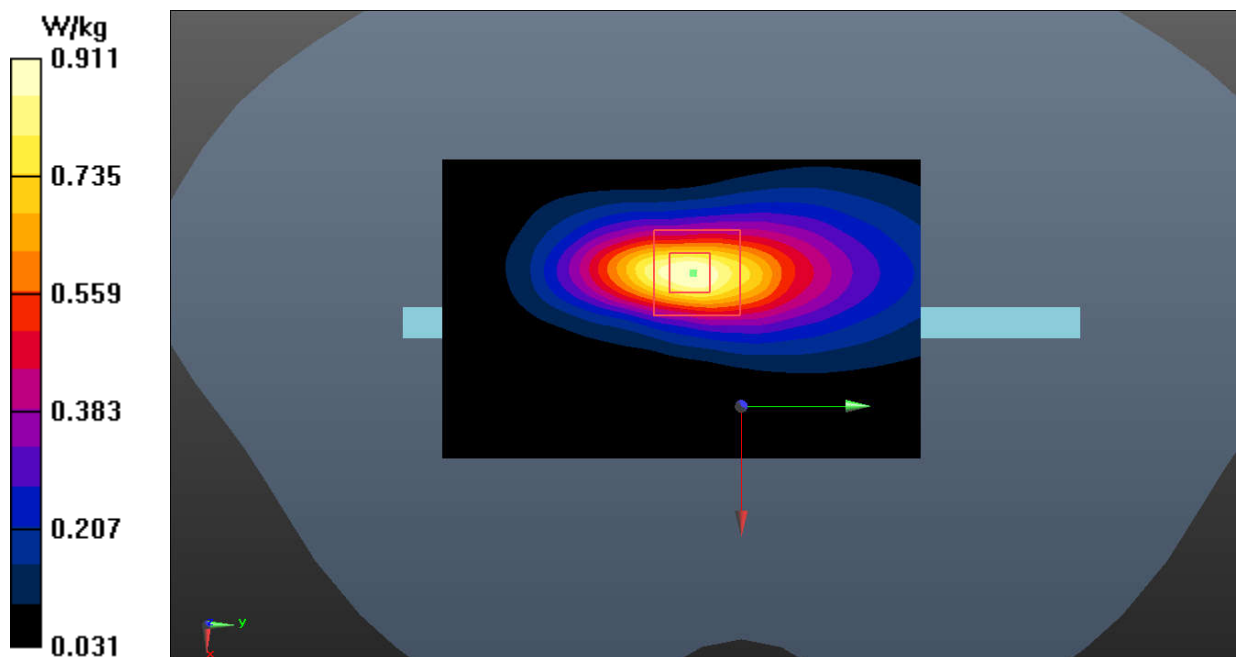
Fig.29 LTE Band 26
