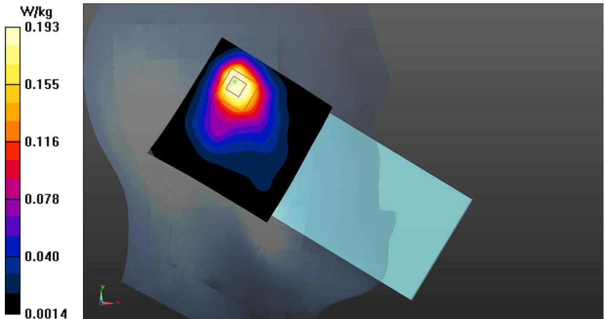
Fig.34 Bluetooth
