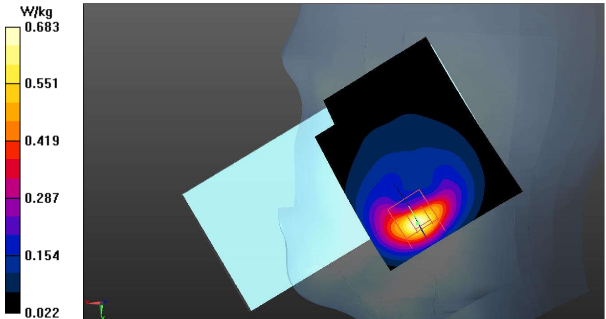
Fig.13 WCDMA Band 5
