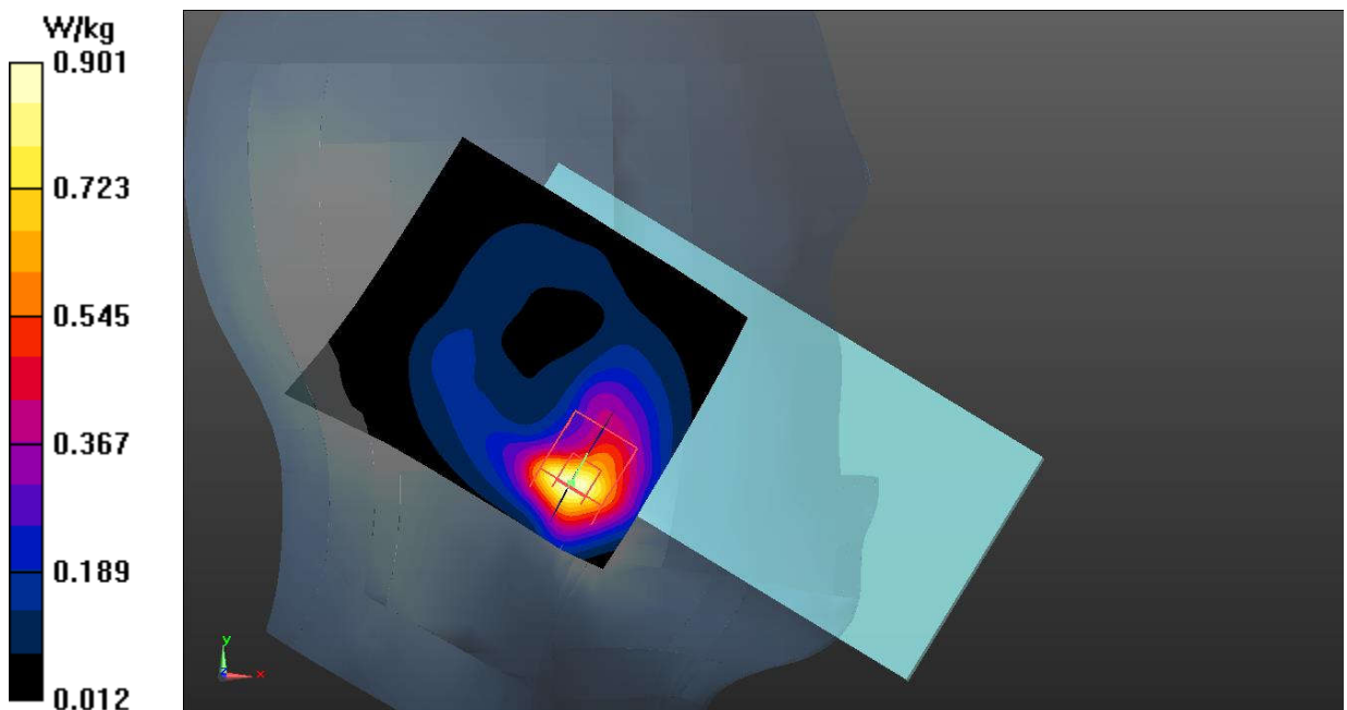
Fig.4 GSM 1900
