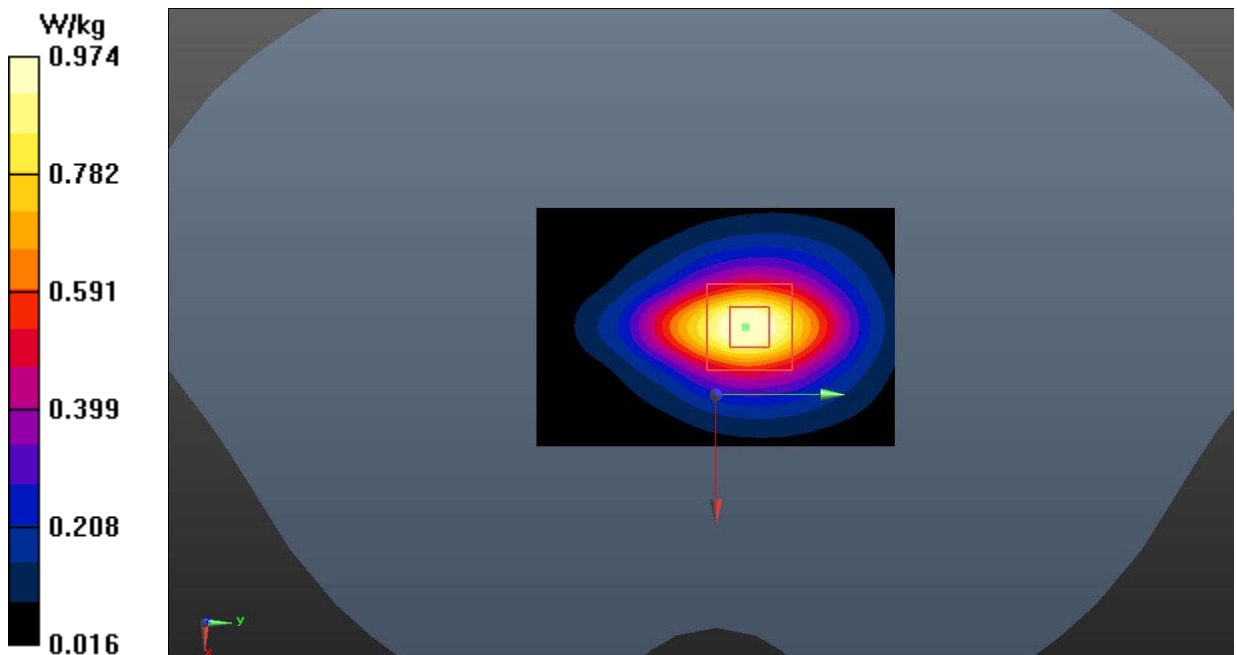
Fig.17 LTE Band 2
