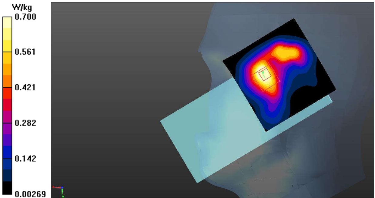
Fig.31 LTE Band 41
