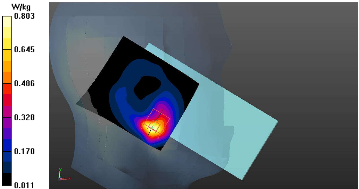
Fig.16 LTE Band 2
