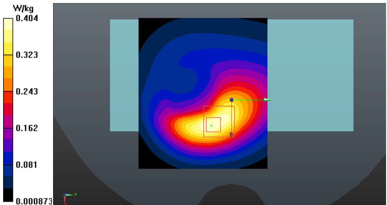
Fig.15 WCDMA Band 5
