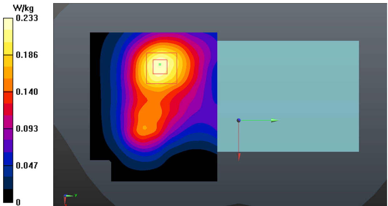
Fig.39 WLAN 2.4G
