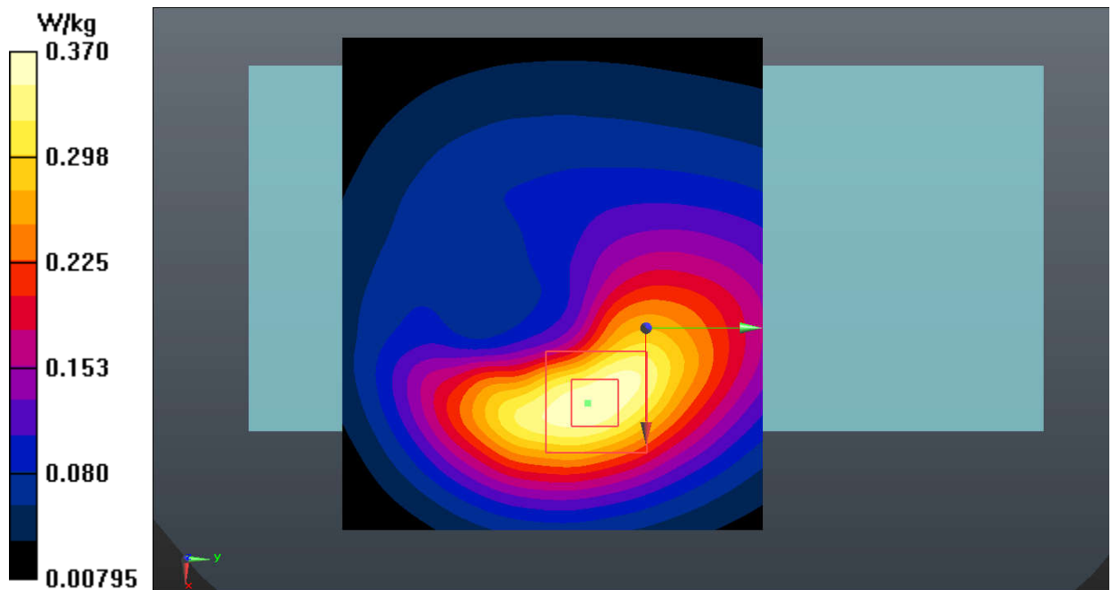
Fig.24 LTE Band 5
