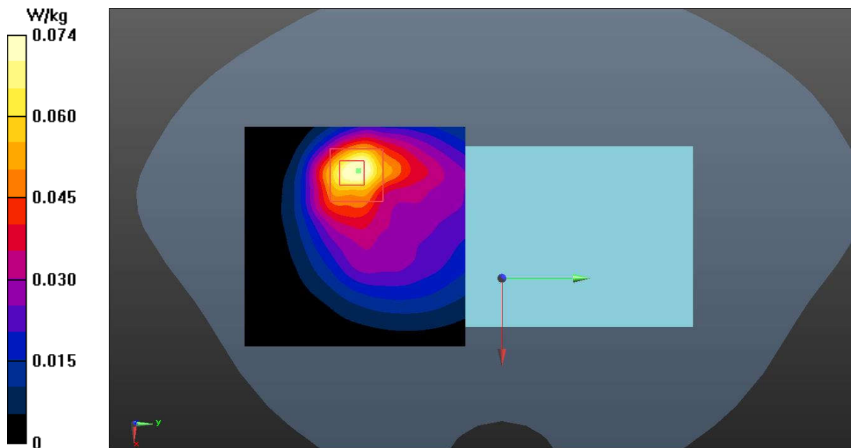
Fig.35 Bluetooth
