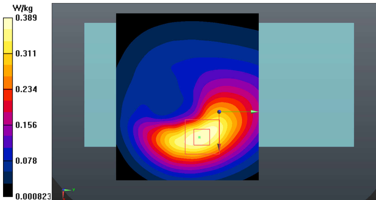
Fig.3 GSM 850
