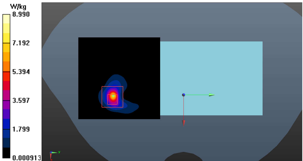
Fig.42 WLAN 5G
