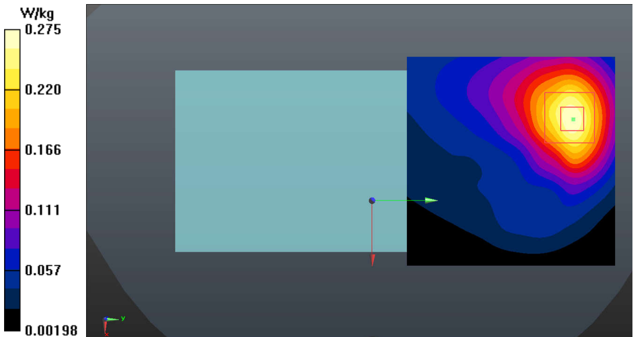
Fig.6 GSM 1900
