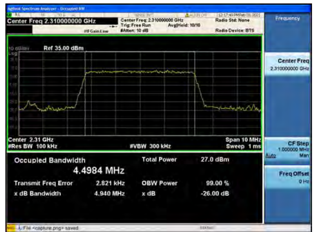
Band30 / 5MHz / Mid CH / 64QAM
