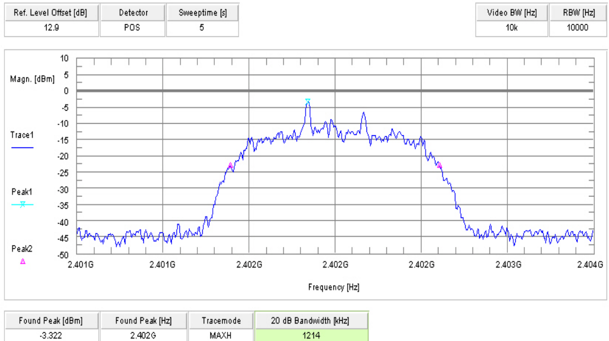
Plot 7 8DPSK
