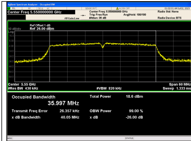
IEEE 802.11ac Channel 110 40MHz Antenna 0
