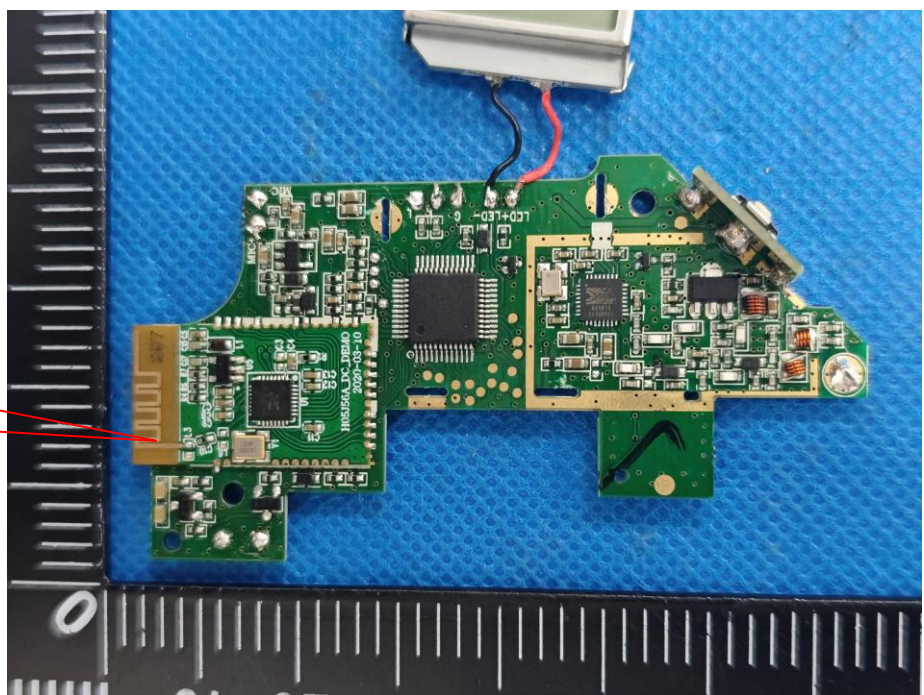
Bluetooth Antenna
