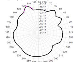
Total(H+V), Max=-11.15dBi, CrD=15.38
