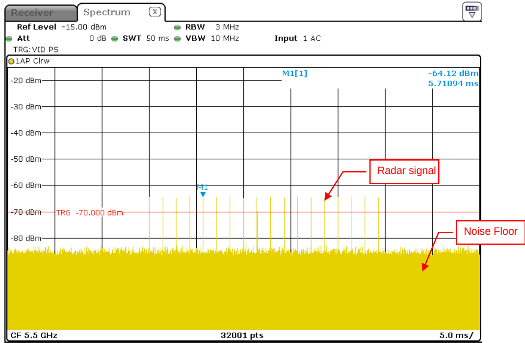
Radar Signal 0
