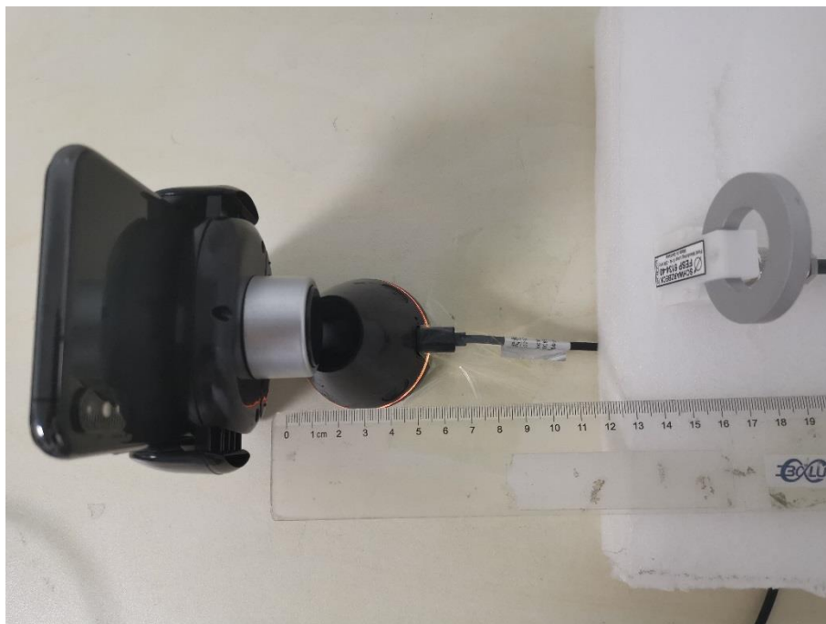
H-field Test Setup Photo Positon F (15cm)
