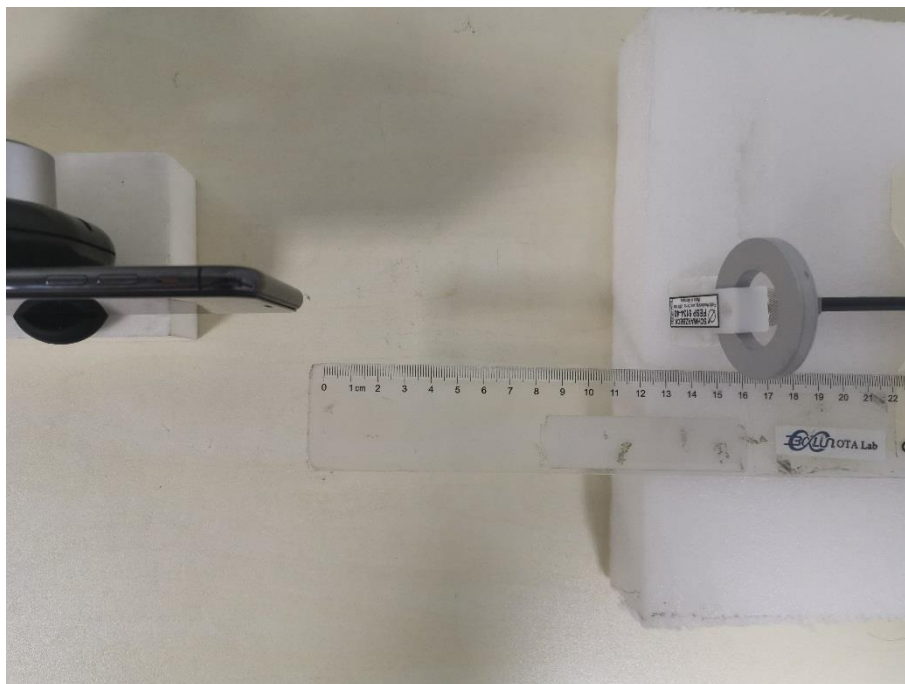
H-field Test Setup Photo Positon B (15cm)
