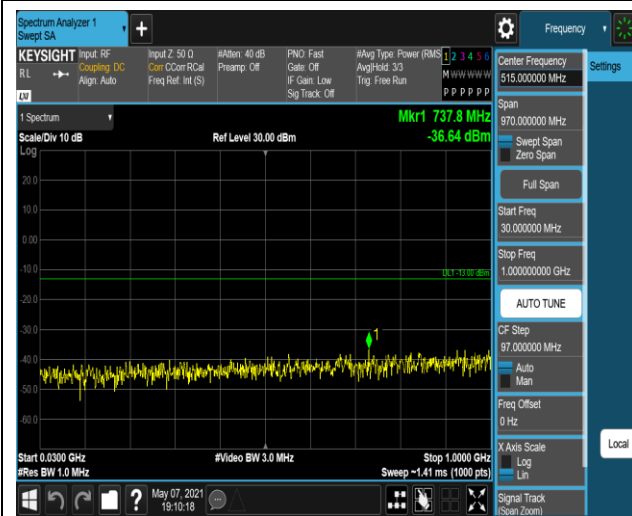
Band4-1.4MHz-16QAM-20175:30~1000MHz
