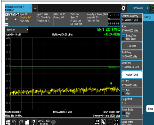
Band2-20MHz-QPSK-18900:30~1000MHz
