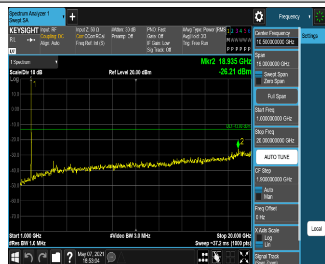
Band2-20MHz-16QAM-19100:1000~20000MHz
