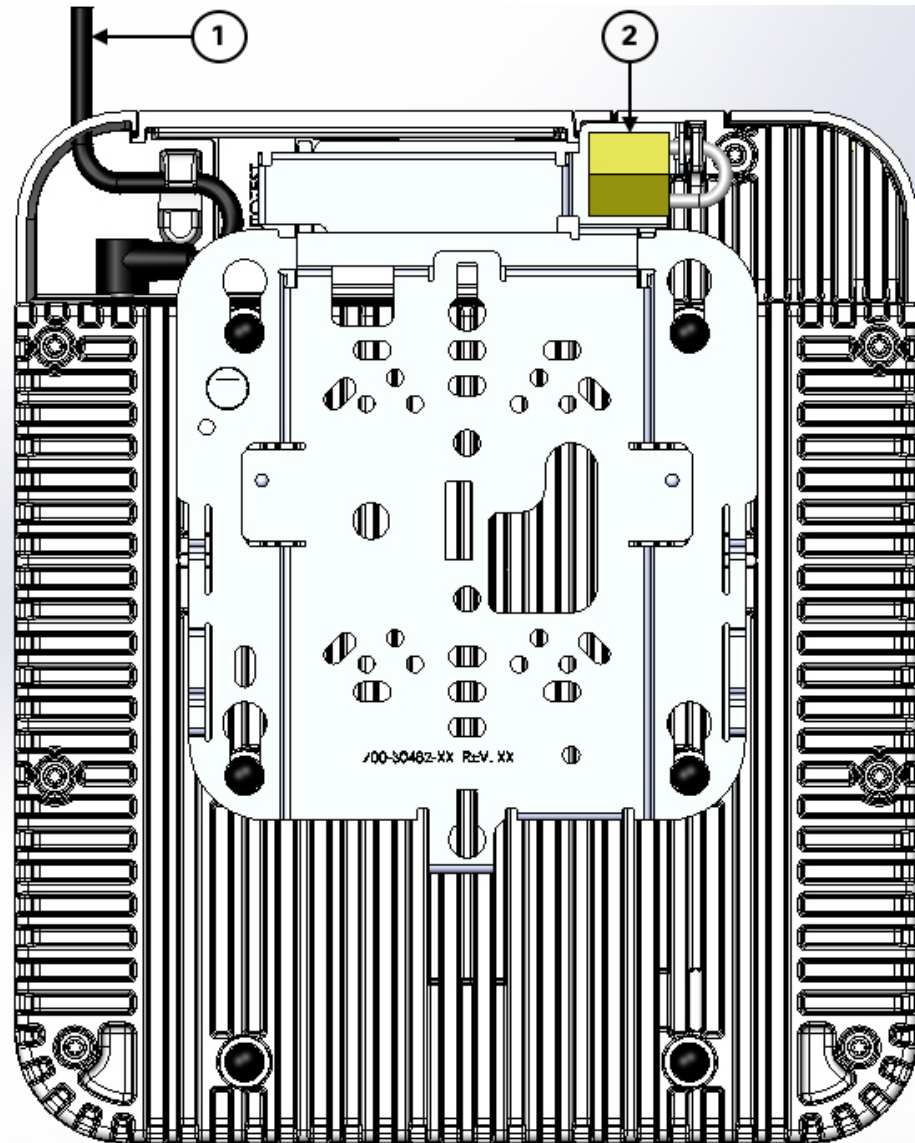
Figure 4 Locking the AP to the Bracket and Power Cable Routing
