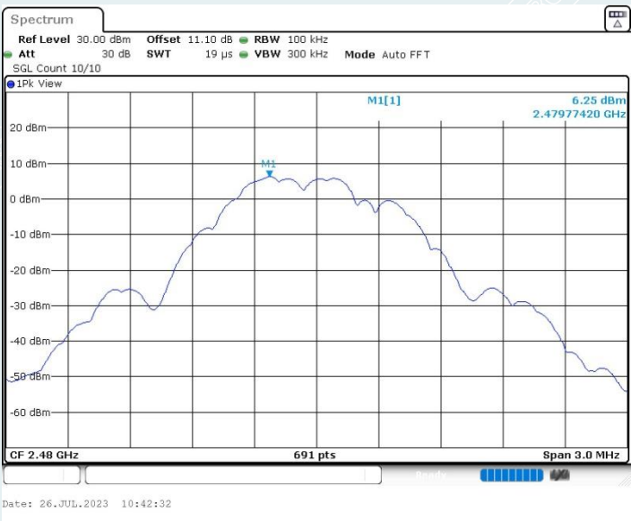
BLE_1M_Ant1_2480MHz_0~Reference
