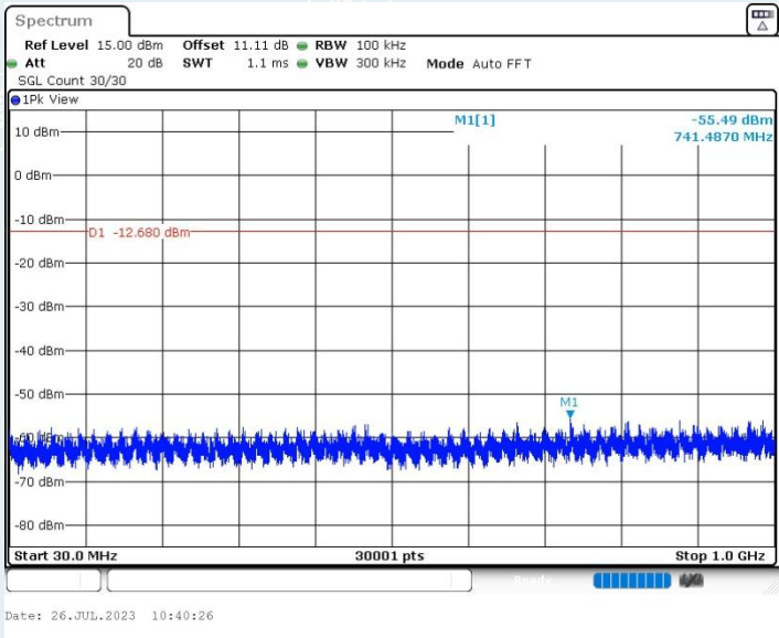
BLE_1M_Ant1_2440MHz_30~1000MHz
