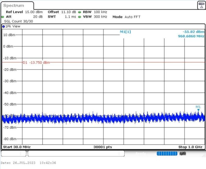
BLE_1M_Ant1_2480MHz_30~1000MHz
