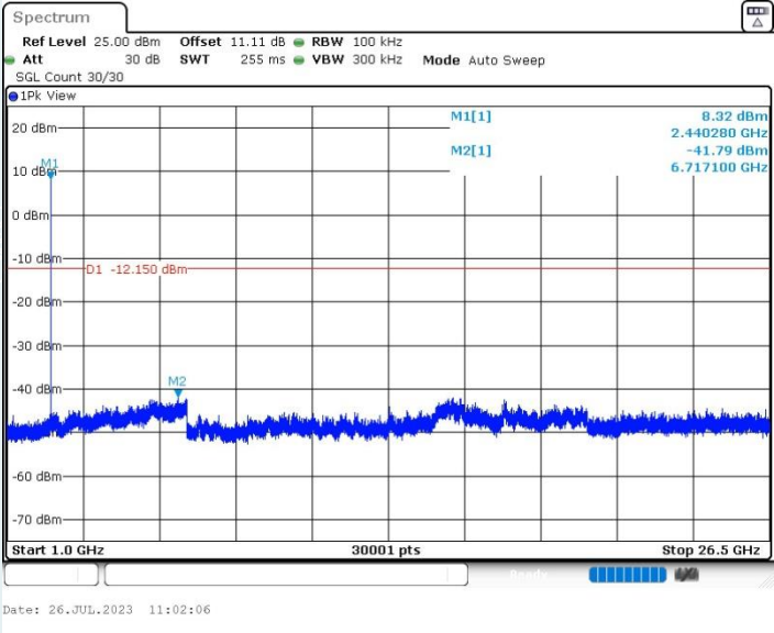
BLE_2M_Ant1_2440MHz_1000~26500MHz
