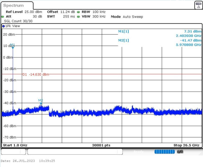
BLE_1M_Ant1_2402MHz_1000~26500MHz
