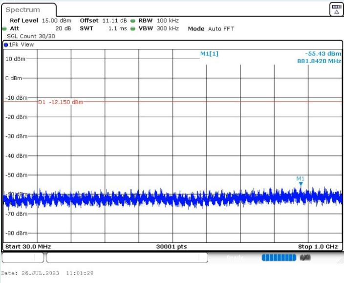
BLE_2M_Ant1_2440MHz_30~1000MHz
