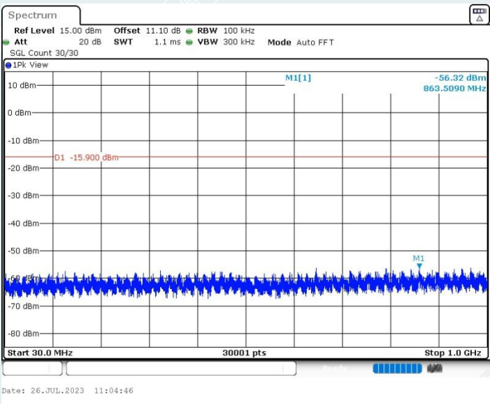
BLE_2M_Ant1_2480MHz_30~1000MHz
