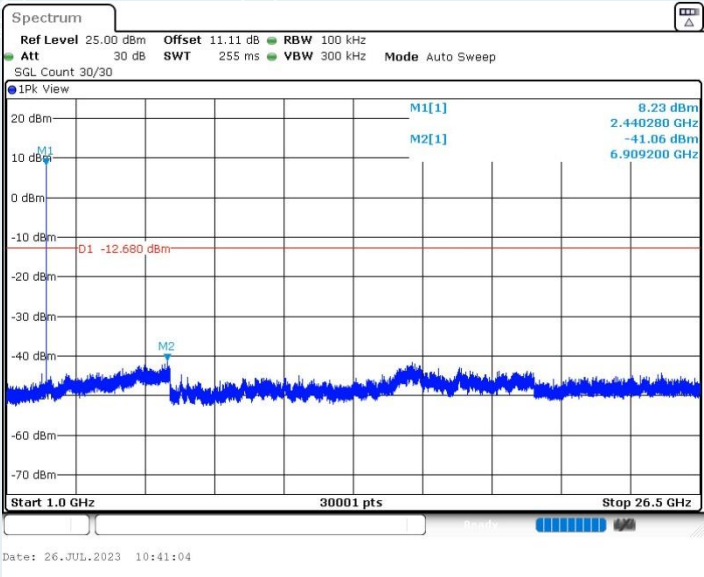
BLE_1M_Ant1_2440MHz_1000~26500MHz
