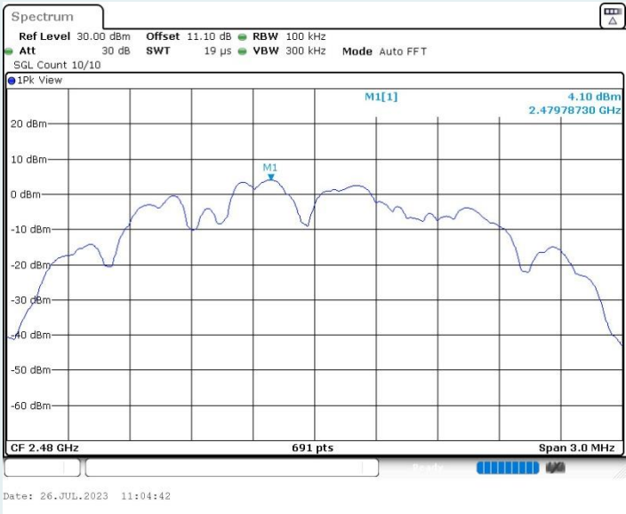
BLE_2M_Ant1_2480MHz_0~Reference
