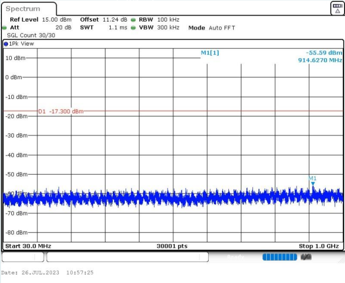
BLE_2M_Ant1_2402MHz_30~1000MHz
