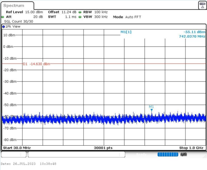
BLE_1M_Ant1_2402MHz_30~1000MHz
