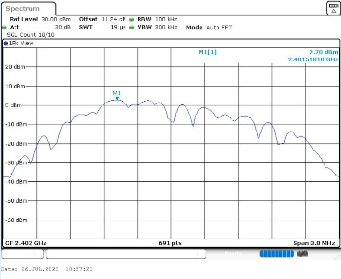
BLE_2M_Ant1_2402MHz_0~Reference
