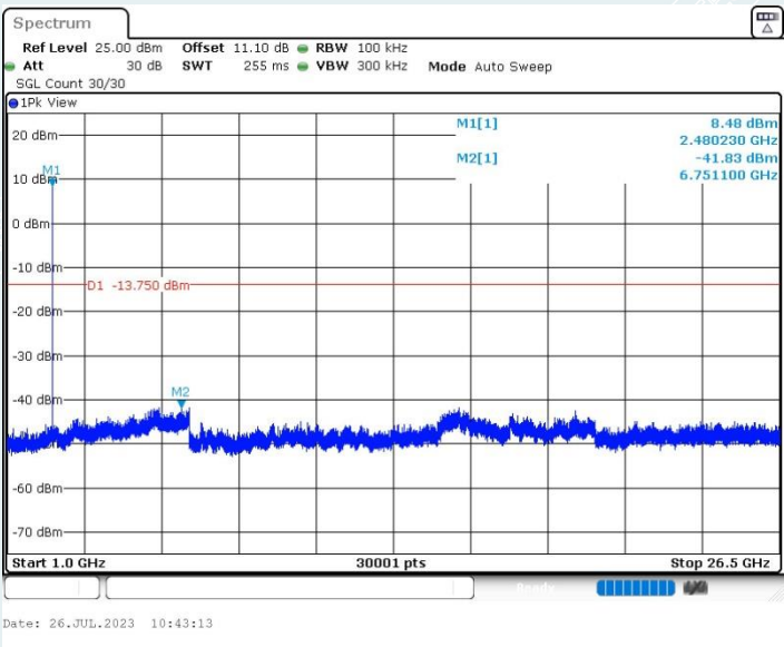
BLE_1M_Ant1_2480MHz_1000~26500MHz
