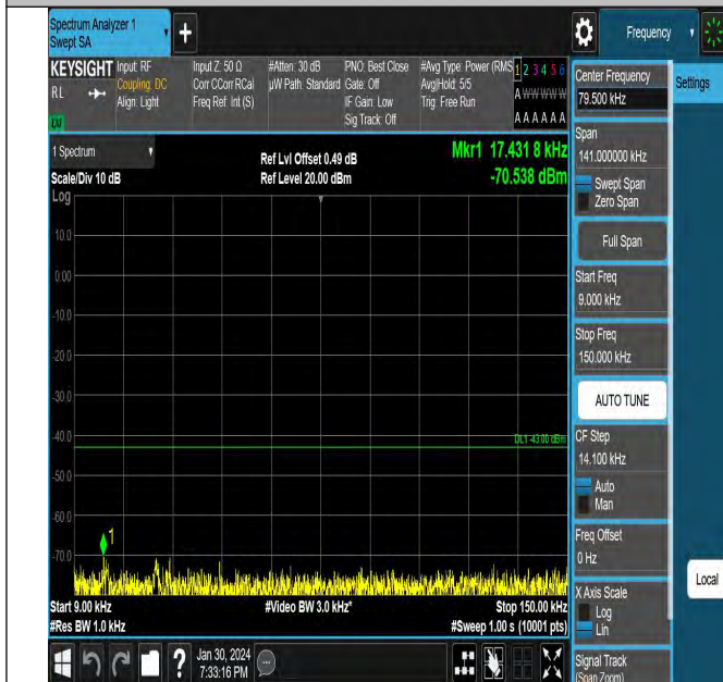
EGPRS1900-512-2-0.009~0.15MHz-PASS
