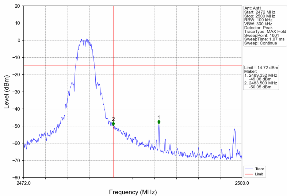
2.4GHz wireless_HCH_2480MHz_Ant1_NTNV
