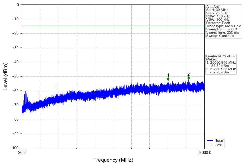
2.4GHz wireless_MCH_2440MHz_Ant1_NTNV
