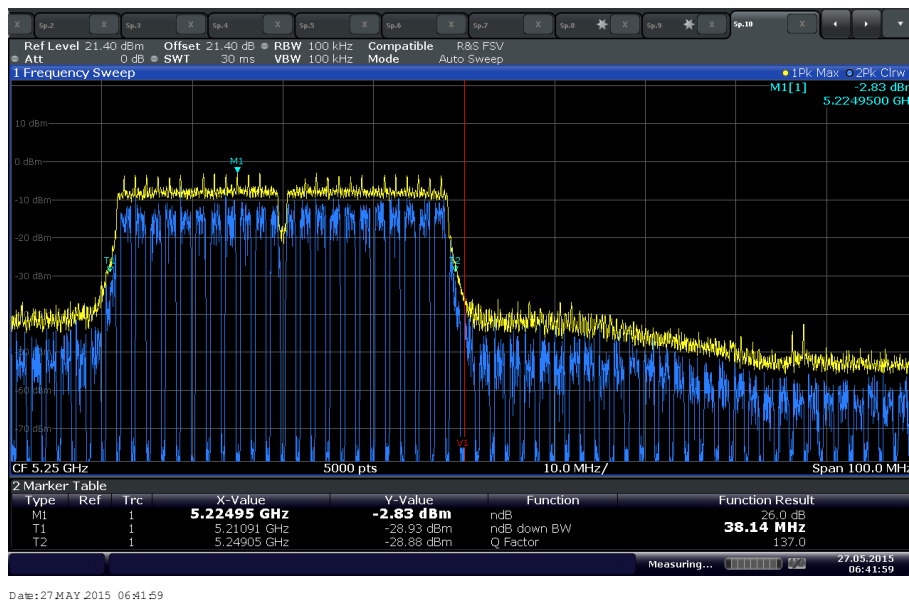
U-NII 1 Worst Case Channel @ 20°C and extreme voltage (102VAC)
