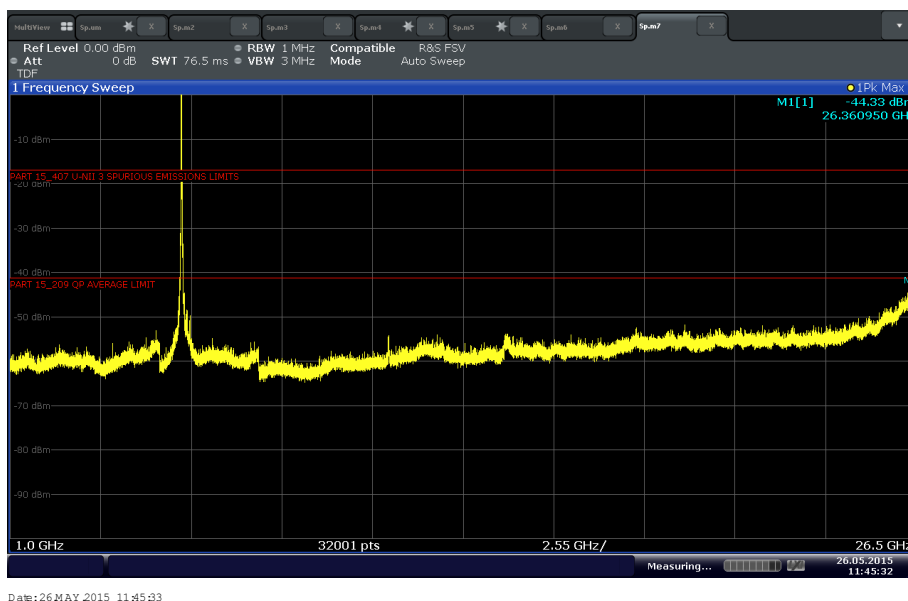
U-NII 3 High Channel above 1GHz (20 MHz BW)
