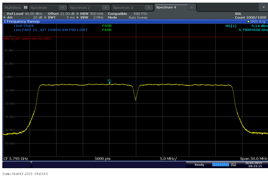
802.11n U-NII 3 40MHz BW Channel 159 (5795 MHz)
