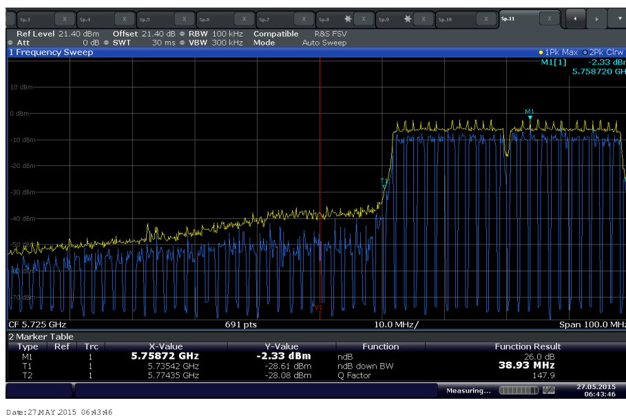
U-NII 3 Worst Case Channel @ 20°C and extreme voltage (138VAC)
