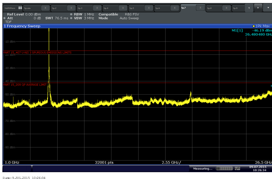
U-NII 2A High Channel above 1GHz (40 MHz BW)
