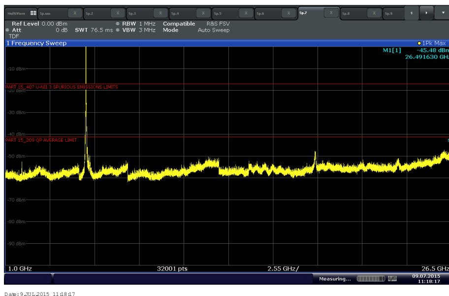
U-NII 2C Mid Channel above 1GHz (20 MHz BW)
