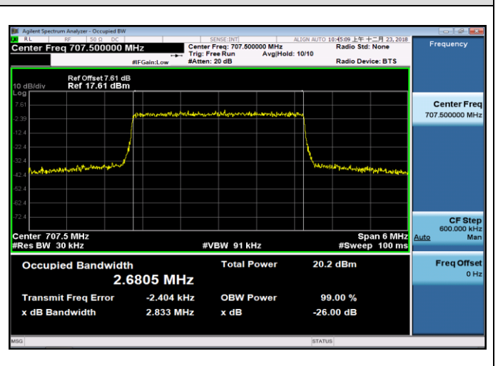
MCH_16QAM_15RB#0
