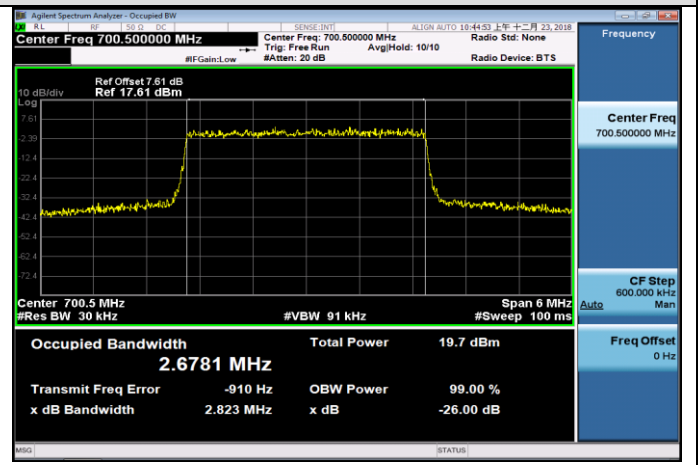
LCH_16QAM_15RB#0
