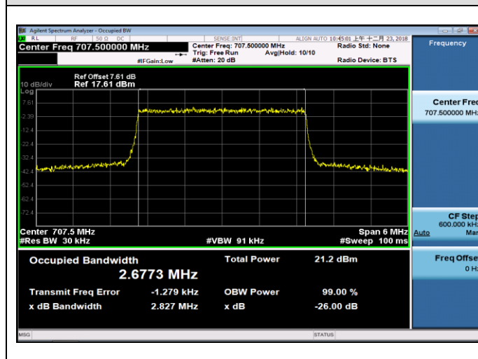
MCH_QPSK_15RB#0
