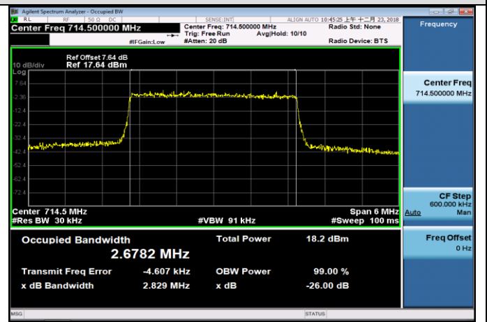
HCH_16QAM_15RB#0
