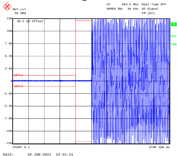
463.5_Turn Off
