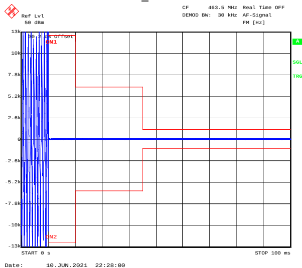
463.5_Turn On
